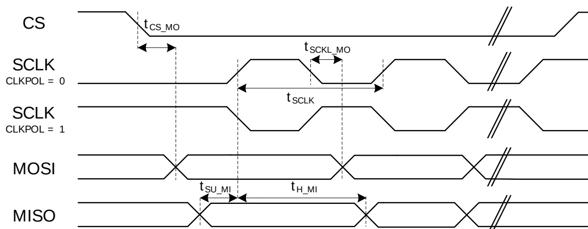
Figure 3.38. SPI Master Timing
