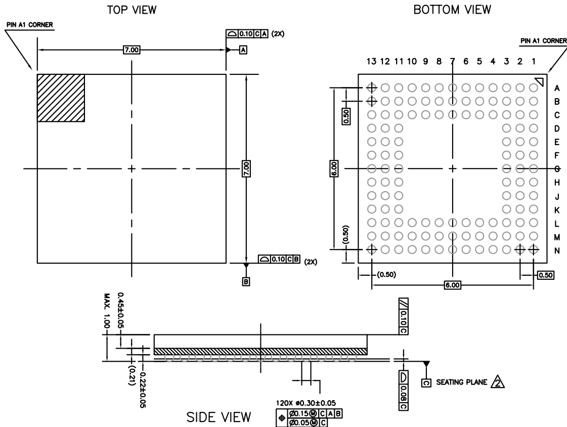
Figure 4.3. BGA120
