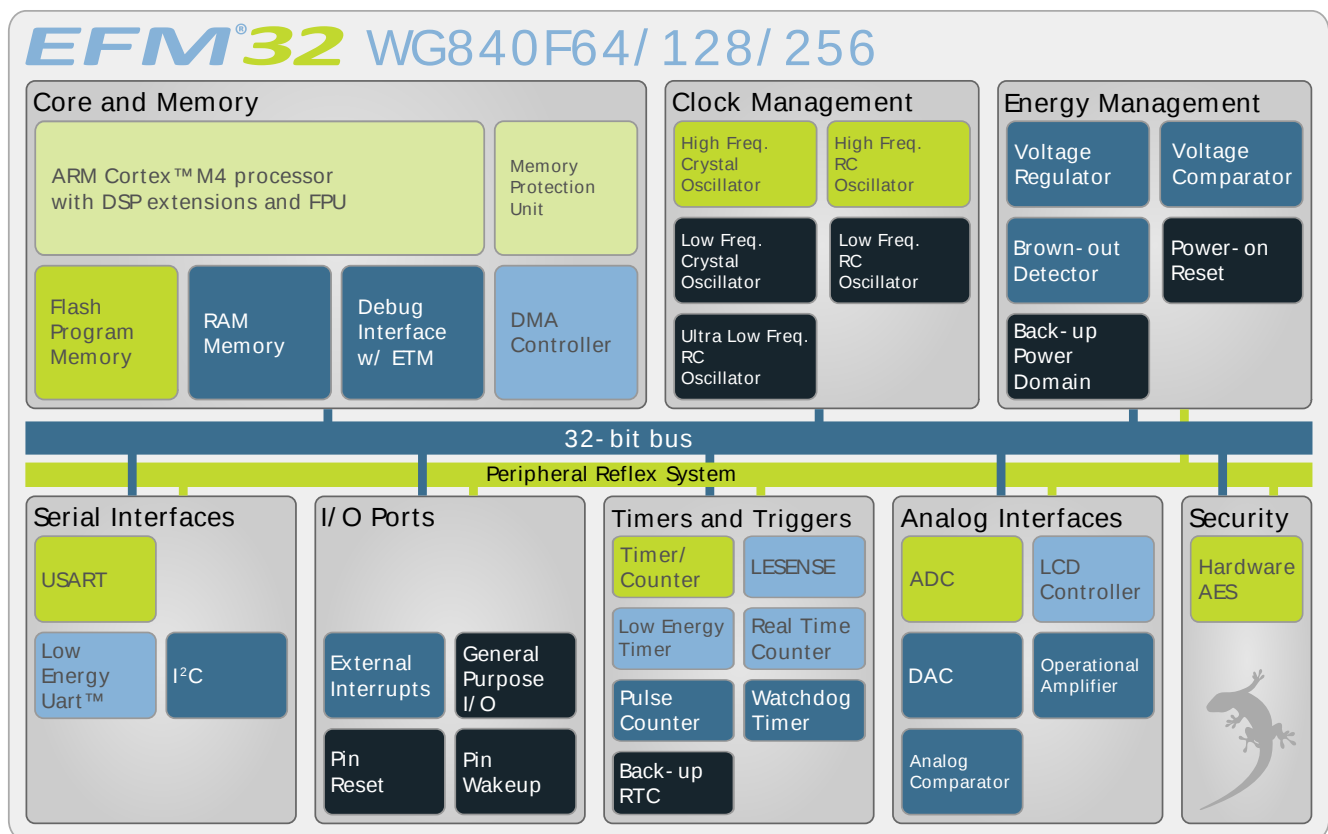
Figure 2.1. Block Diagram
