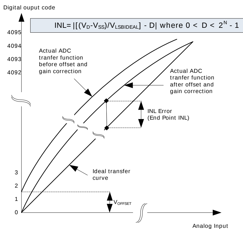
Figure 3.24. Integral Non-Linearity (INL)
