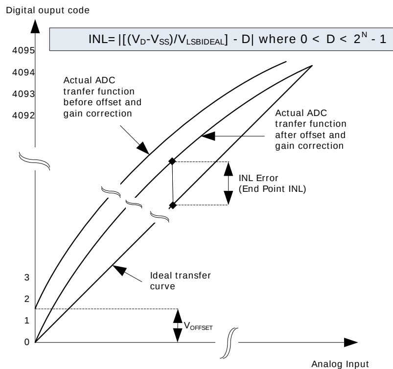
Figure 3.24. Integral Non-Linearity (INL)
