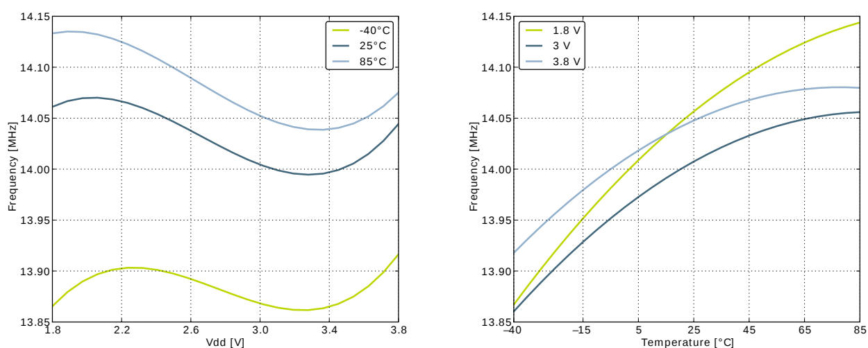
Figure 3.22. Calibrated HFRCO 21 MHz Band Frequency vs Supply Voltage and Temperature
