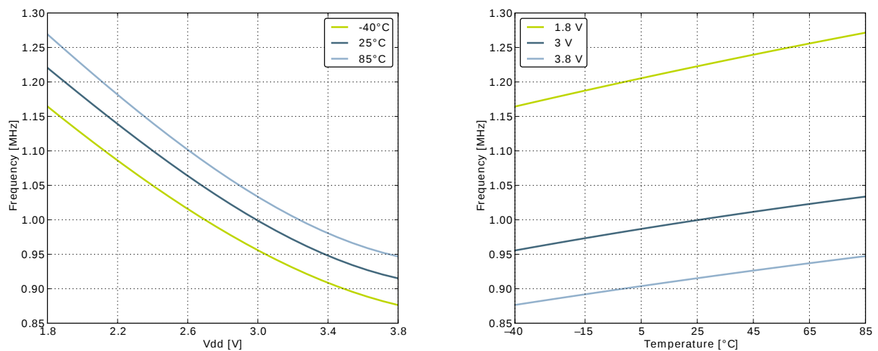
Figure 3.19. Calibrated HFRCO 7 MHz Band Frequency vs Supply Voltage and Temperature
