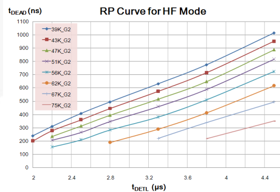
Figure 6. t_{\text{DEAD}} vs. t_{\text{DETL}} RP Curve for HF Mode
