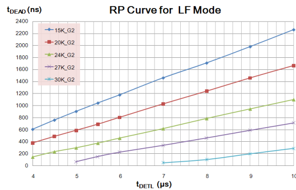
Figure 5. t_{\text{DEAD}} vs. t_{\text{DETL}} RP Curve for LF Mode
