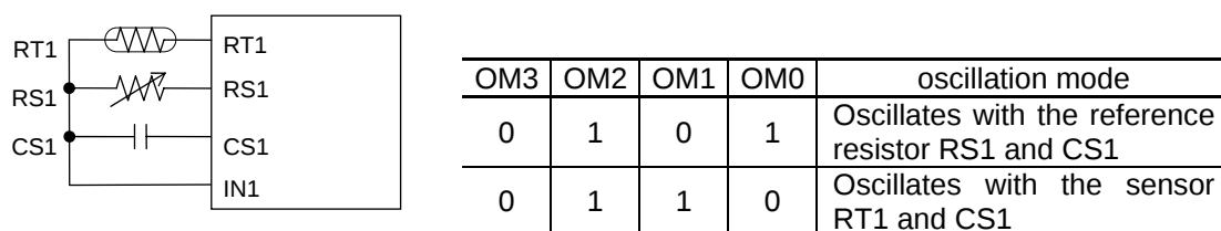
Figure 21-5 When RCOSC1 Is Used for Measurement with One Resistive Sensor
