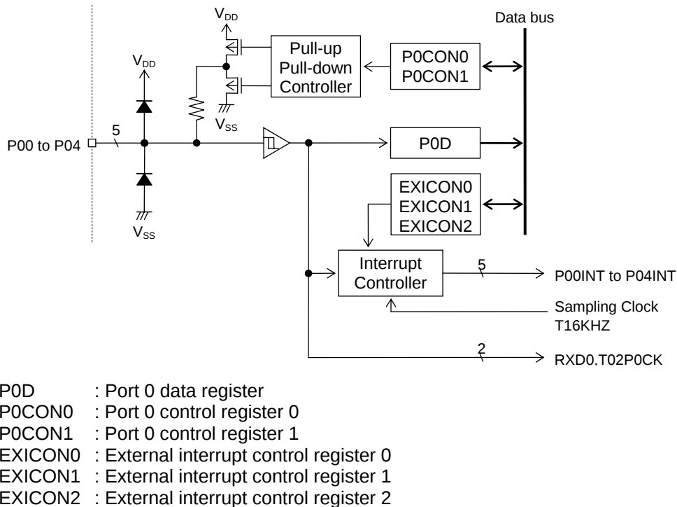
Figure 14-1 Configuration of Port 0
