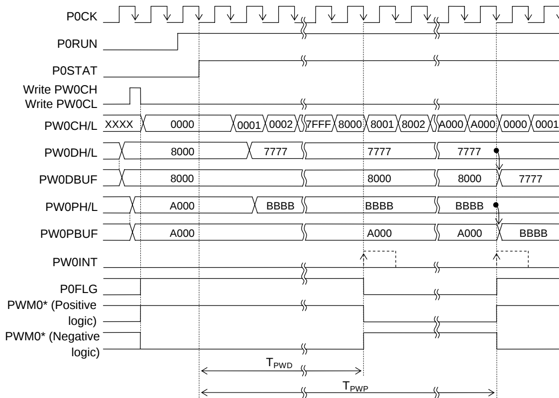
Figure 10-2 (1/2) Operation Timing Diagram of PWM0
