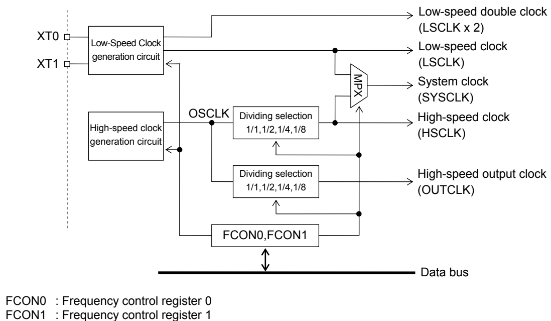
Figure 6-1 Configuration of Clock Generation Circuit
