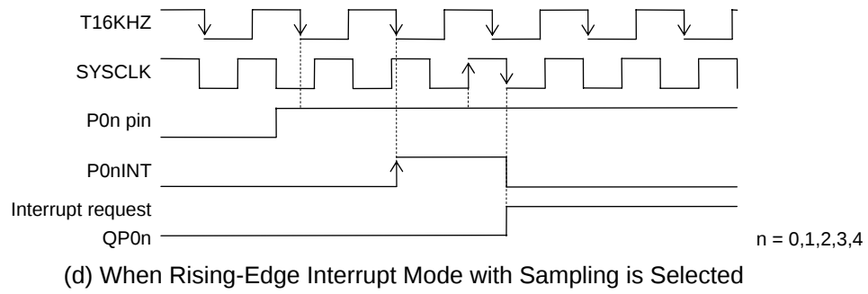
Figure 14-2 P00 to P04 Interrupts Generation Timing
