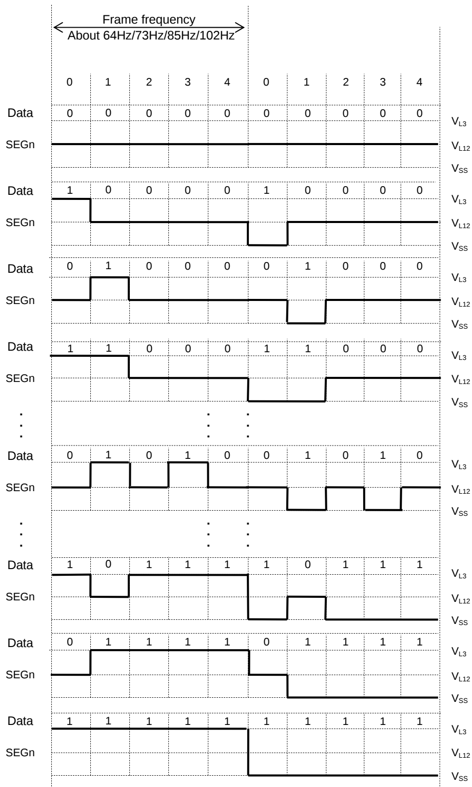
Figure 22-12 Segment Output Waveform at 1/5 Duty (5 Commons) and 1/2 Bias (ML610Q407/ML610Q408/ML610Q409)
