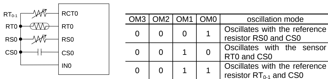
Figure 21-3 When RCOSC0 Is Used for Measurement with One Resistive Sensor (Two points are adjusted with two reference resistors)
