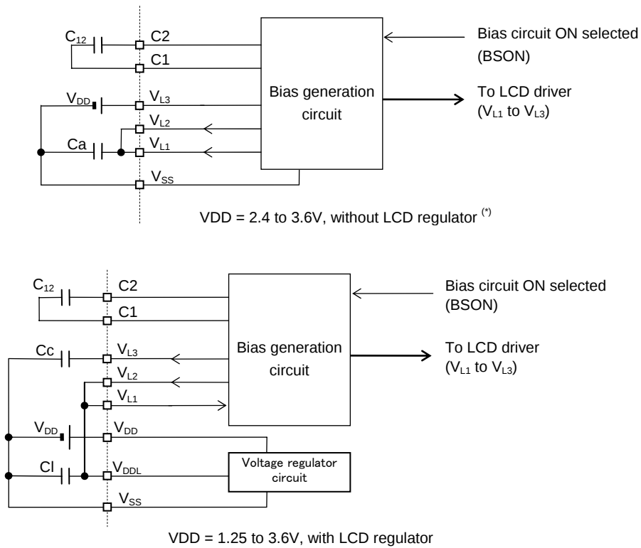
Figure 22-5-2 Configuration of Bias Generation Circuit (1/2 Bias)
