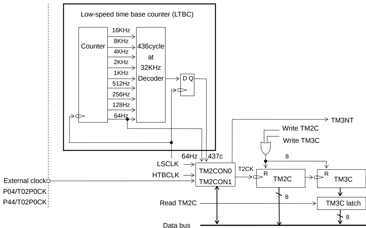
(c) Frequency measurement mode with 16 bit timer(Timer2 to 3)
