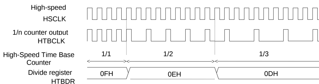
Figure 7-5 Output Waveform of HTBCLK
