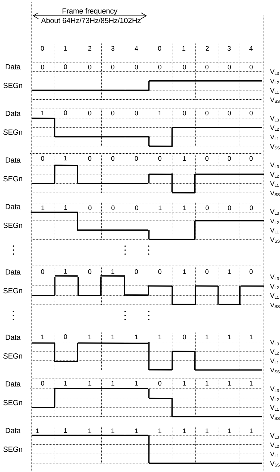
Figure 22-11 Segment Output Waveform at 1/5 Duty (5 Commons) and 1/3 Bias
