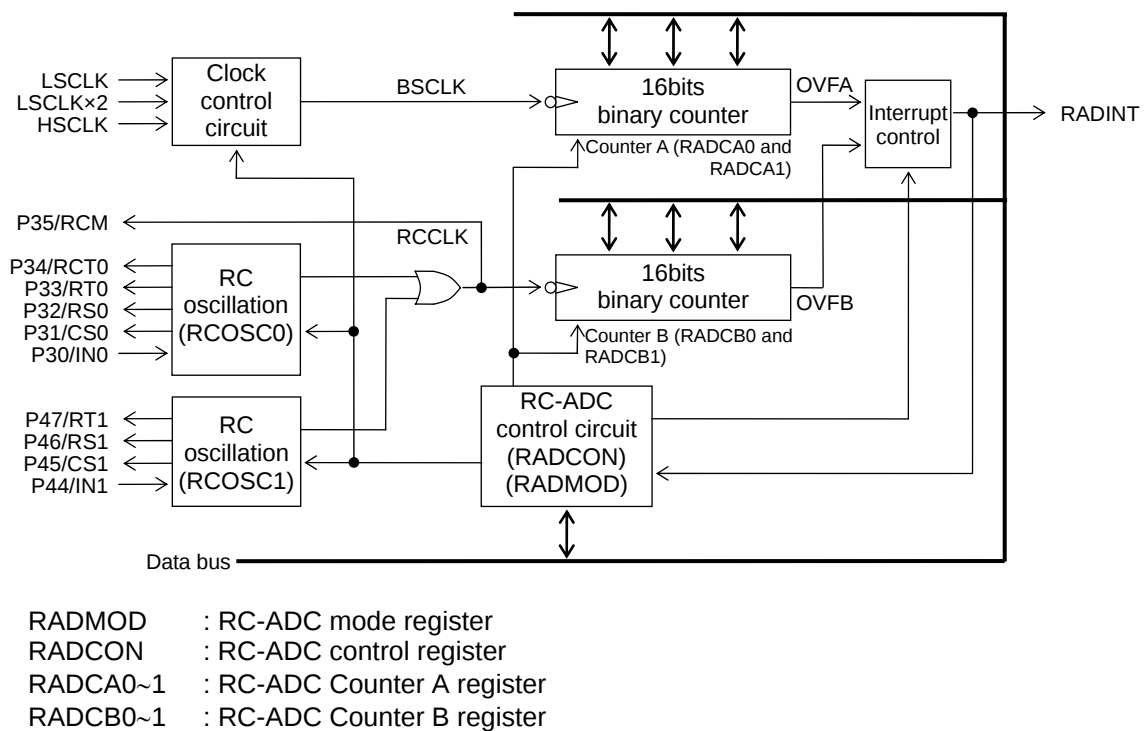
Figure 21-1 Configuration of RC-ADC
