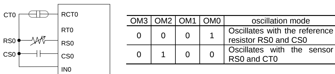
Figure 21-4 When RCOSC0 Is Used for Measurement with One Capacitive Sensor
