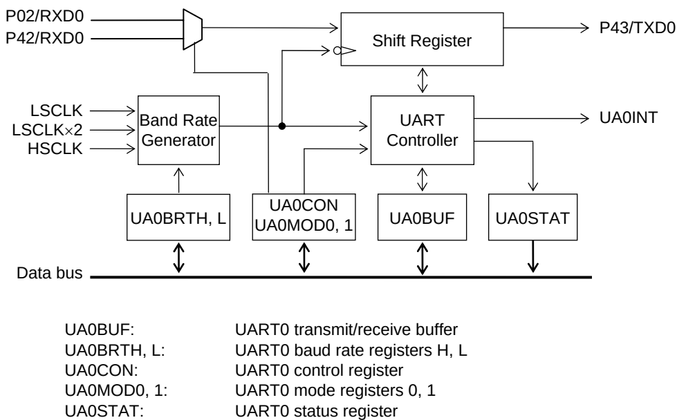
Figure 12-1 Configuration of UART
