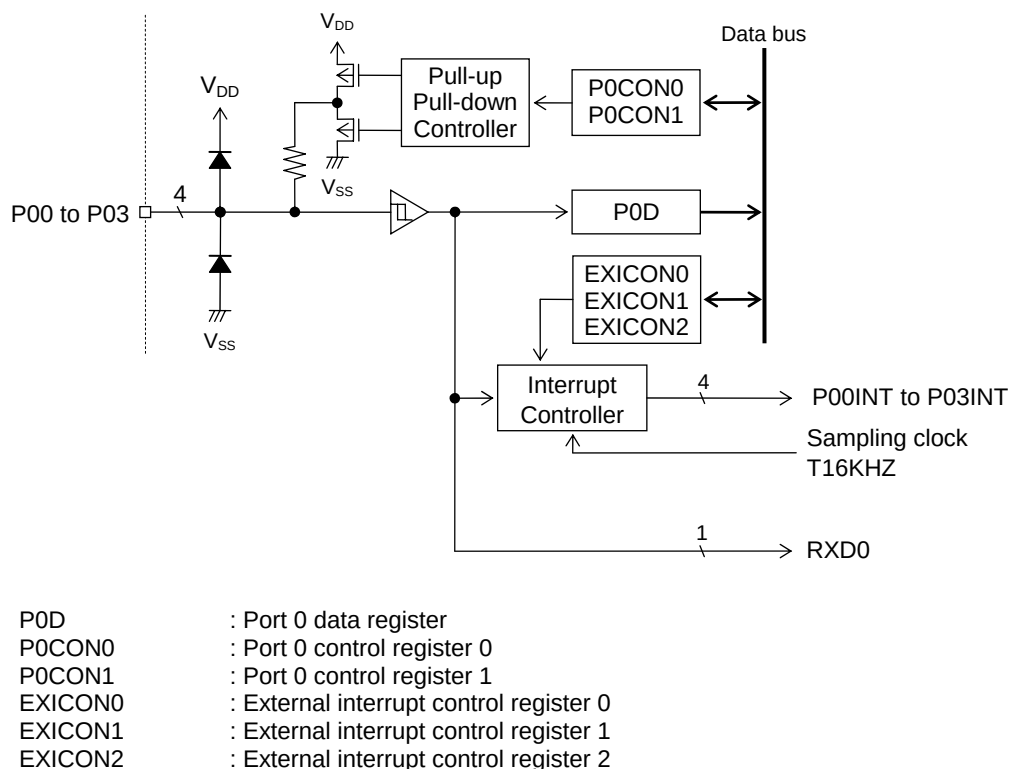
Figure 15-1 Configuration of Port 0
