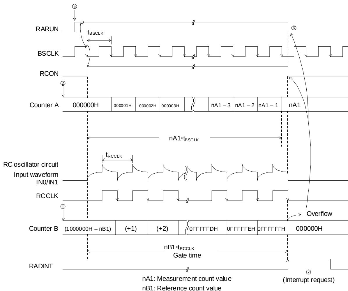
Figure 22-7 Operation Timing in Counter B Reference Mode
