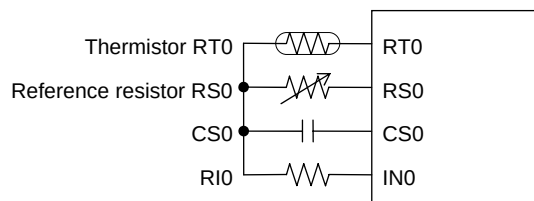
Figure 22-8 Configuration of 1-Thermistor RC Oscillator Circuit Using RCOSC0
