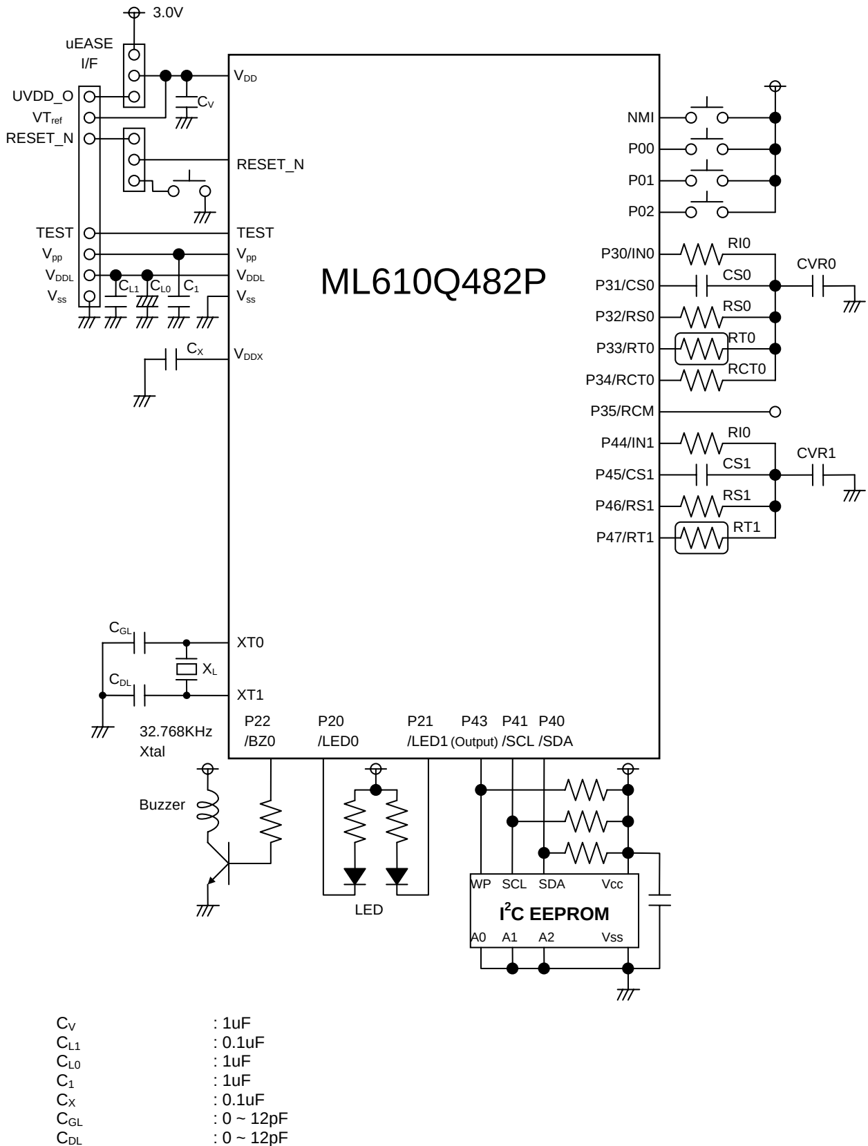
Figure D-1 Application Circuit Example of ML610Q482P
