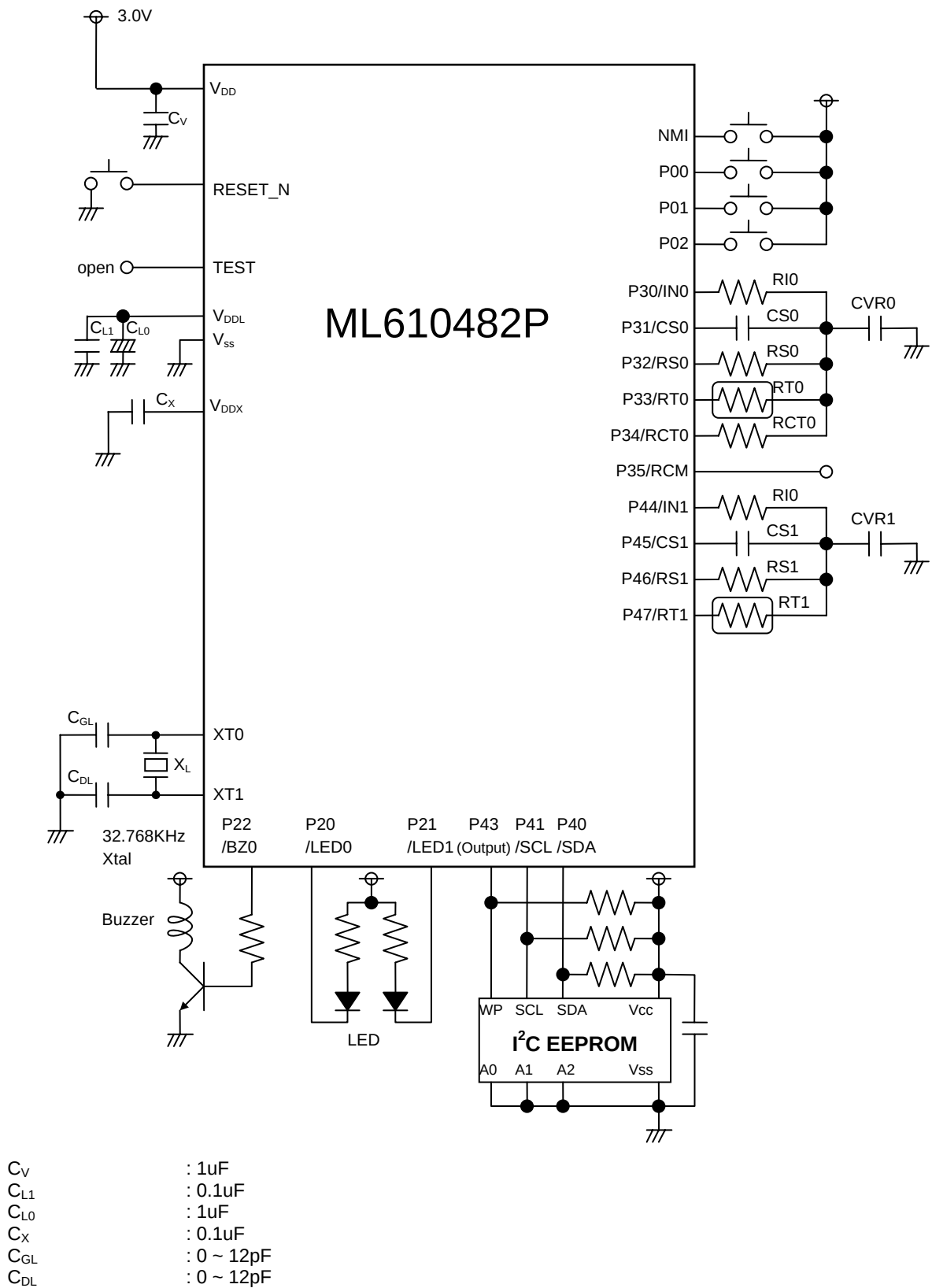
Figure D-2 Application Circuit Example of ML610482P
