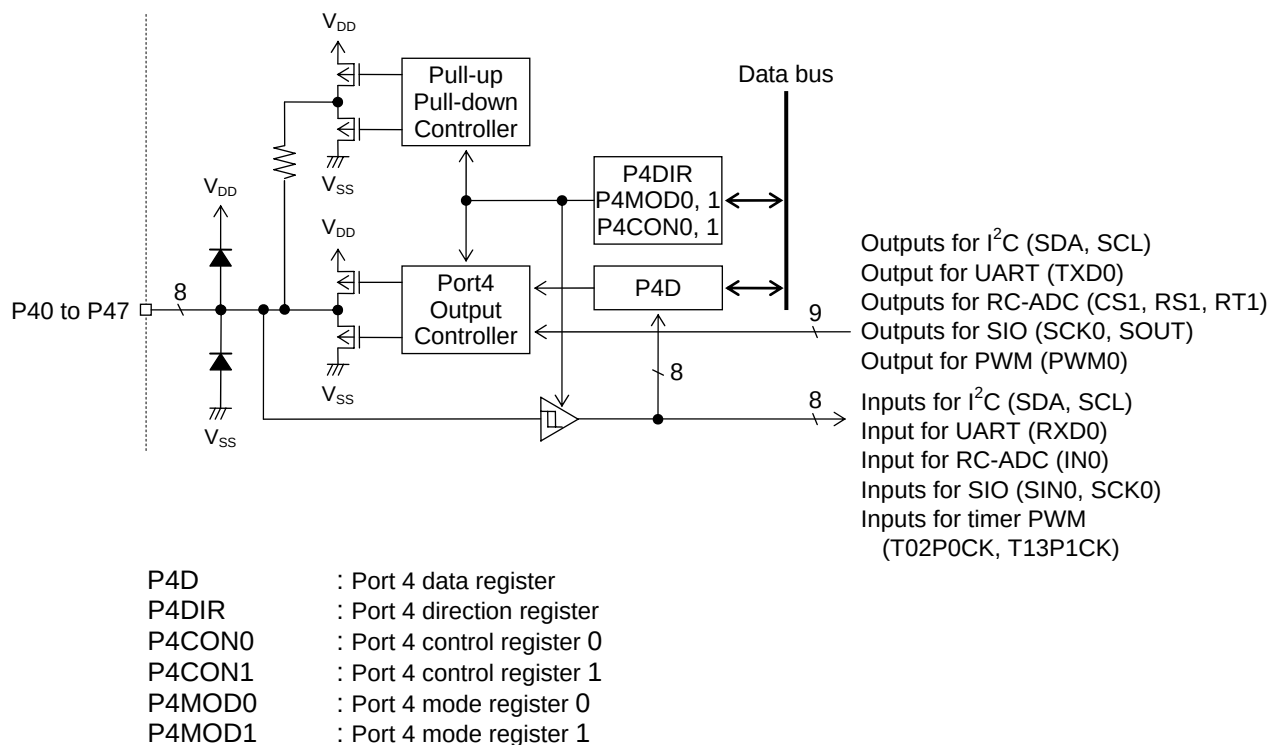
Figure 19-1 Configuration of Port 4
