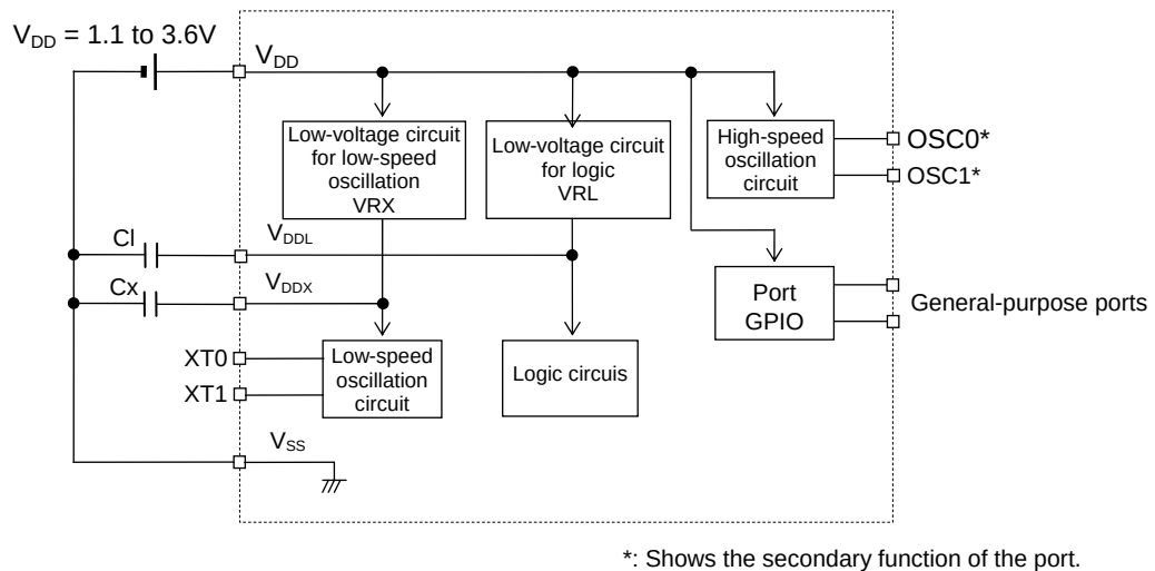
Figure 25-1 Configuration of Power Supply Circuit
