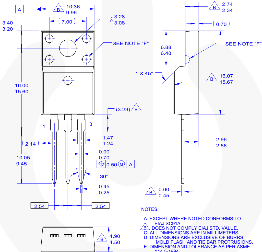
Figure 9. TO220, MOLDED, 3-LEAD, FULL PACK, EIAJ SC91, STRAIGHT LEAD (ACTIVE)
