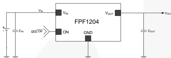
Figure 22. Typical Application
