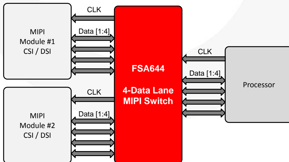
Figure 1. Mobile Phone Example
