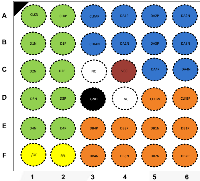
Figure 3. Top Through View
