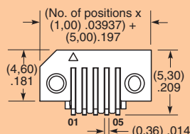
-03, -06 & -10 Contact Detail
