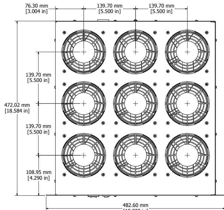
ASSEMBLY - VIEW FROM TOP
