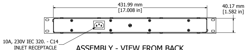
ASSEMBLY - VIEW FROM BACK
