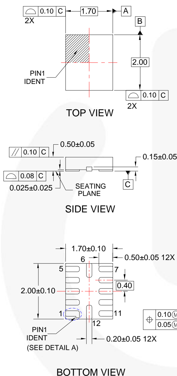
Figure 11. 12-Lead, Ultrathin Molded Leadless Package (UMLP)
