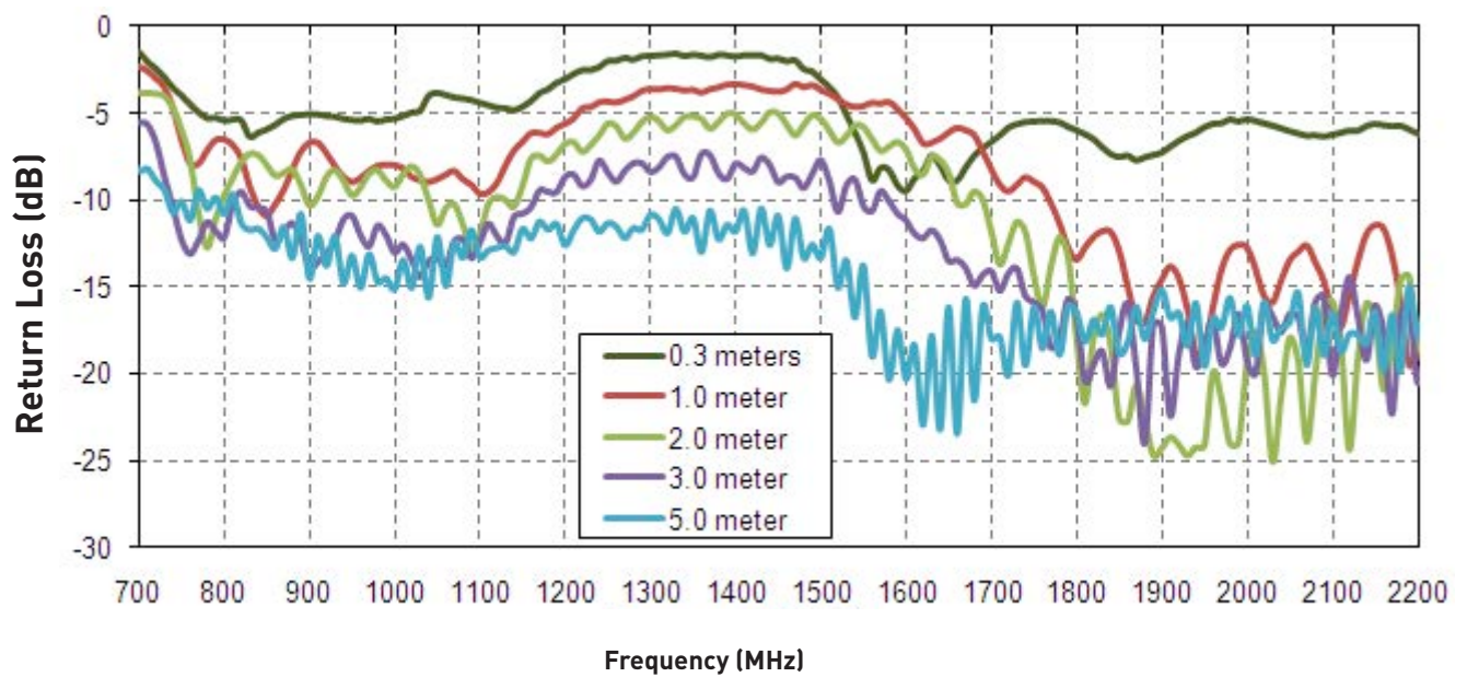
Figure 4. Return Loss of G21 Hercules antenna on 60cm metal plate
