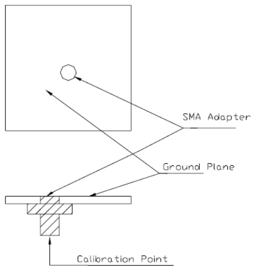
Test Fixture
