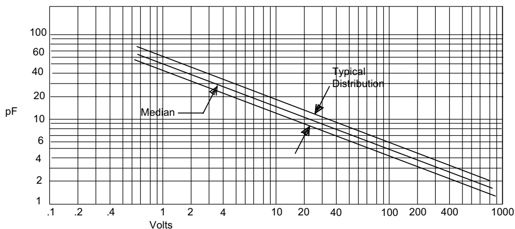
Figure 2 Junction Capacitance
