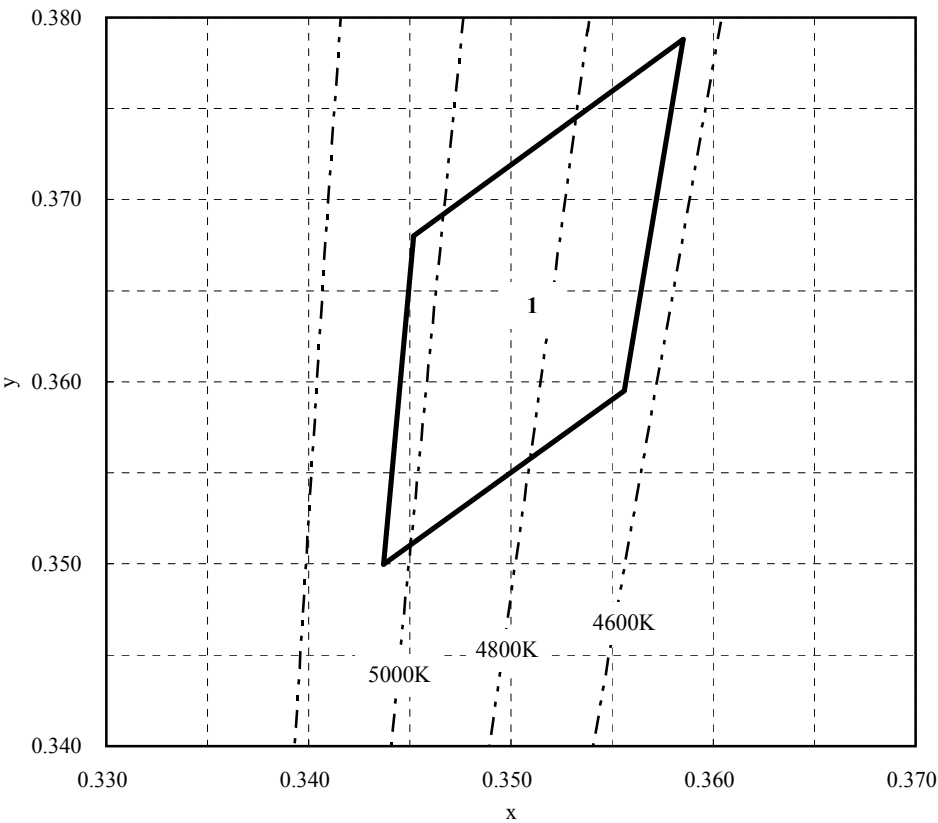
Chromaticity Diagram
