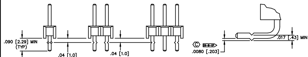
CRIMP DETAIL
