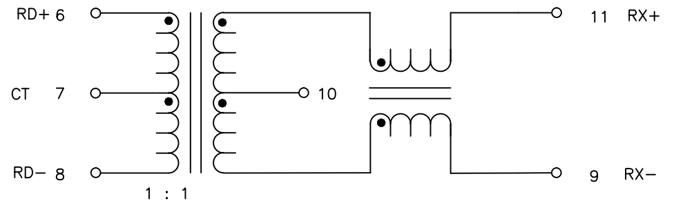
SCHEMATIC
