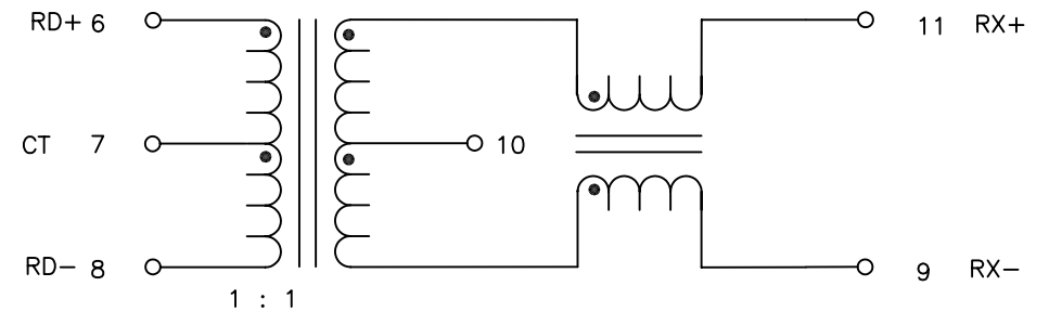
SCHEMATIC
