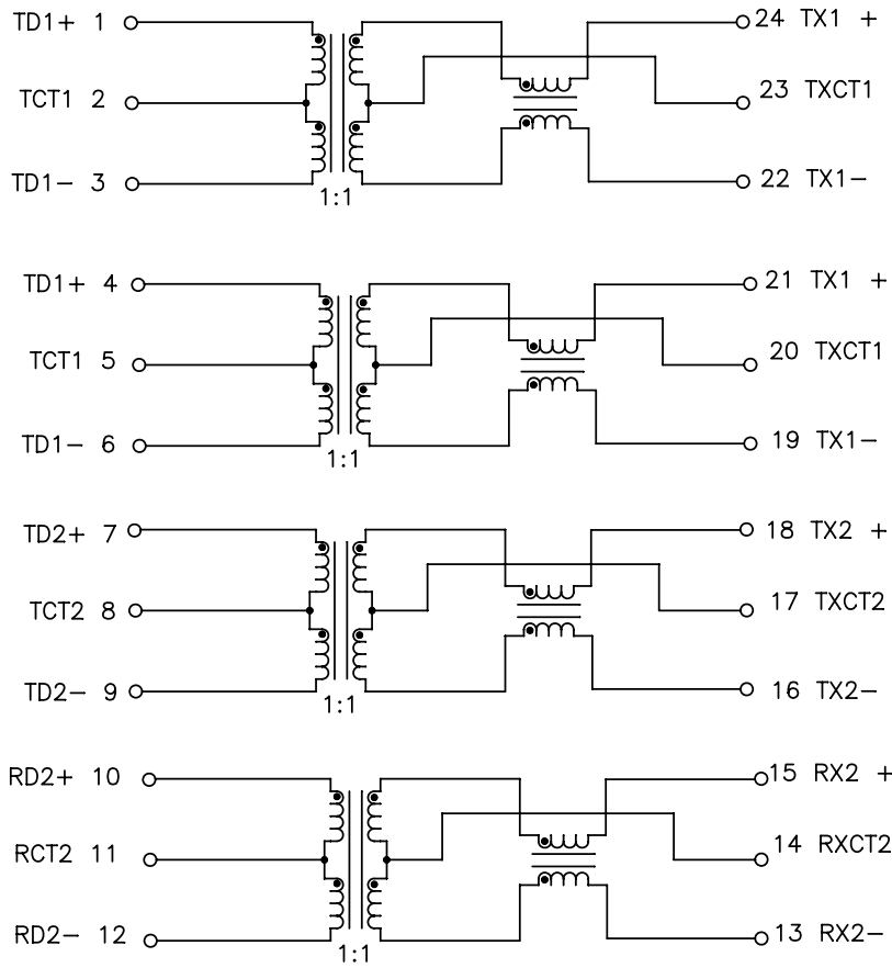
SCHEMATIC
