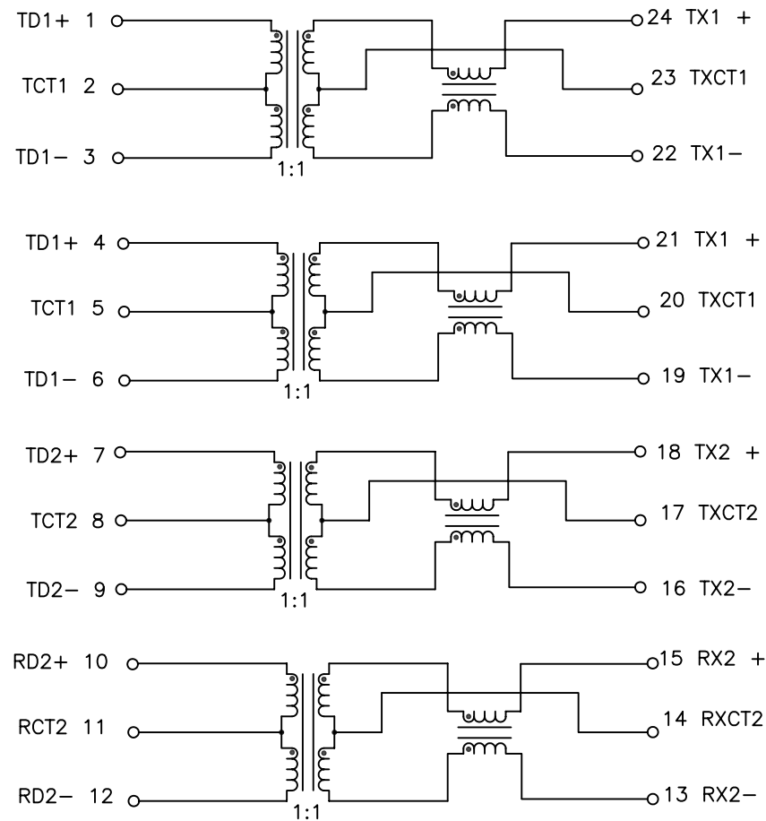
SCHEMATIC
