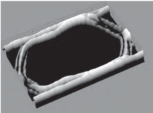
Fig 7. Eye diagram using reference PCB
