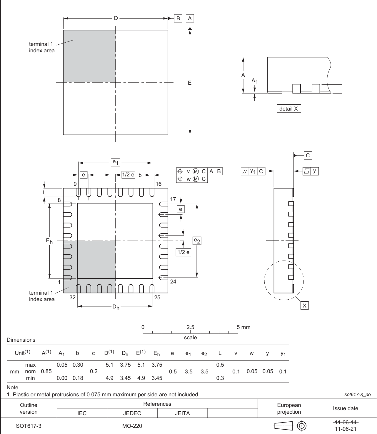
Fig 24. Package outline DFN5050-32 (SOT617-3/HVQFN32)
