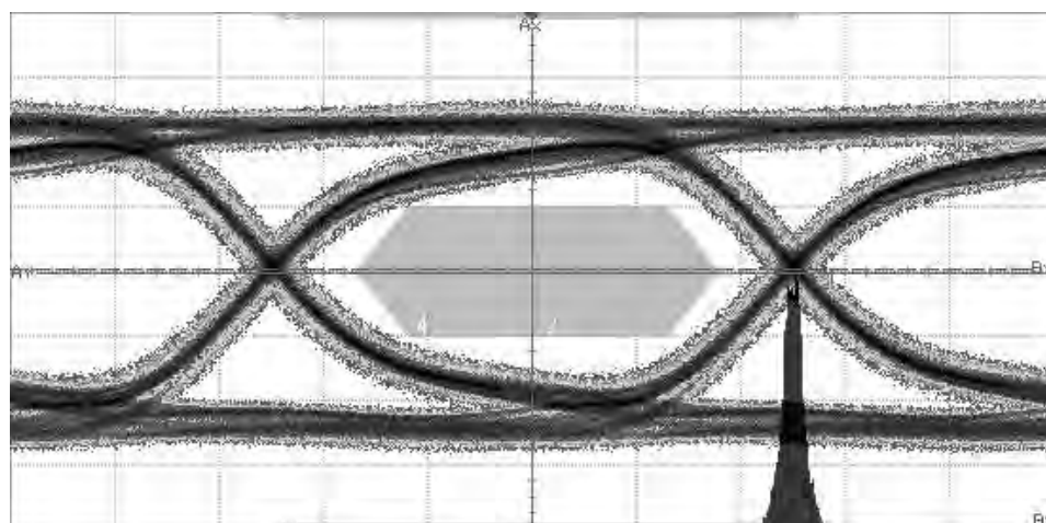
Fig 4. Eye diagram using IP4788CZ32 (1080p, 12 bit)
