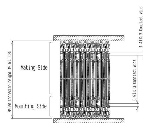
Mating Cross Section (Free)
