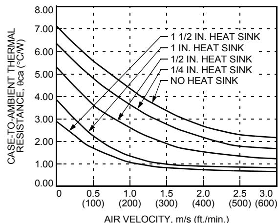
Figure 33. JAHW050A and JAHW075A Case-to-Ambient Thermal Resistance Curves; Either Orientation
