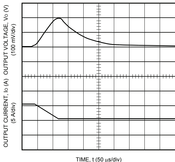
Figure 13. Typical JAHW050A Transient Response to Step Decrease in Load from 50% to 25% of I_{o, \max} at Room Temperature and 48 Vdc Input (Waveform Averaged to Eliminate Ripple Component.)
