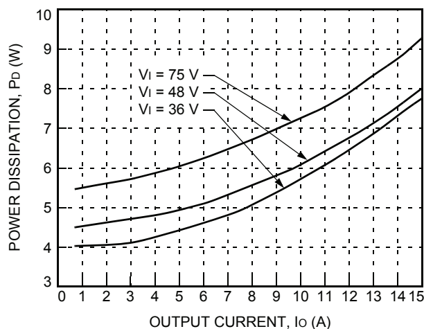
Figure 31. JAHW075A Power Dissipation vs. Output Current at 25 °C
