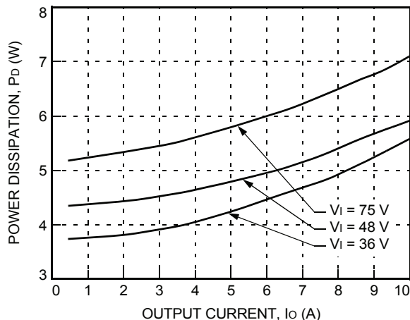
Figure 30. JAHW050A Power Dissipation vs. Output Current at 25 °C
