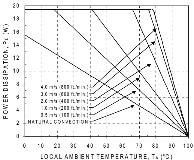
Figure 29. JAHW100A Forced Convection Power Derating with No Heat Sink; Either Orientation
