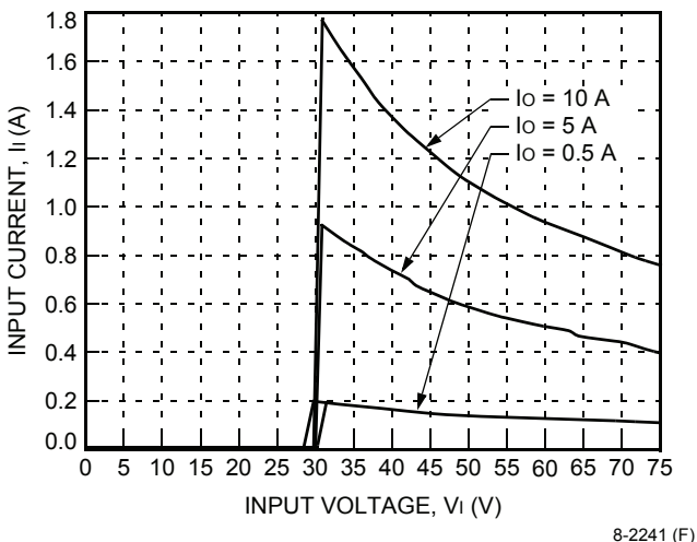
Figure 1. Typical JAHW050A Input Characteristics at Room Temperature
