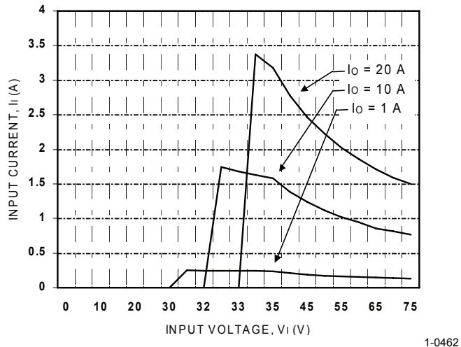
Figure 3. Typical JAHW100A Input Characteristics at Room Temperature
