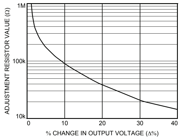
Figure 25. Resistor Selection for Decreased Output Voltage
