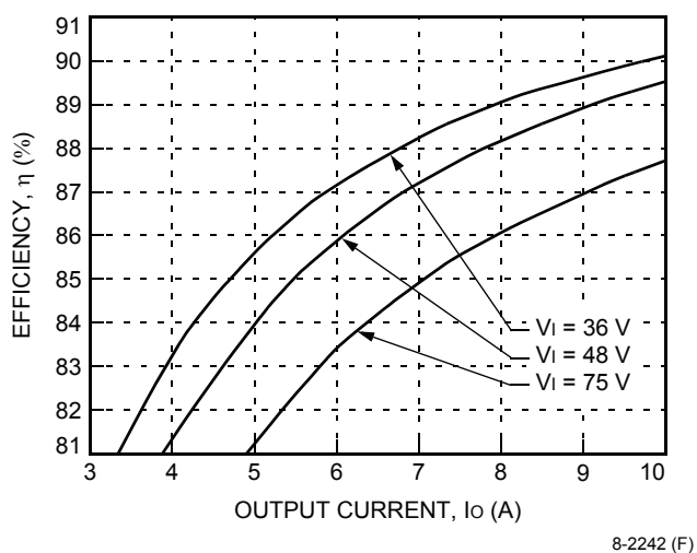
Figure 4. Typical JAHW050A Converter Efficiency vs. Output Current at Room Temperature
