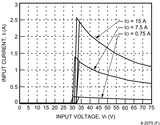
Figure 2. Typical JAHW075A Input Characteristics at Room Temperature
