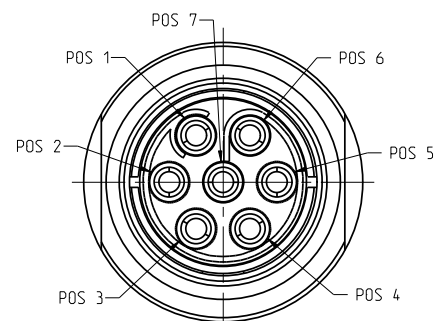
WIRE SIDE VIEW ( 'COLLET SET' NOT SHOWN)
