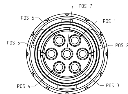
MATING SIDE VIEW
