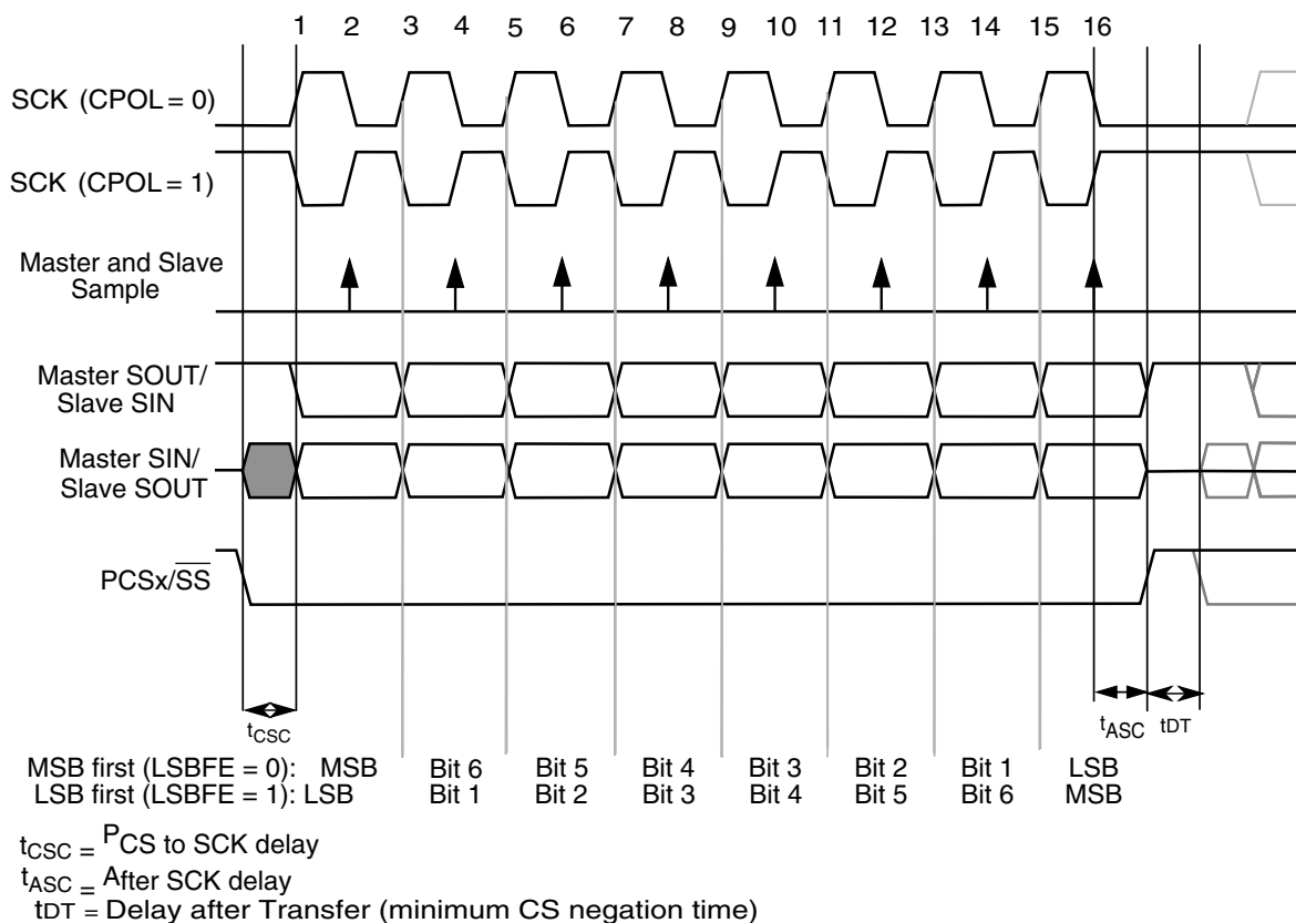
Figure 43-95. DSPI Transfer Timing Diagram (MTFE=0, CPHA=1, FMSZ=8)
