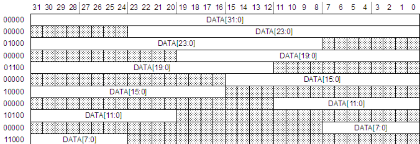
Figure 42-51. SAI first bit shifted, LSB first
