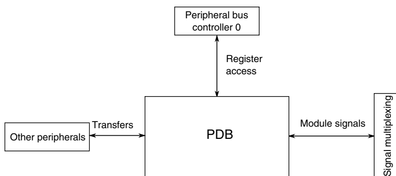
Figure 3-31. PDB configuration
