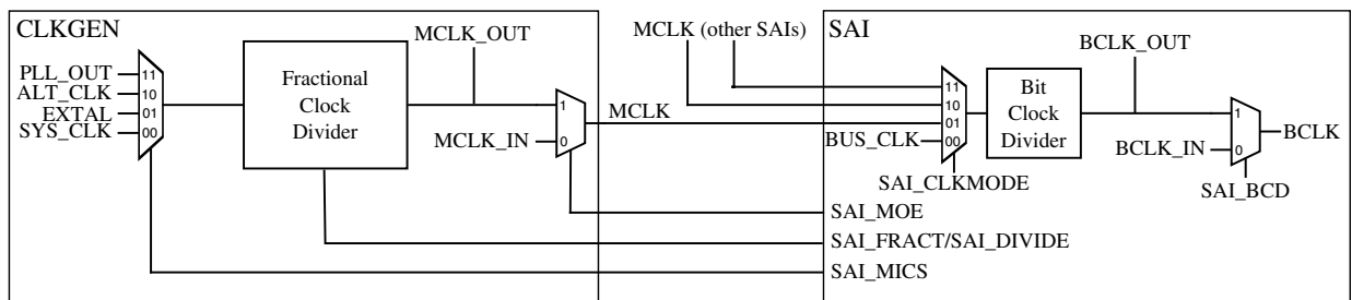
Figure 43-50. SAI master clock generation
