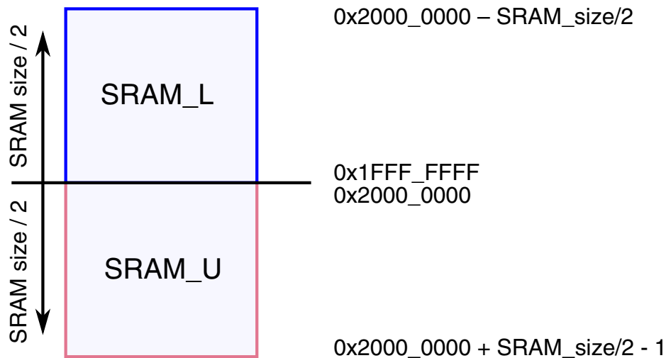
Figure 3-23. SRAM blocks memory map
