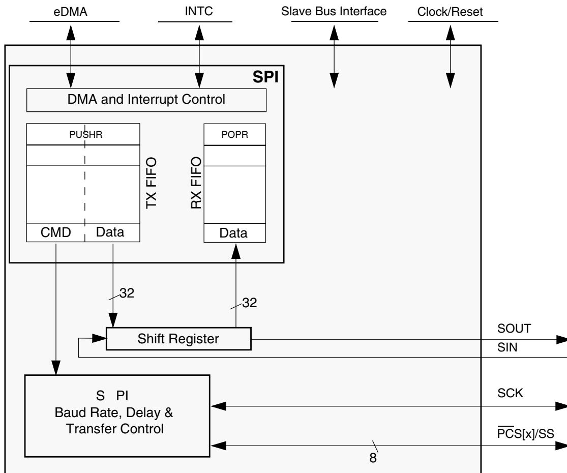
Figure 40-1. DSPI Block Diagram
