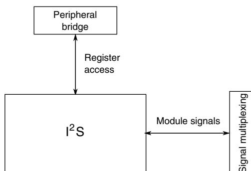
Figure 3-44. I²S configuration
