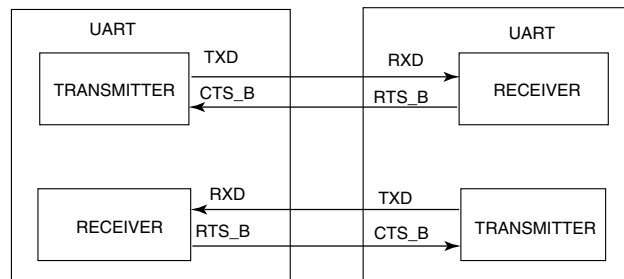
Figure 42-218. Ready-to-receive
