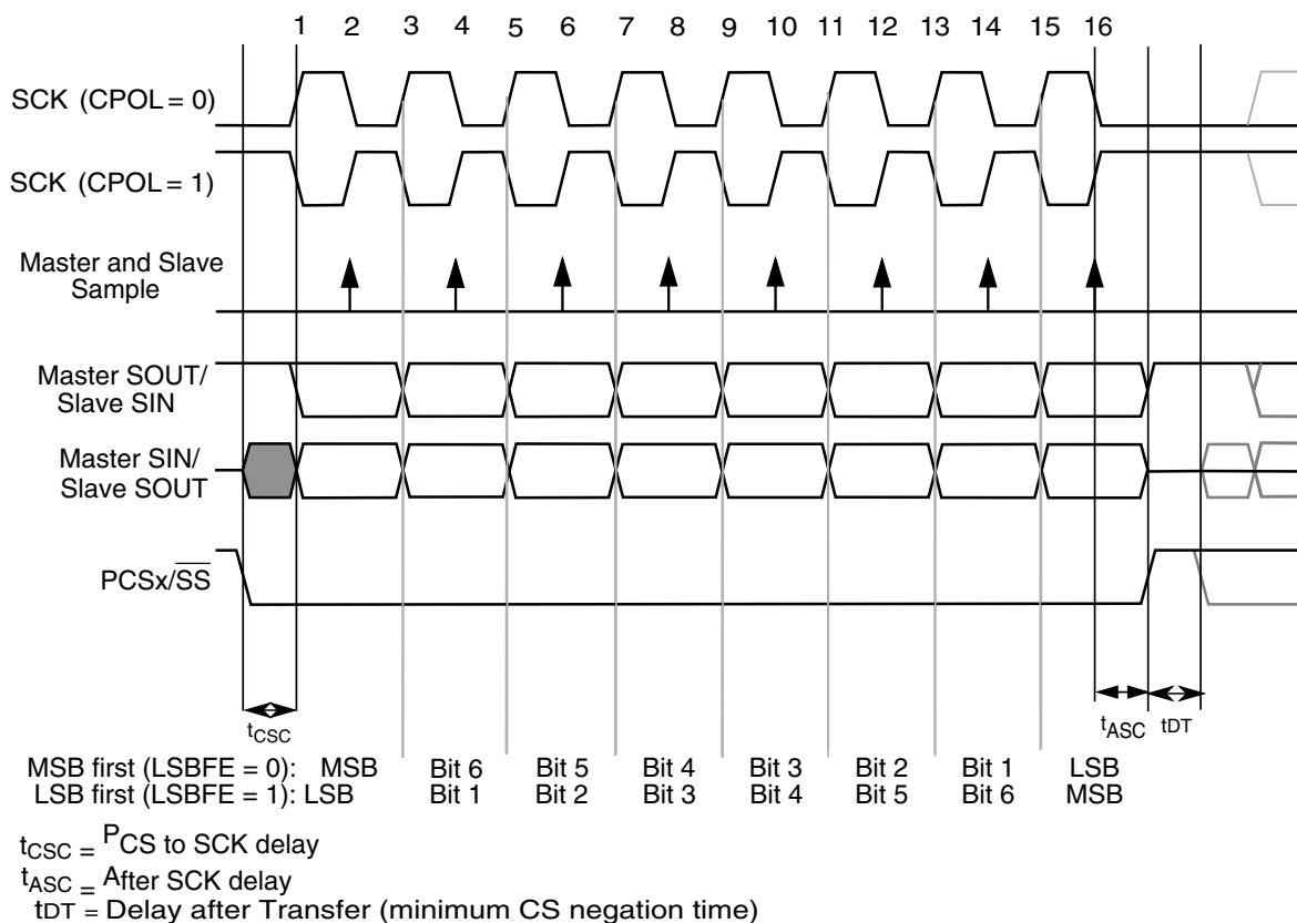
Figure 40-50. DSPI transfer timing diagram (MTFE=0, CPHA=1, FMSZ=8)
