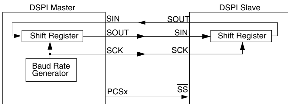
Figure 44-69. SPI serial protocol overview
