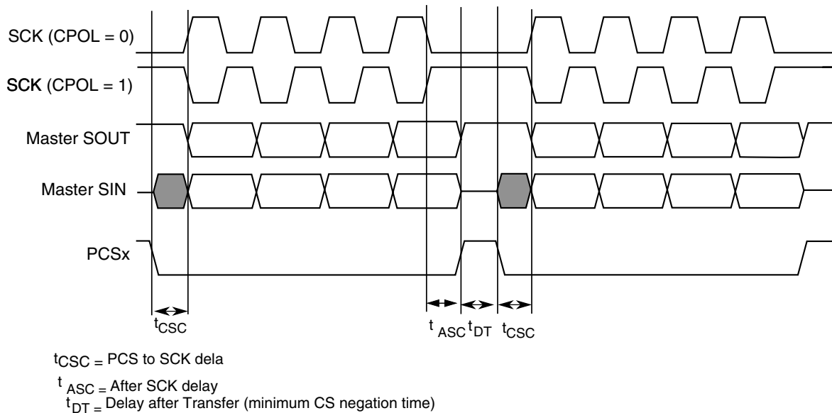
Figure 46-95. Example of non-continuous format (CPHA=1, CONT=0)
