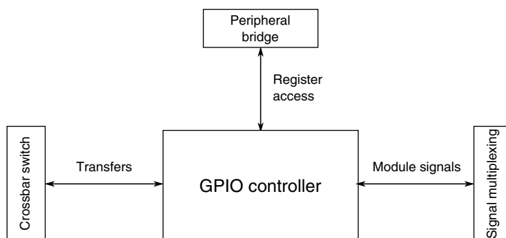
Figure 3-61. GPIO configuration
