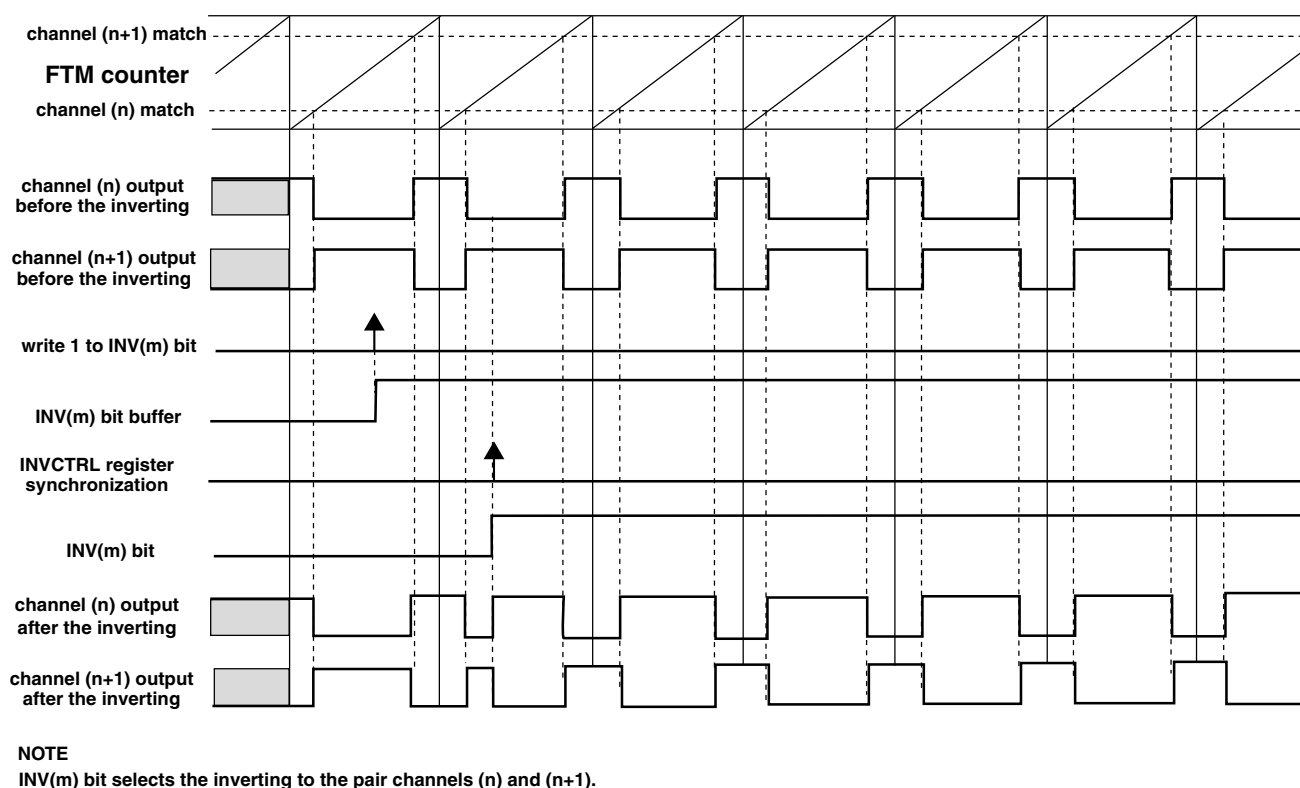
Figure 37-226. Channels (n) and (n+1) outputs after the inverting in Low-True (ELSnB:ELSnA = X:1) Combine mode
