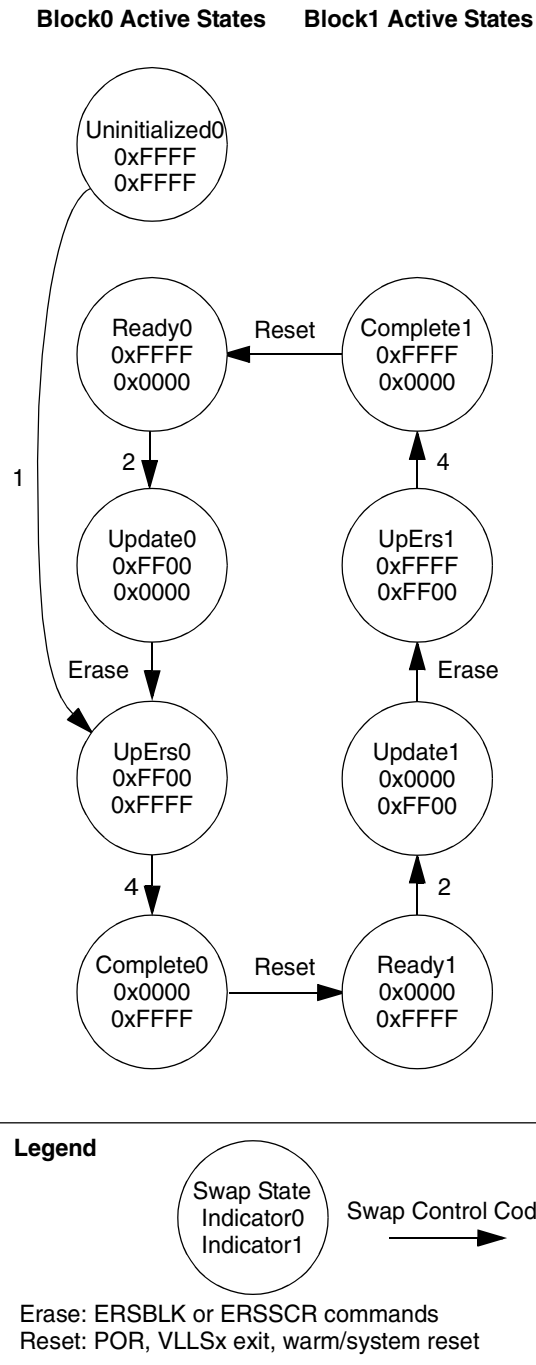
Figure 28-27. Valid Swap State Sequencing
