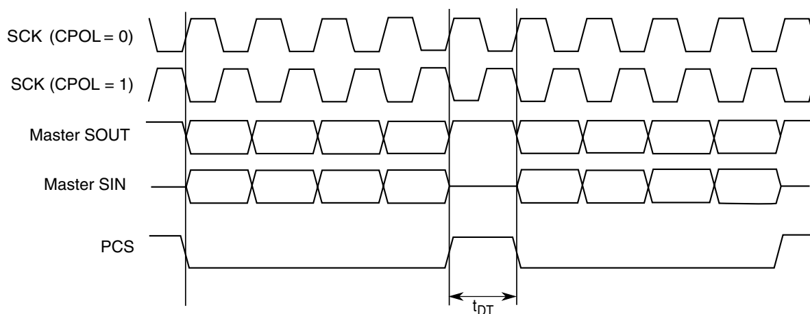
Figure 46-97. Continuous SCK Timing Diagram (CONT=0)
