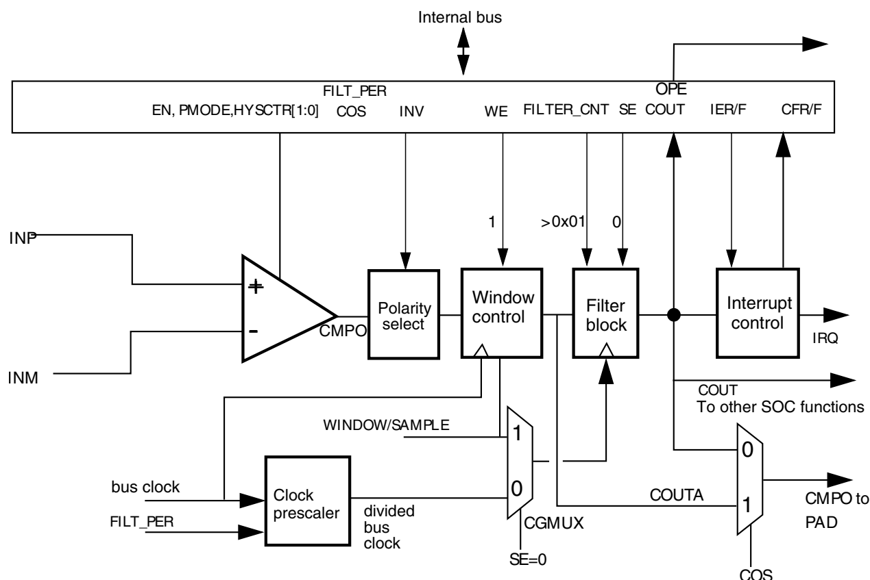
Figure 33-35. Windowed/Filtered mode
