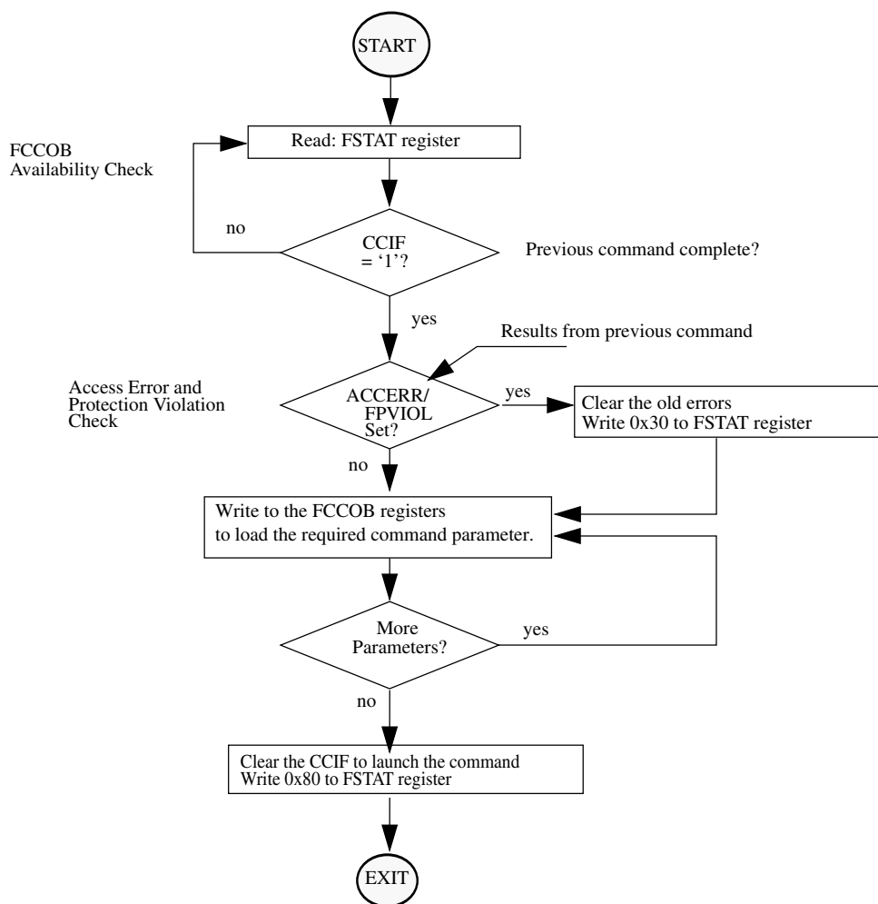
Figure 28-25. Generic Flash Command Write Sequence Flowchart
