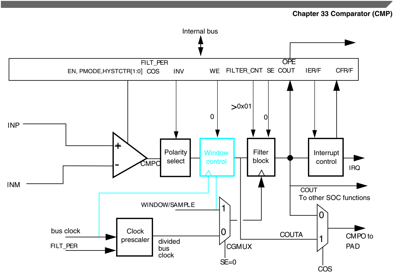
Figure 33-31. Sampled, Filtered (# 4B): sampling point internally derived
