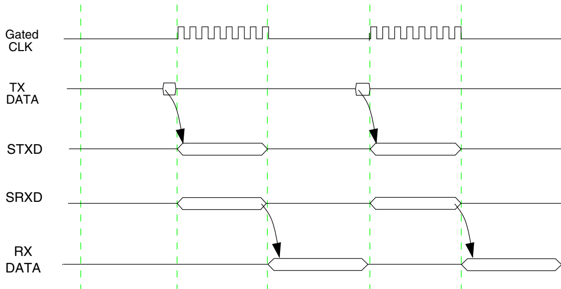
Figure 50-48. Normal mode timing - external gated clock
