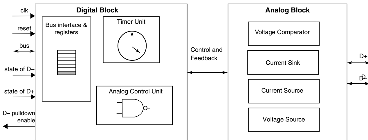
Figure 41-1. Block diagram
