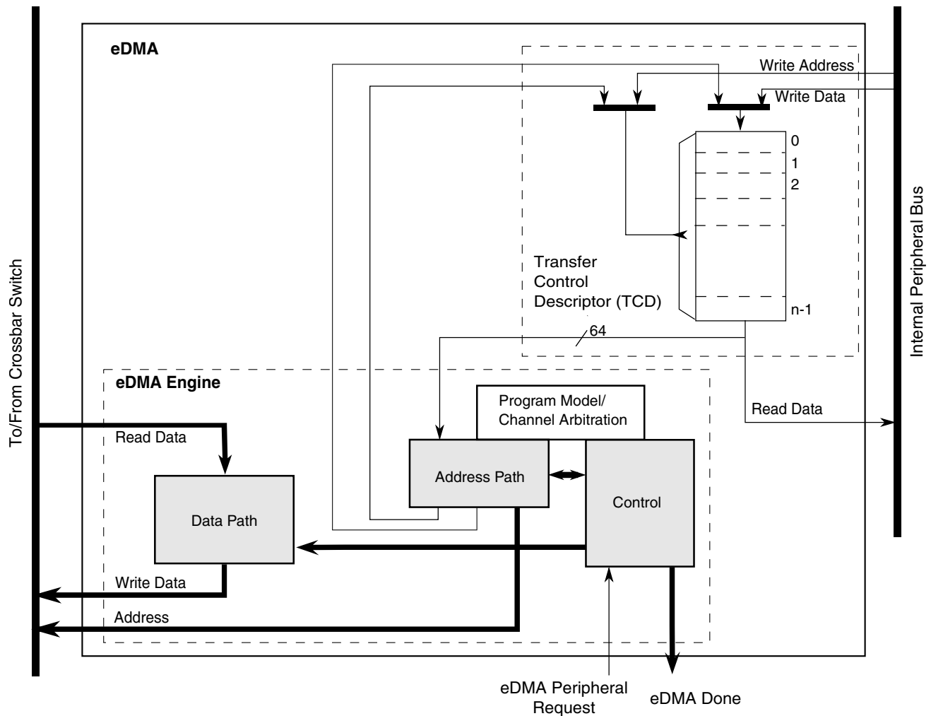
Figure 21-99. eDMA operation, part 2
