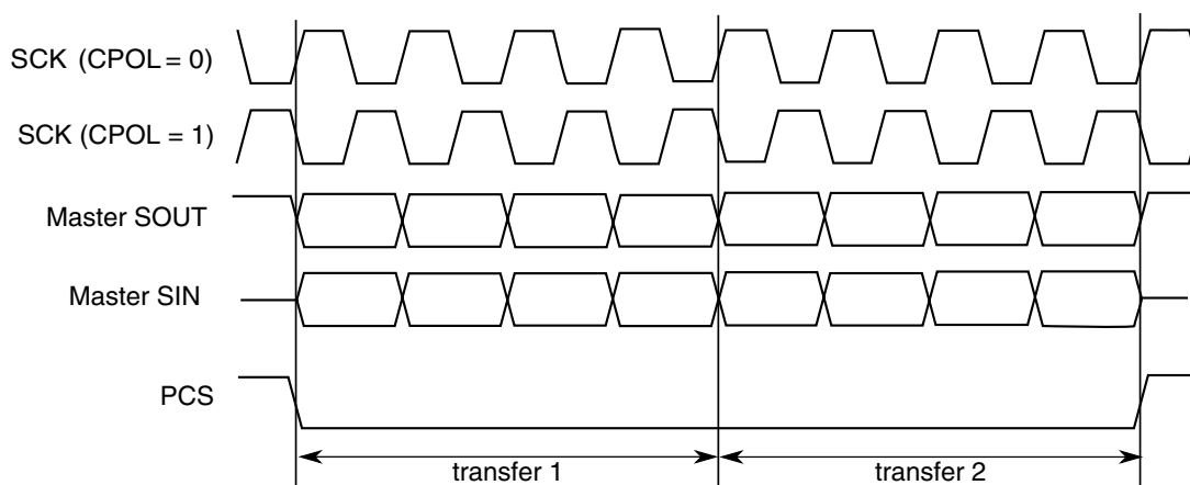
Figure 47-76. Continuous SCK timing diagram (CONT=1)
