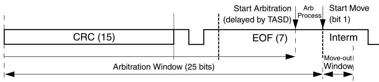
Figure 46-101. Arbitration and move-out time windows
