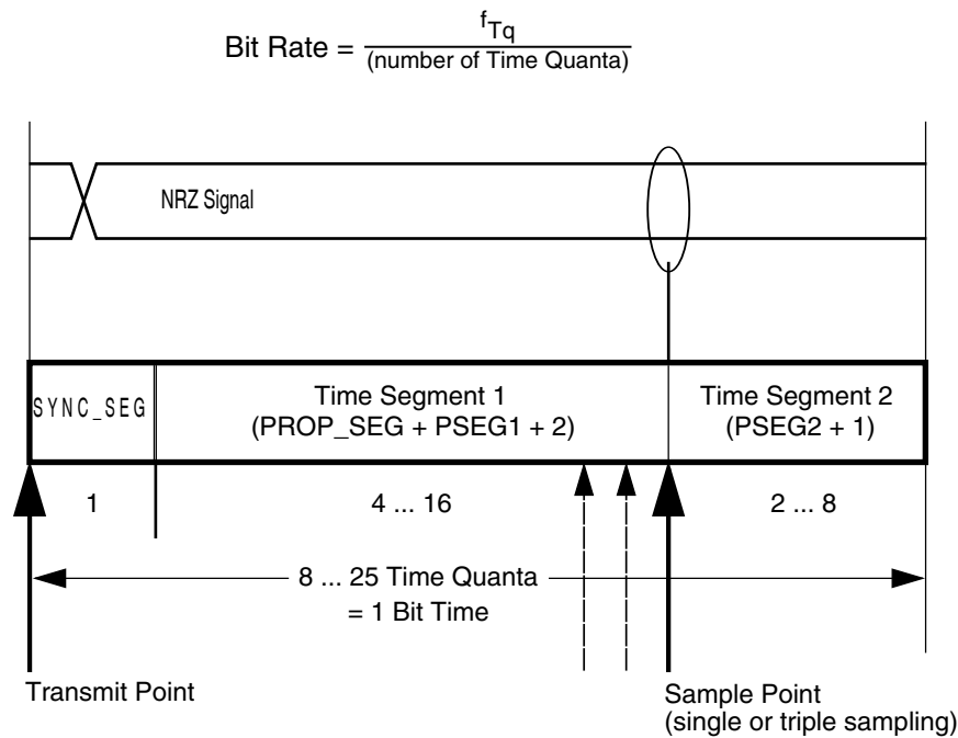
Figure 46-99. Segments within the bit time
