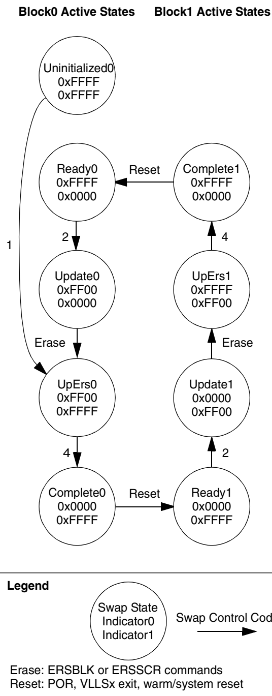
Figure 29-27. Valid Swap State Sequencing
