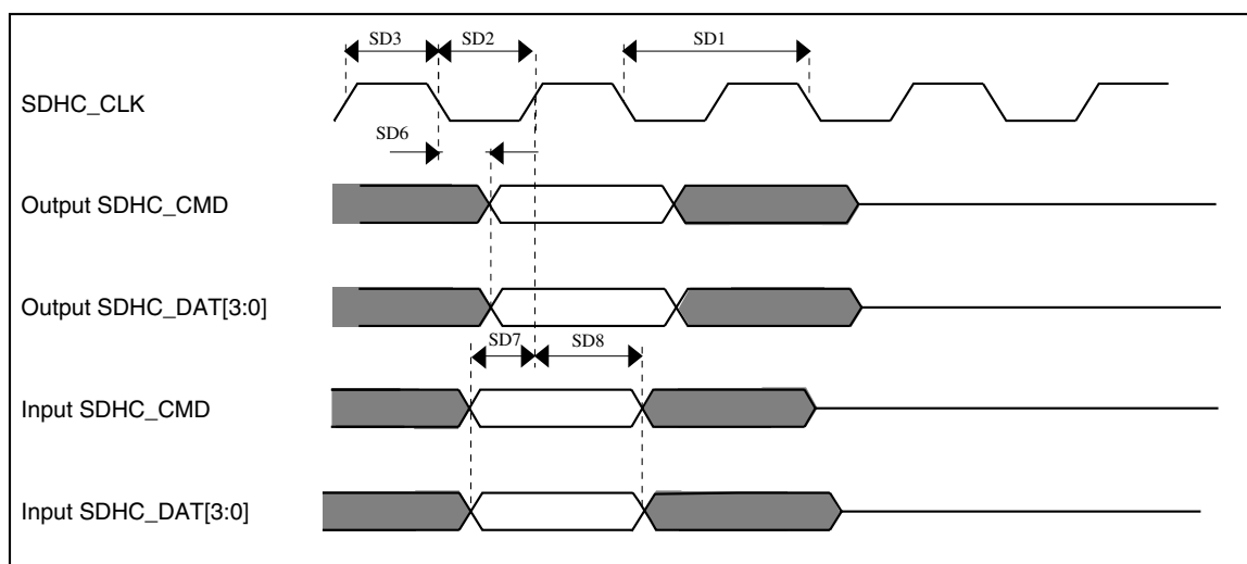
Figure 22. SDHC timing
