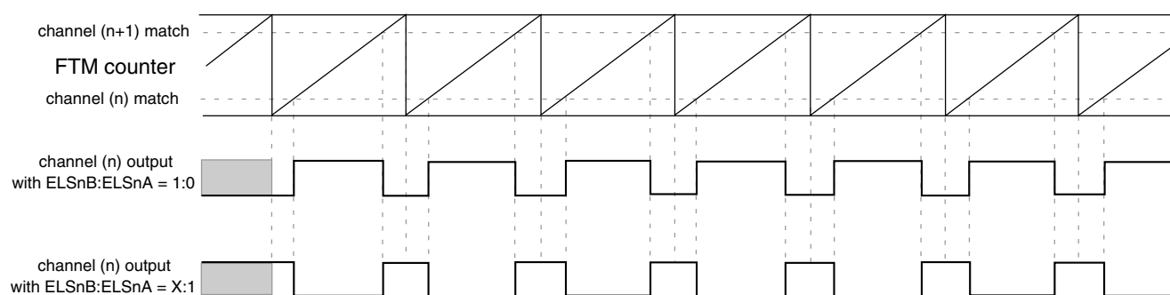
Figure 37-187. Combine mode
