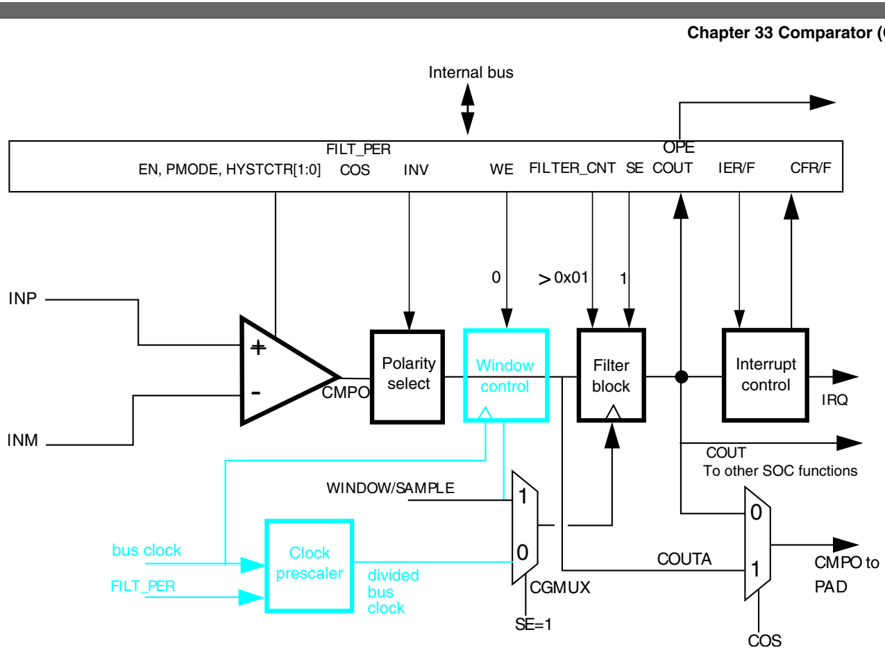
Figure 33-30. Sampled, Filtered (# 4A): sampling point externally driven
