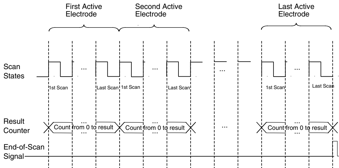
Figure 52-41. Scan sequence
