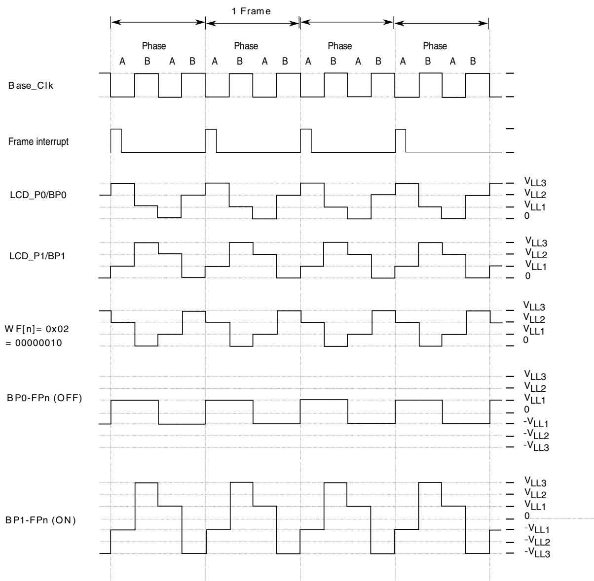
Figure 53-29. 1/2 duty and 1/3 bias (low-power waveform)
