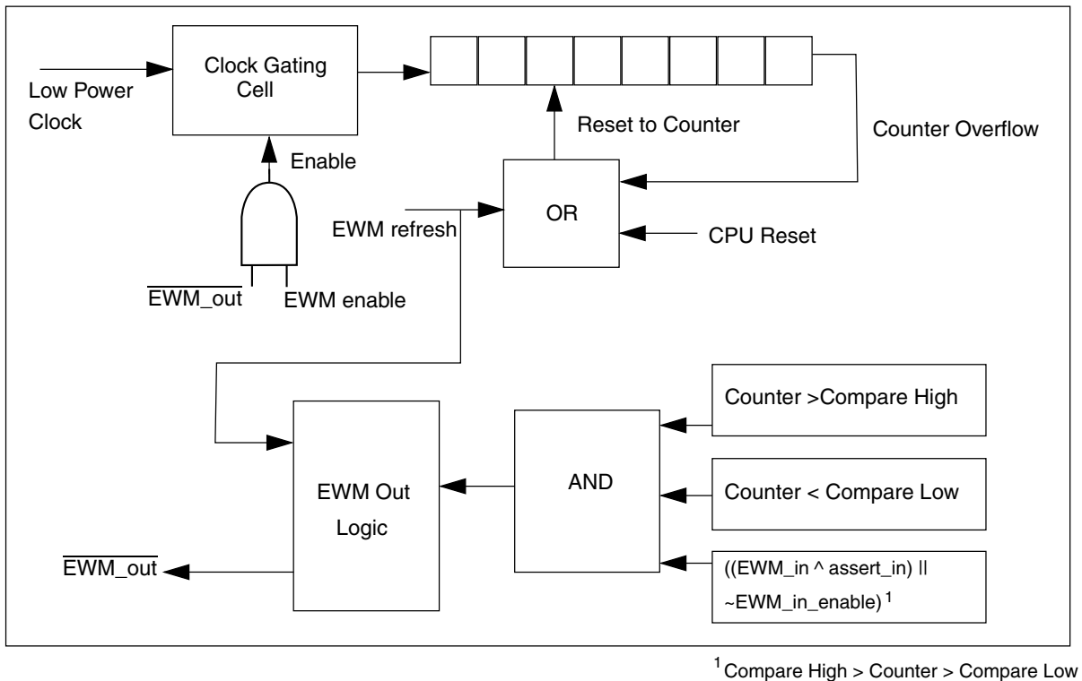
Figure 23-1. EWM Block Diagram
