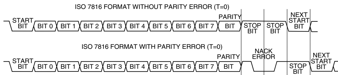
Figure 48-304. ISO-7816 T = 0 data format
