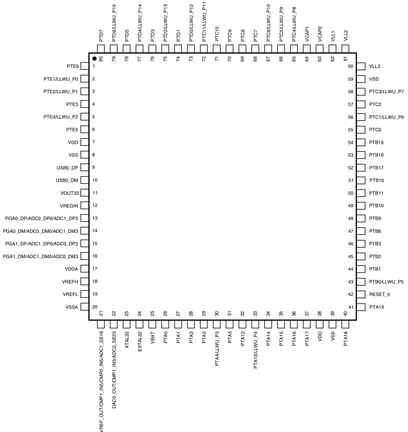
Figure 10-3. K40 80 LQFP Pinout Diagram
