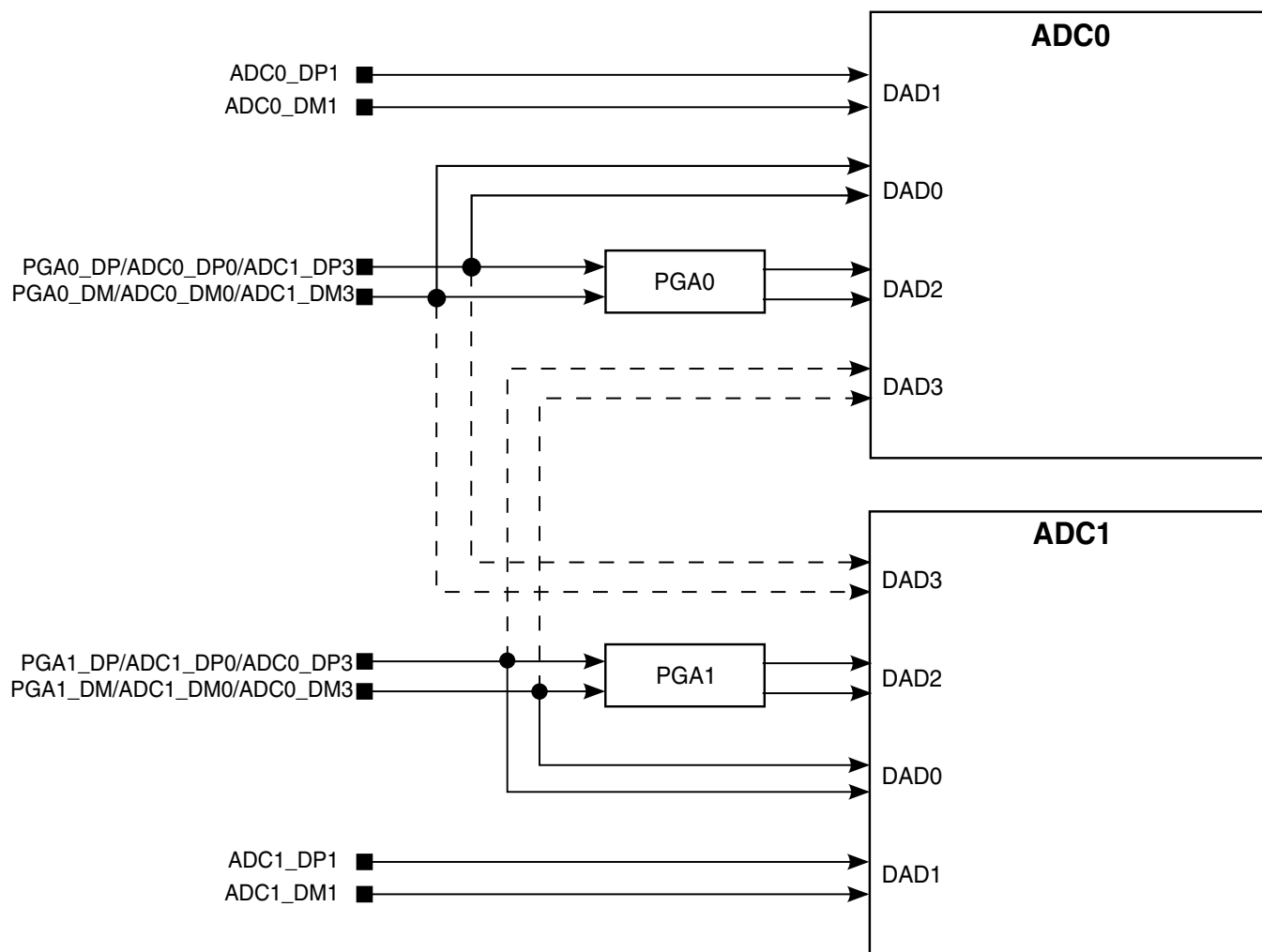
Figure 3-38. PGA Integration
