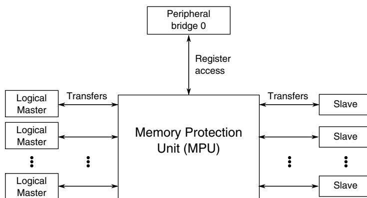
Figure 3-11. Memory Protection Unit configuration
