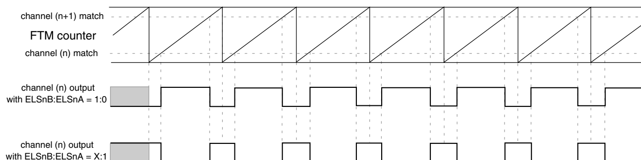
Figure 39-187. Combine Mode
