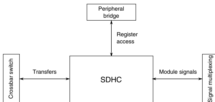
Figure 3-62. SDHC configuration
