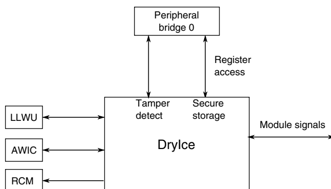
Figure 3-34. Drylce configuration
