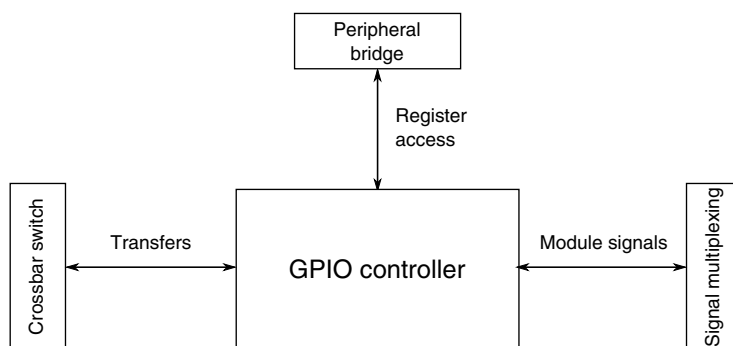
Figure 3-64. GPIO configuration
