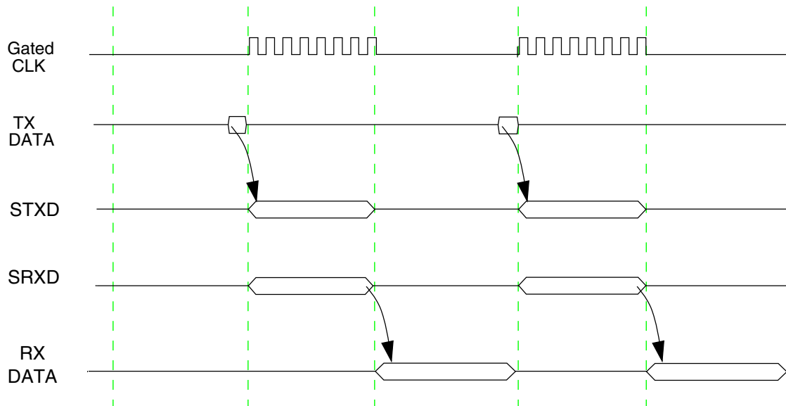
Figure 51-48. Normal mode timing - external gated clock
