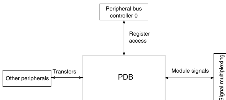
Figure 3-44. PDB configuration
