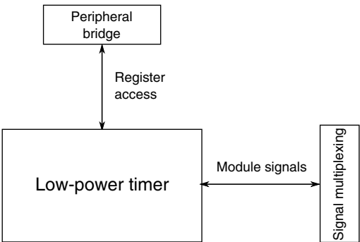
Figure 3-49. LPT configuration
