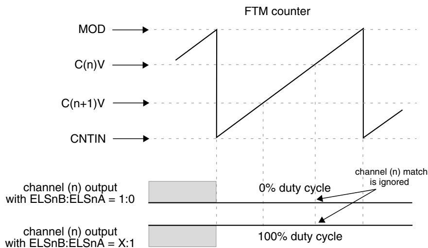
Figure 41-197. Channel (n) Output If (\text{CNTIN} < C(n)V < \text{MOD}) and (\text{CNTIN} < C(n+1)V < \text{MOD}) and (C(n)V > C(n+1)V)
