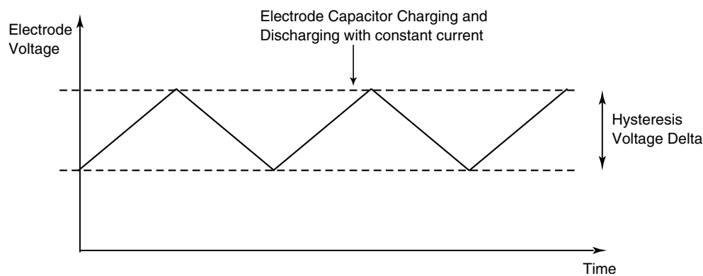
Figure 56-65. TSI electrode oscillator chart
