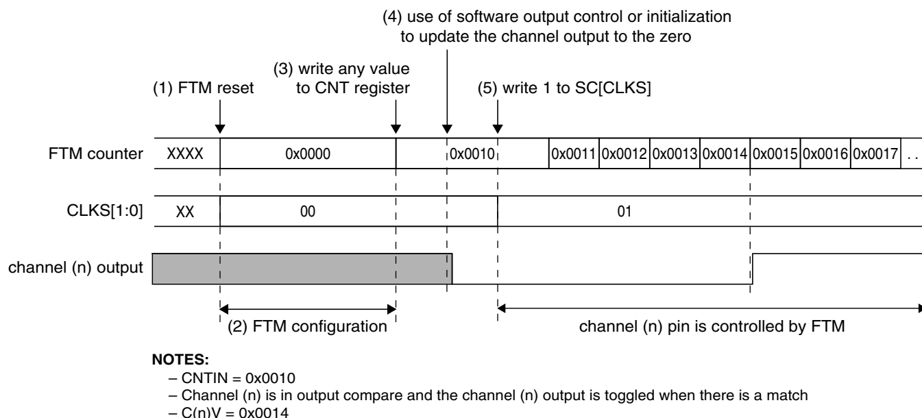
Figure 41-260. FTM Behavior After Reset When the Channel (n) Is in Output Compare Mode
