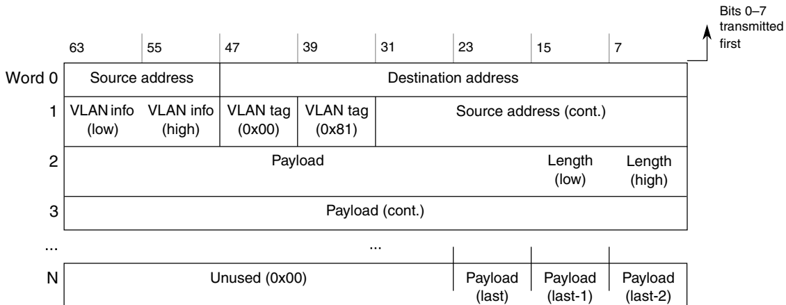
Figure 46-65. VLAN tagged Frame 64-bit Mapping Example
