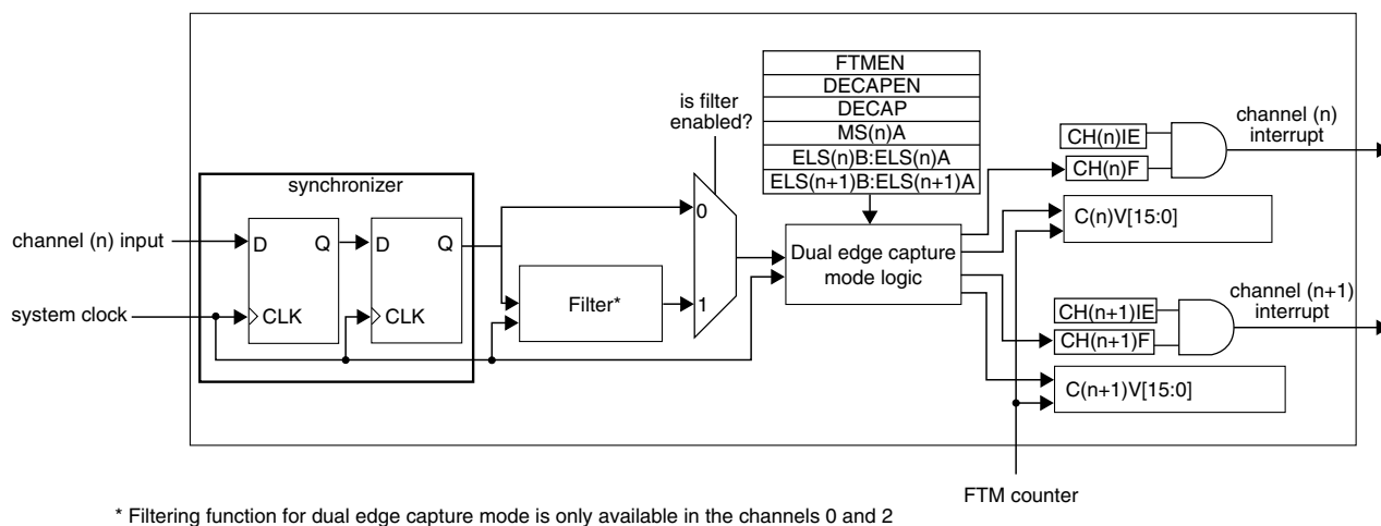
Figure 41-244. Dual Edge Capture Mode Block Diagram
