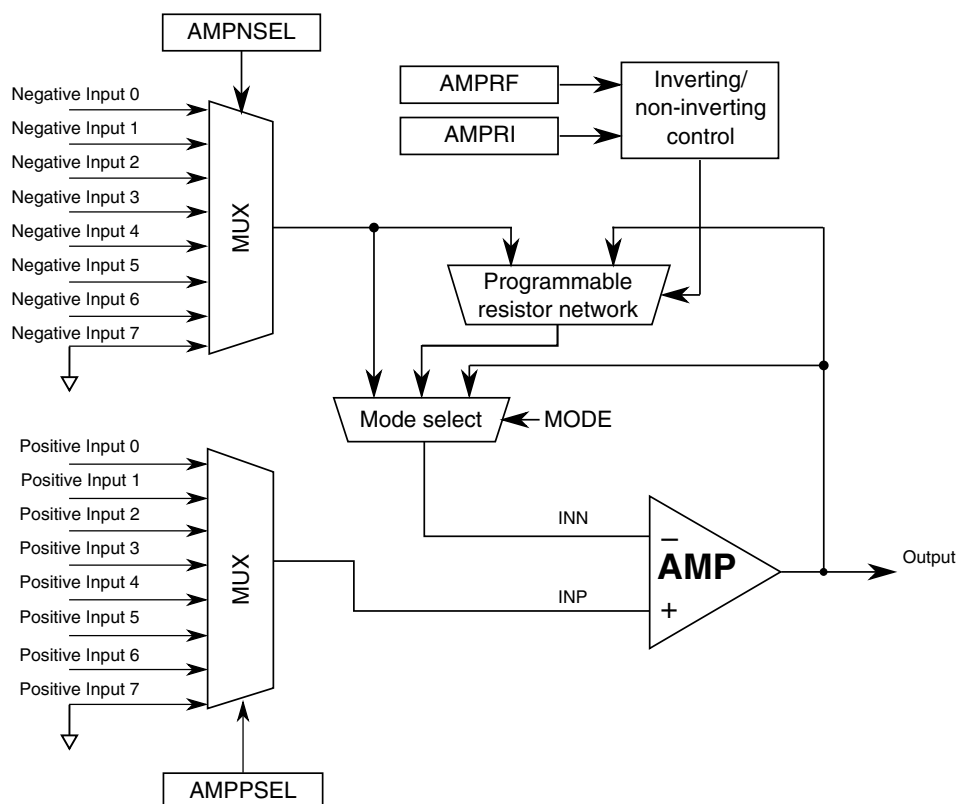
Figure 37-1. Op-Amp Block Diagram
