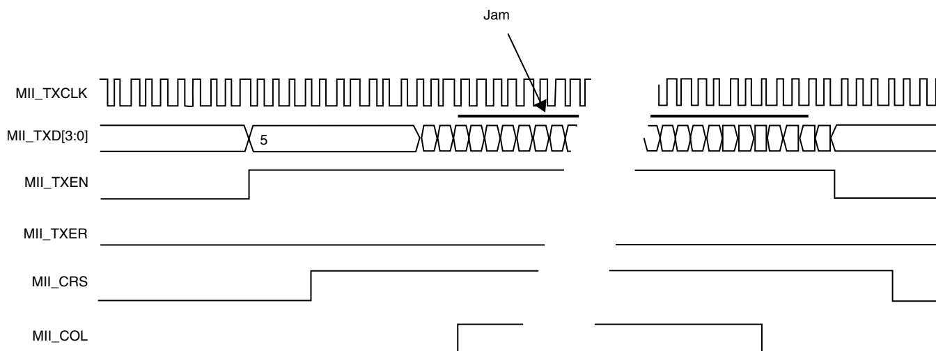
Figure 46-74. MII Transmit Operation — Transmission with Collision
