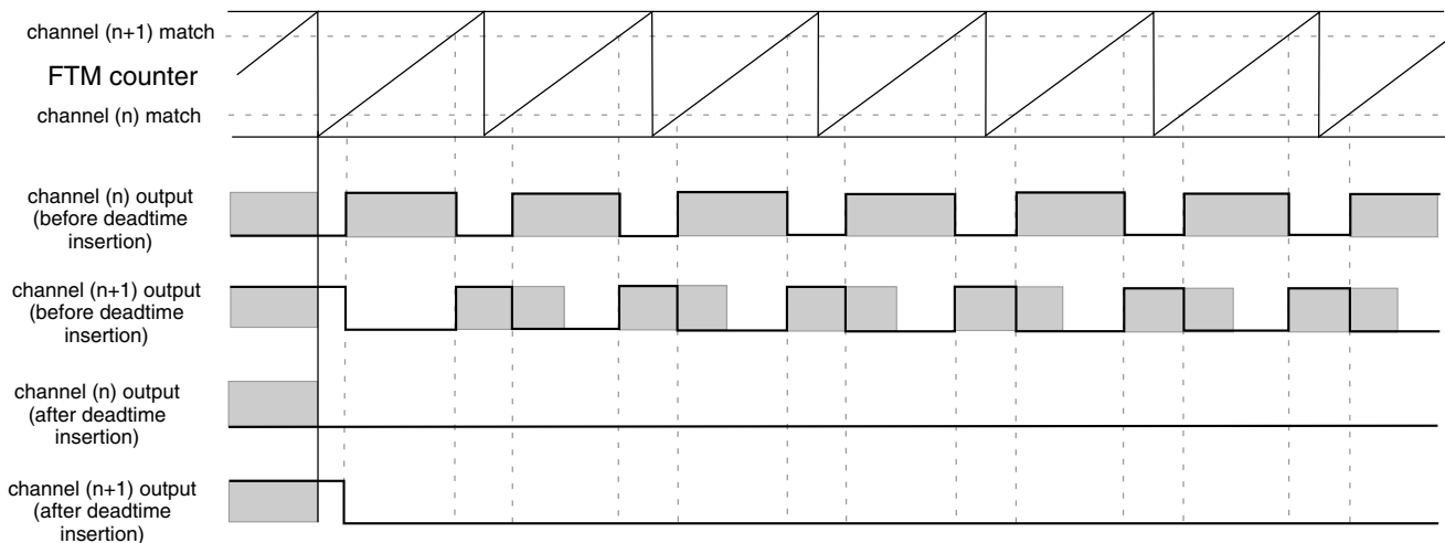
Figure 41-231. Example of the Deadtime Insertion (ELSnB:ELSnA = 1:0, POL(n) = 0, and POL(n+1) = 0) when the Deadtime Delay Is Comparable To Channels (n) and (n+1) Duty Cycle
