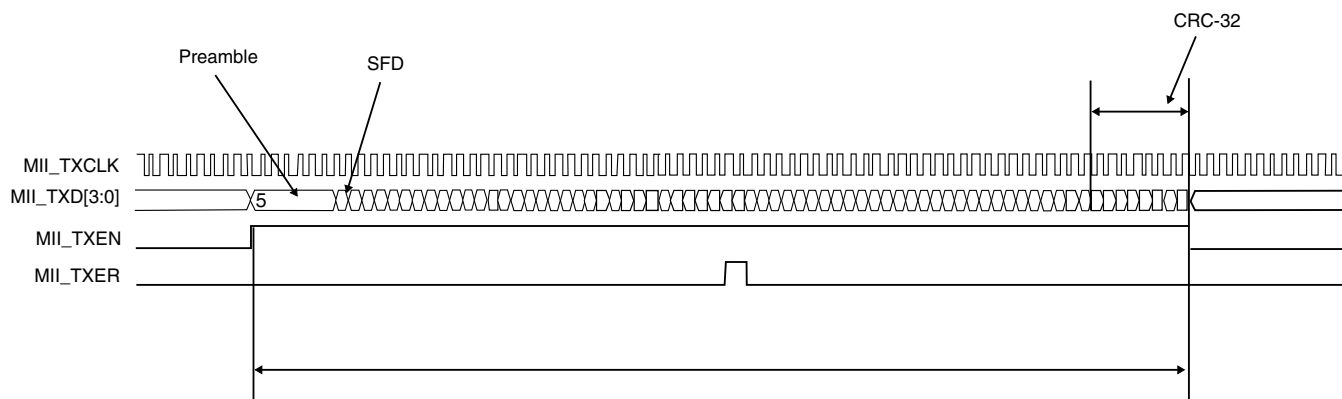
Figure 46-73. MII Transmit Operation — Errored Frame
