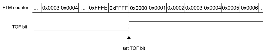
Figure 41-172. Example When the FTM Counter Is a Free Running
