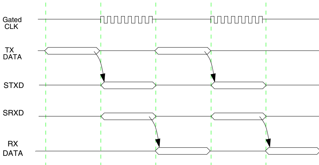
Figure 54-47. Normal mode timing - internal gated clock
