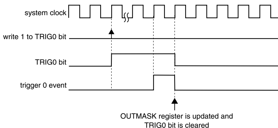
Figure 41-216. OUTMASK Synchronization with (SYNCMODE = 0), (HWTRIGMODE = 0), (SYNCHOM = 1), (PWMSYNC = 0), and (a Hardware Trigger Was Used)
