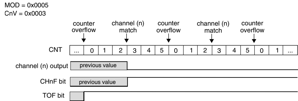
Figure 41-179. Example of the Output Compare Mode when the Match Clears the Channel Output
