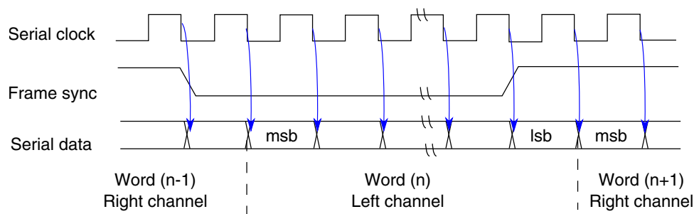
Figure 54-54. I 2 S mode timing - serial clock, frame sync and serial data
