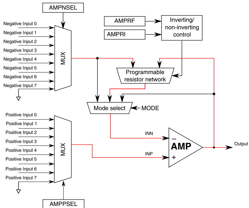
Figure 37-13. Operational Amplifier Block Diagram in Non-Inverting/Inverting PGA Mode
