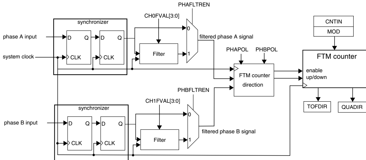
Figure 41-250. Quadrature Decoder Block Diagram
