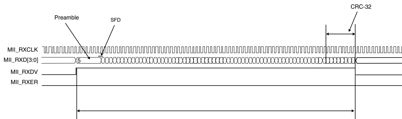
Figure 46-75. MII Receive Operation
