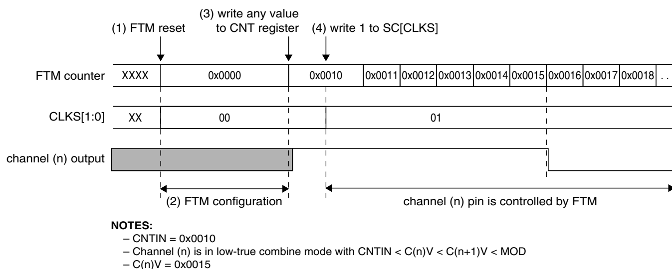
Figure 41-259. FTM Behavior After Reset When the Channel (n) Is in Combine Mode
