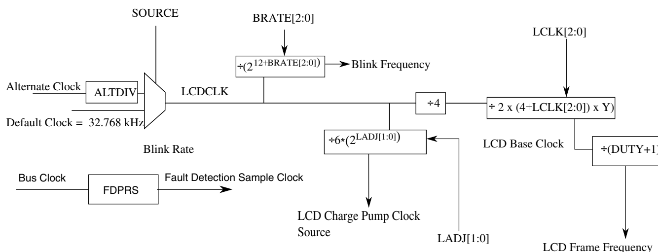
Figure 57-28. LCD clock tree
