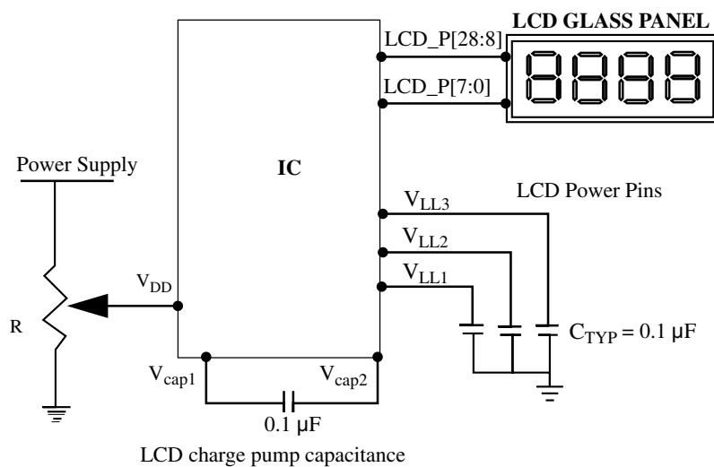
Figure 57-43. Power connections for contrast control
