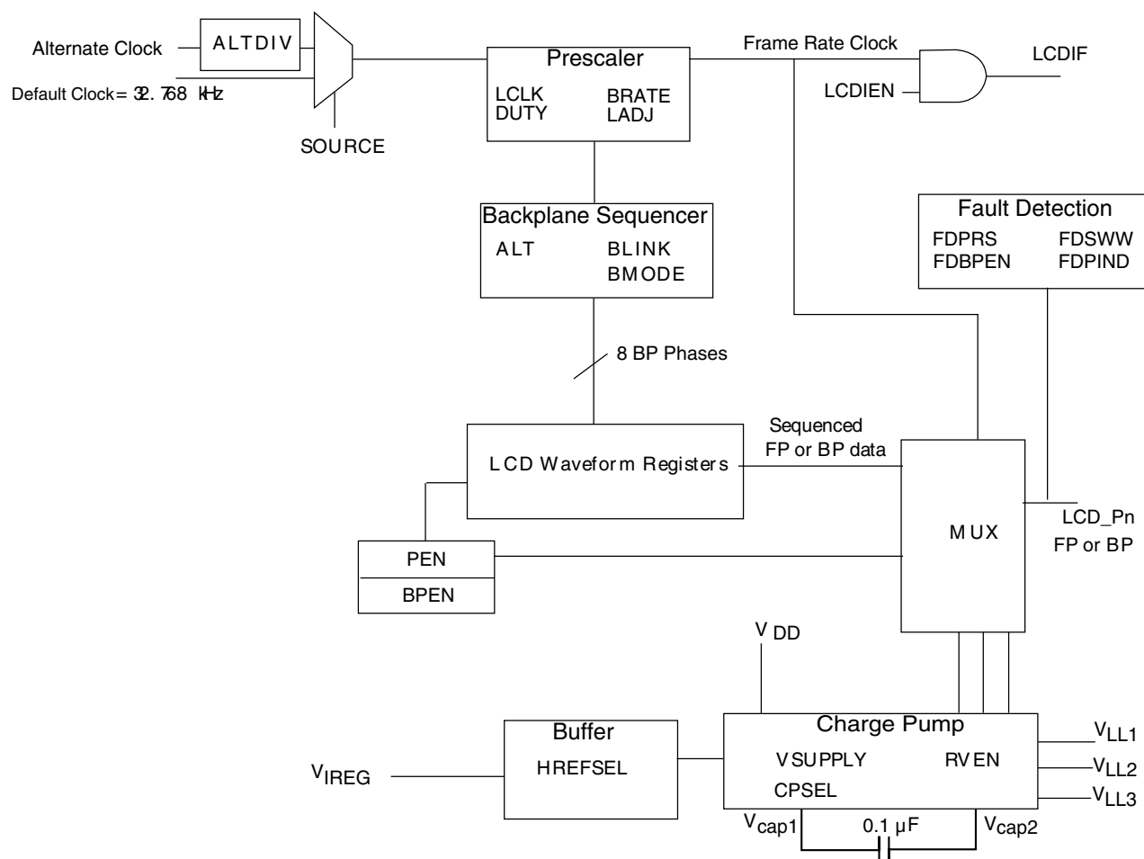
Figure 57-1. LCD controller block diagram
