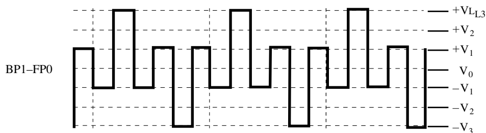
Figure 57-41. "f" segment voltage waveform
