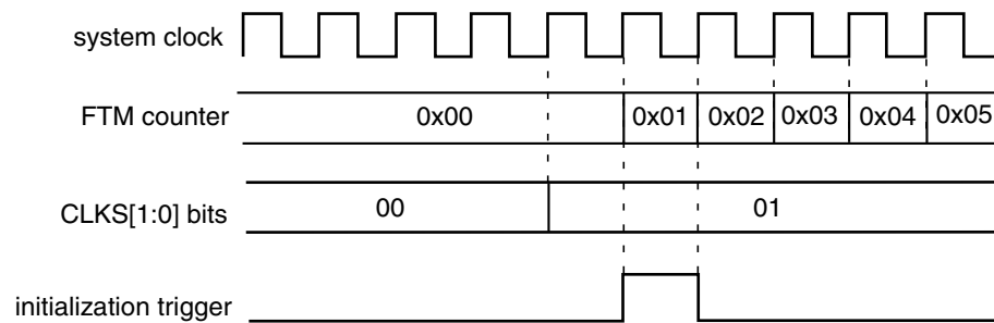
Figure 41-242. Initialization Trigger Is Generated If (CNT = CNTIN), (CLKS[1:0] = 0:0), and a Value Different From Zero Is Written to CLKS[1:0] Bits
