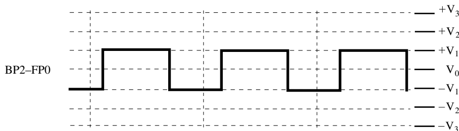
Figure 57-42. "e" segment voltage waveform
