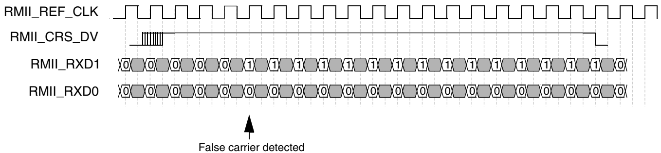
Figure 46-70. RMII receive operation with false carrier
