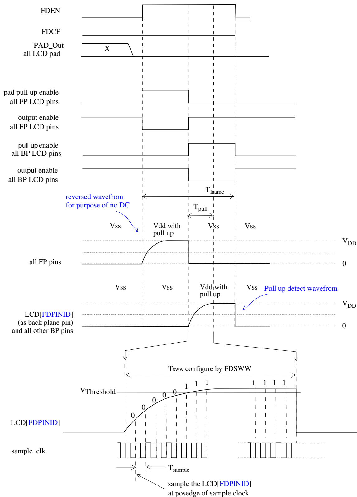
Figure 57-37. Pullup fault detection timing diagram, while FDBPEN is 1
