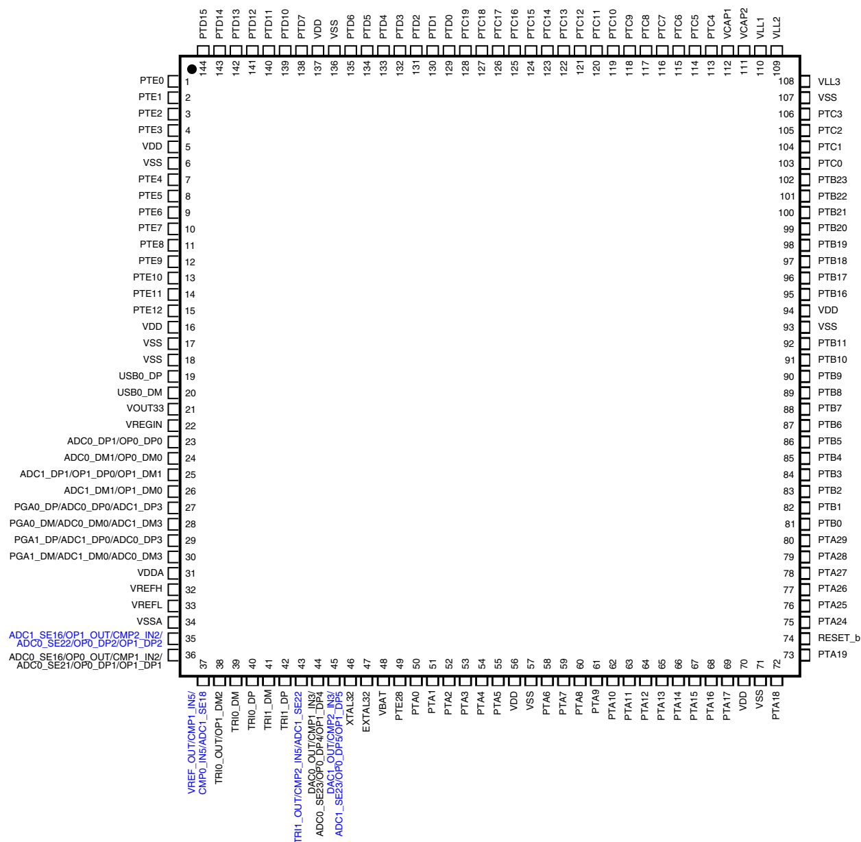
Figure 10-2. K53 144 LQFP Pinout Diagram
