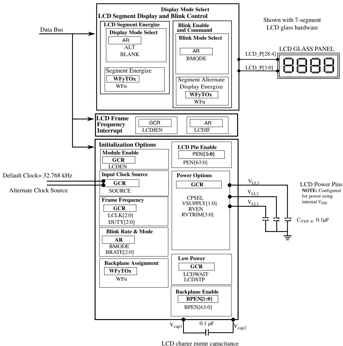
Figure 57-38. LCD programmer's model diagram
