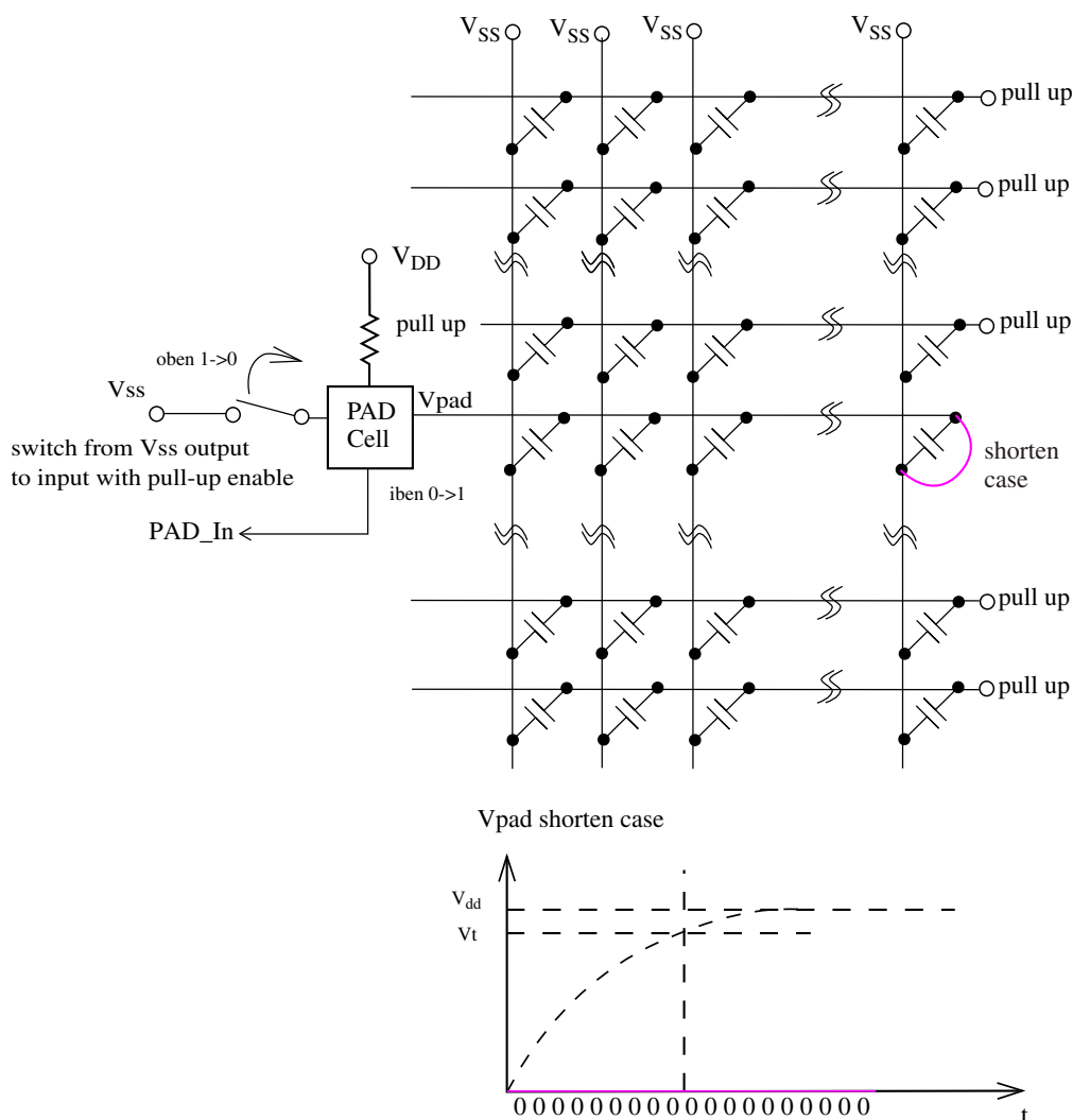
Figure 57-35. Pullup fault detect in connection/segment short case
