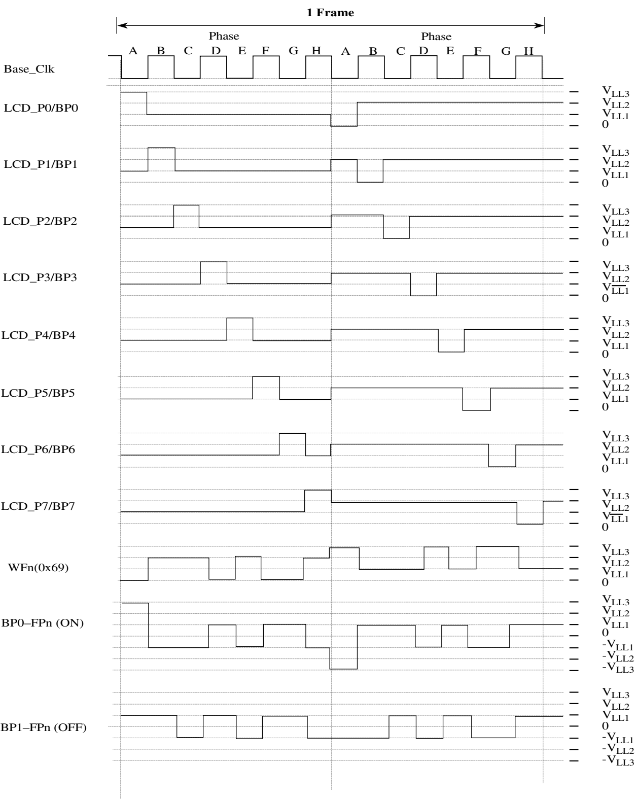
Figure 57-31. 1/8 Duty and 1/3 bias (low-power waveform)
