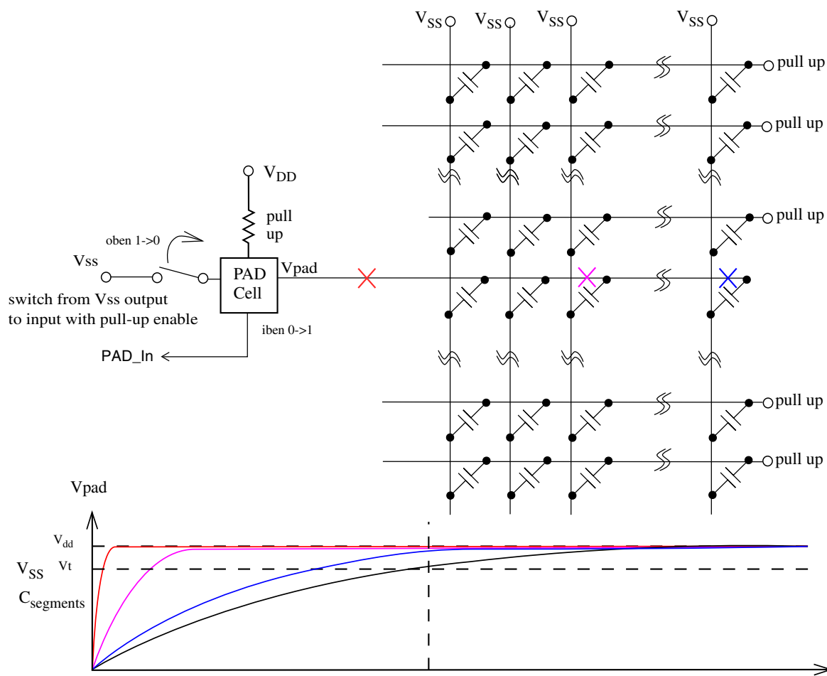
Figure 57-34. Pullup fault detect in connection/segment open case
