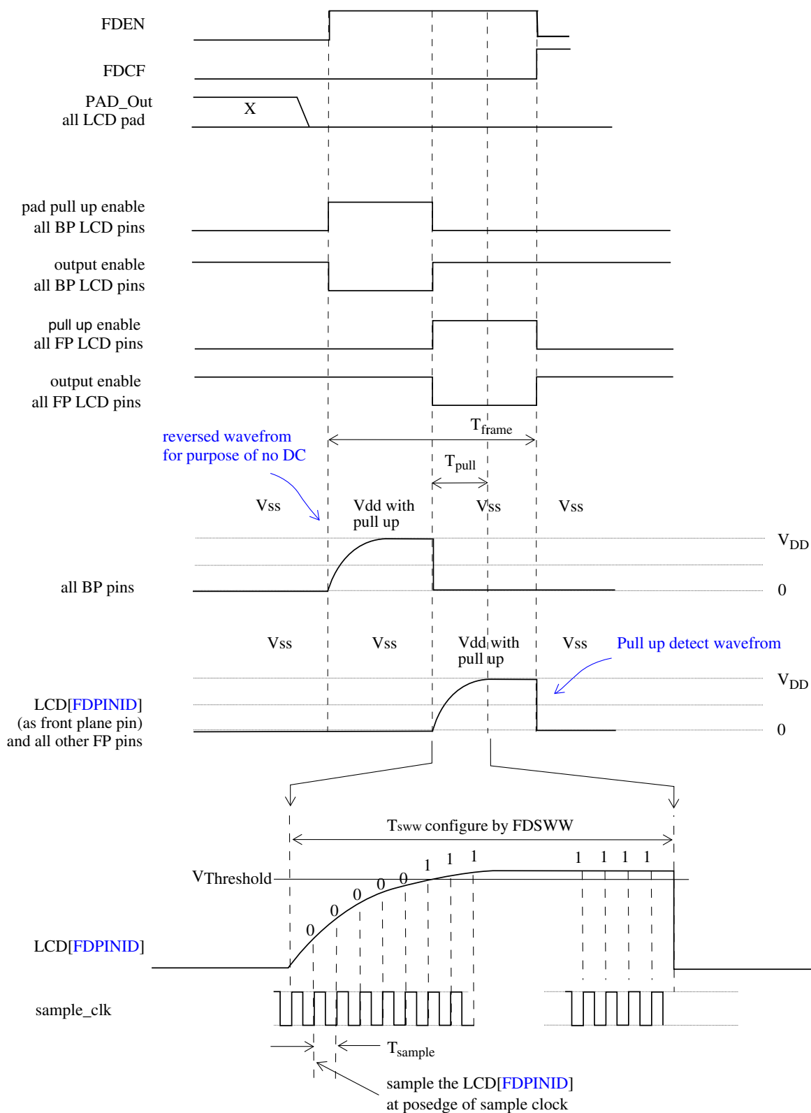
Figure 57-36. Pullup fault detection timing diagram, while FDBPEN is 0
