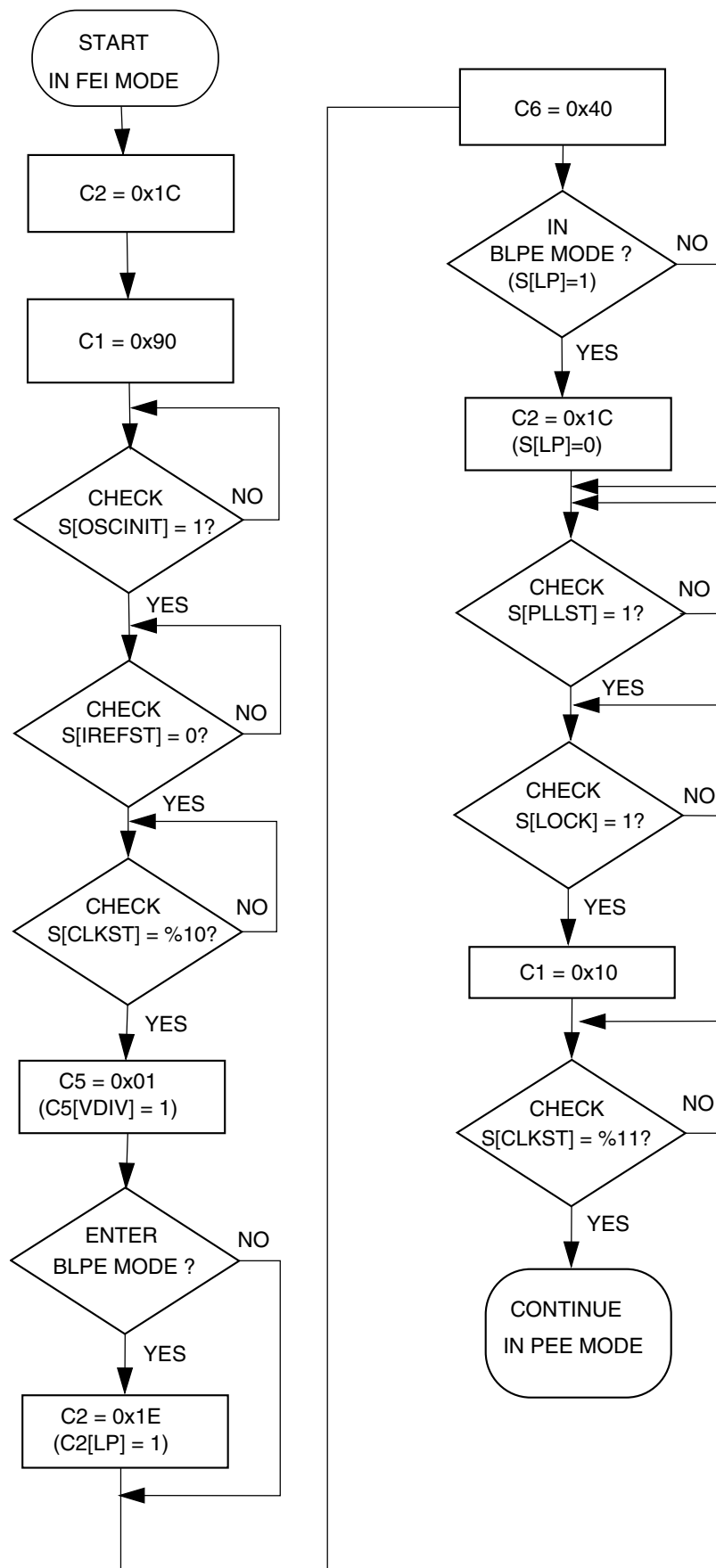
Figure 24-13. Flowchart of FEI to PEE Mode Transition using a 4 MHz crystal K53 Sub-Family Reference Manual, Rev. 6, Nov 2011
