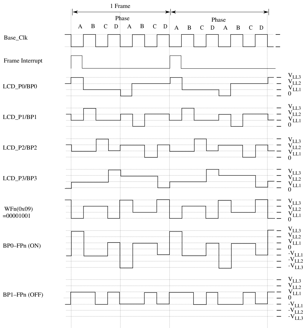
Figure 57-30. 1/4 Duty and 1/3 bias (low-power waveform)
