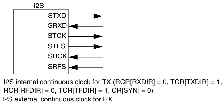
Figure 54-2. Asynchronous (SYN = 0) I 2 S configurations—continuous clock
