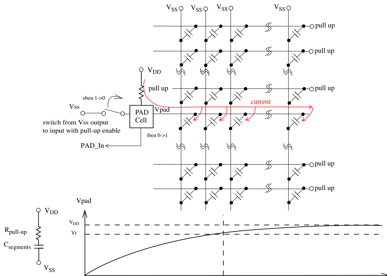
Figure 57-33. Pullup fault detect in connection/segment normal case
