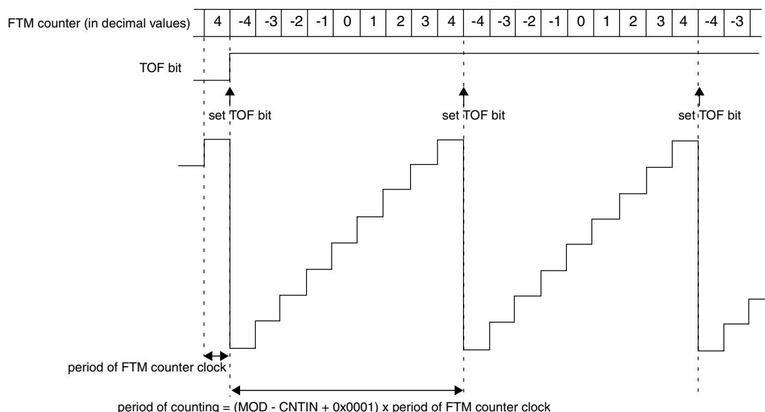
Figure 41-168. Example of FTM Up and Signed Counting
