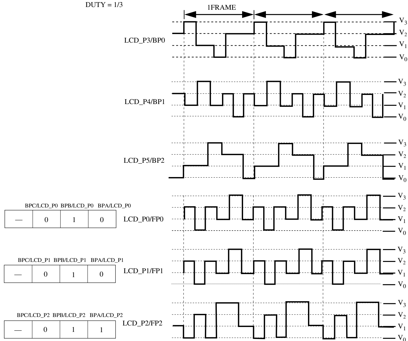
Figure 57-40. LCD waveforms
