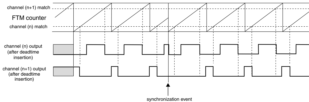
Figure 41-220. FTM Counter Synchronization
