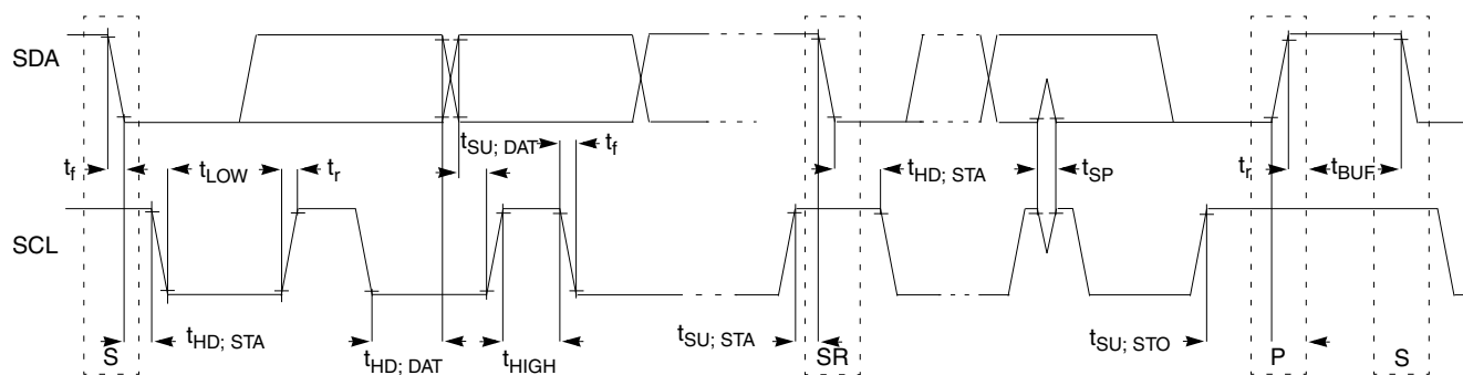
Figure 34. Timing definition for fast and standard mode devices on the I²C bus
