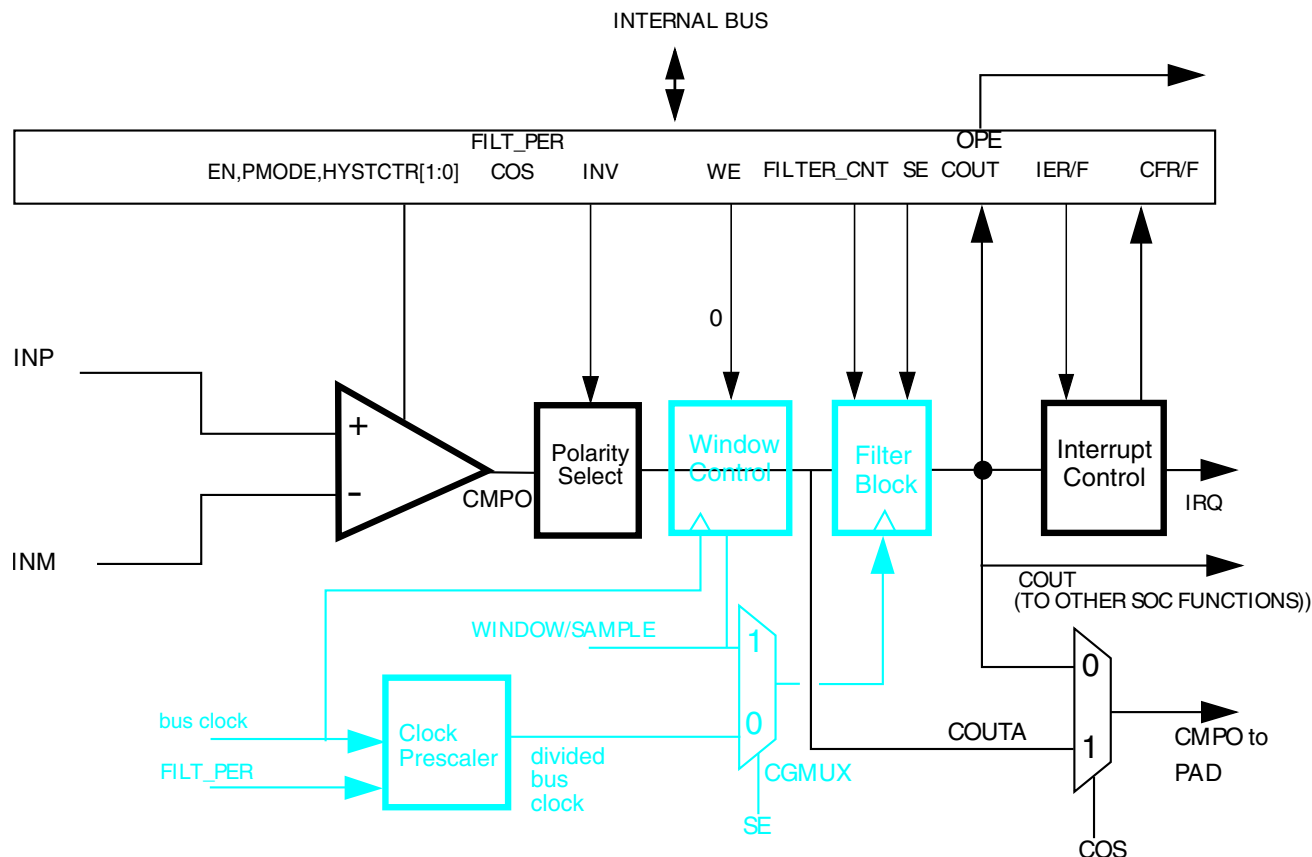
Figure 39-33. Comparator Operation in Continuous Mode
