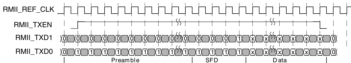
Figure 48-71. RMII transmit operation
