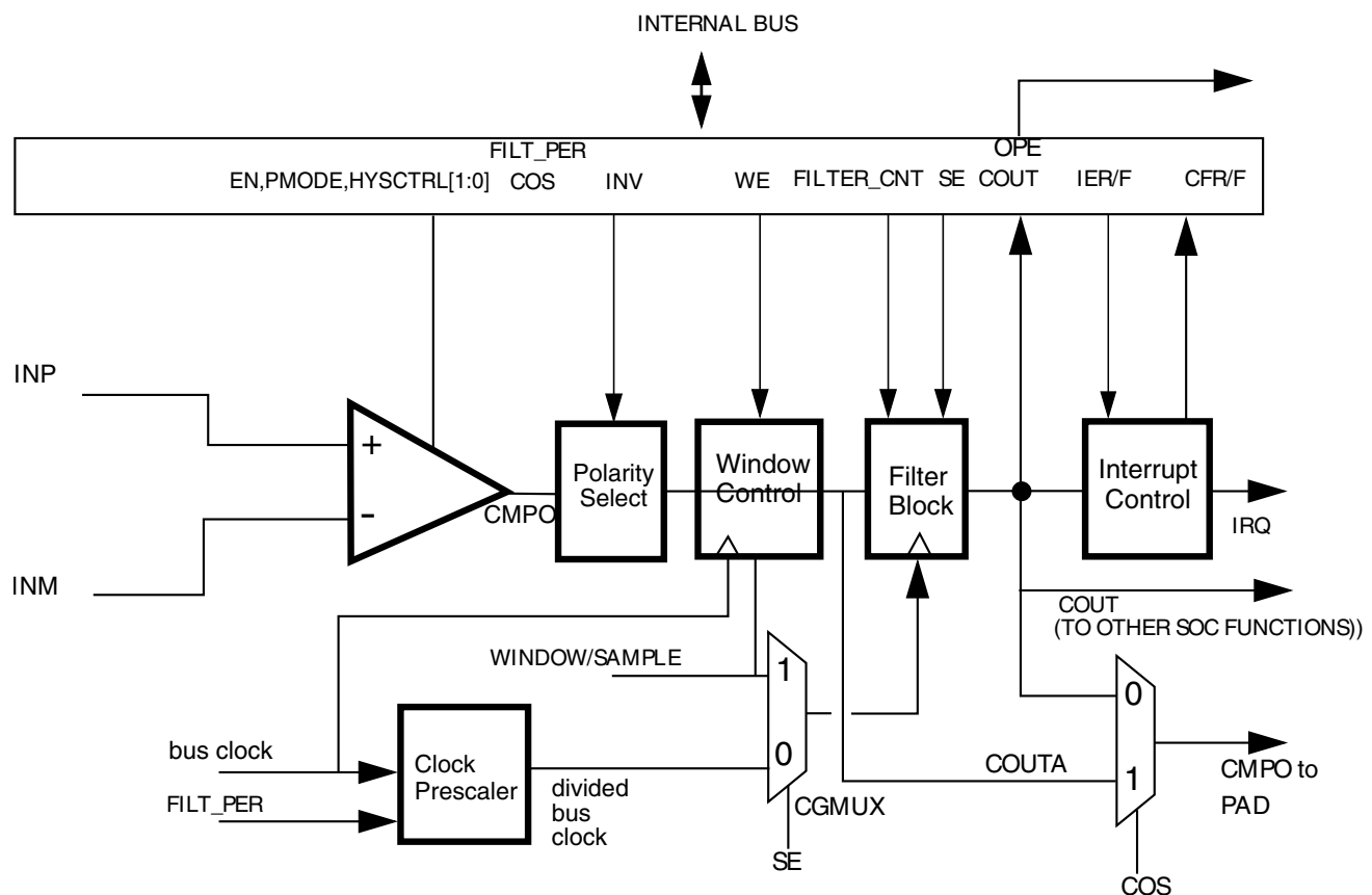
Figure 39-2. Comparator Module Block Diagram
