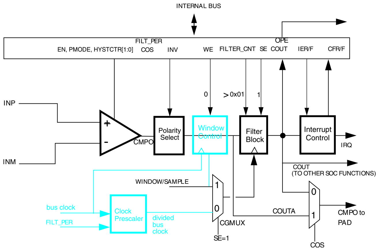
Figure 39-36. Sampled, Filtered (# 4A): Sampling point externally driven
