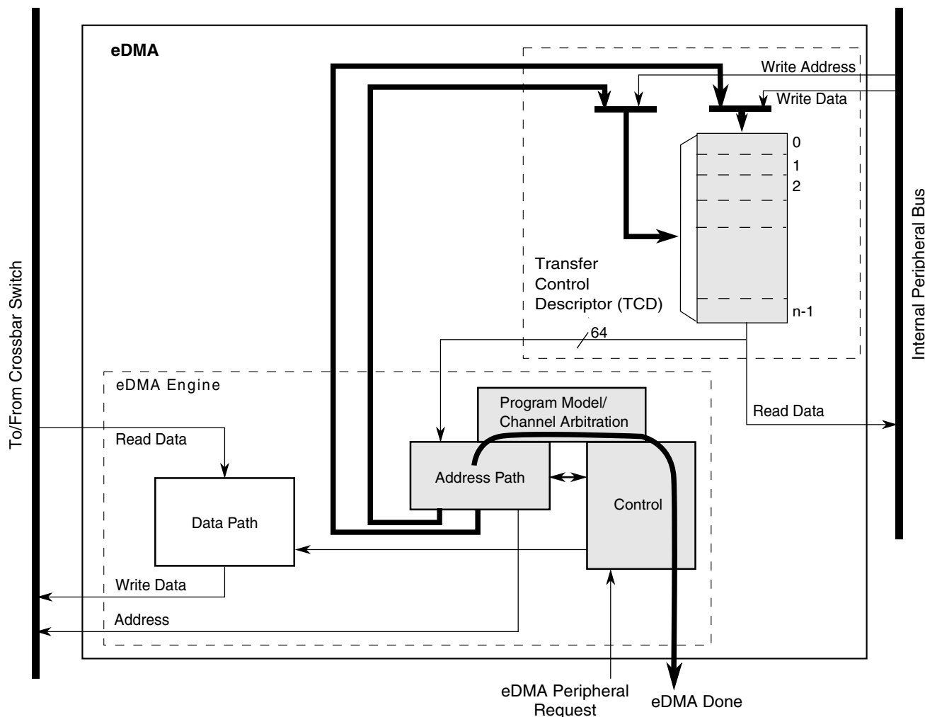
Figure 22-547. eDMA operation, part 3
