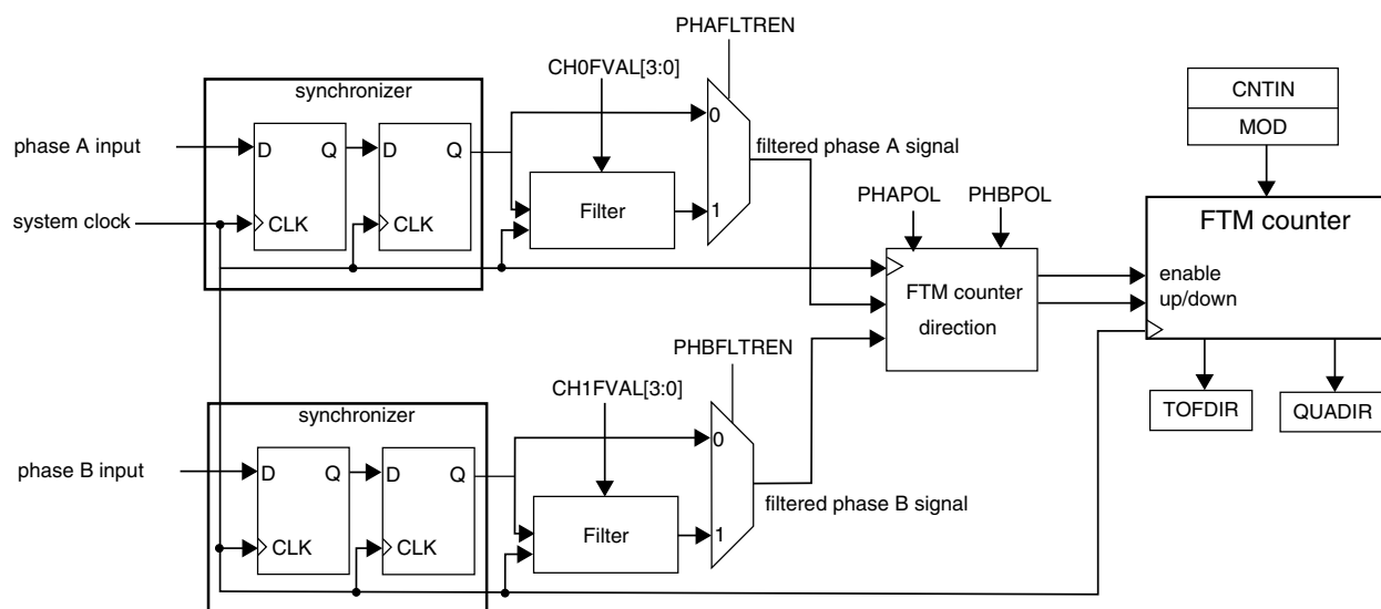
Figure 43-291. Quadrature Decoder Block Diagram
