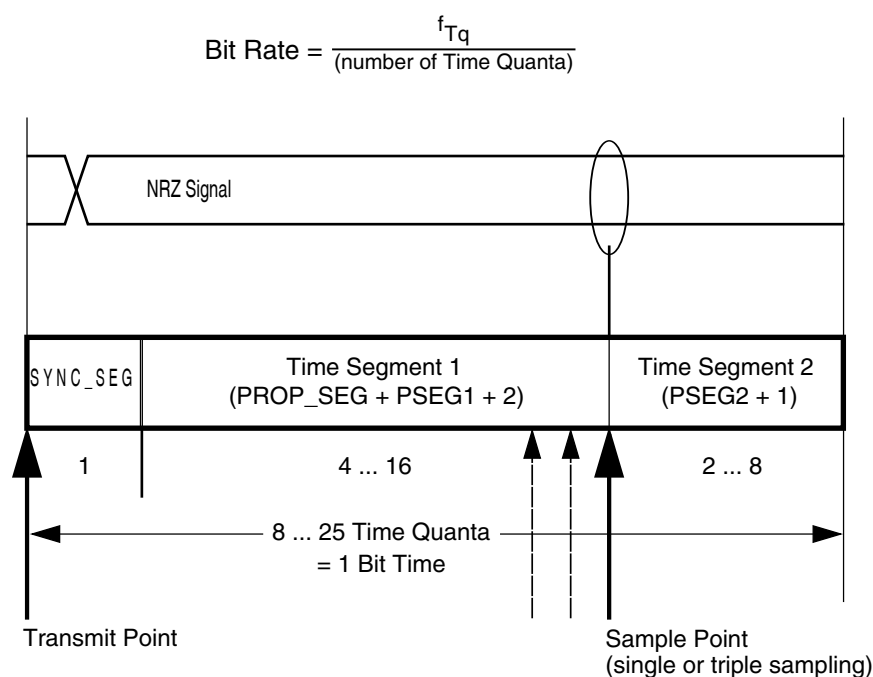
Figure 53-105. Segments within the Bit Time
