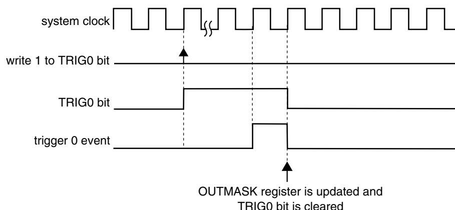
Figure 43-257. OUTMASK Synchronization with (SYNCMODE = 0), (HWTRIGMODE = 0), (SYNCHOM = 1), (PWMSYNC = 0), and (a Hardware Trigger Was Used)
