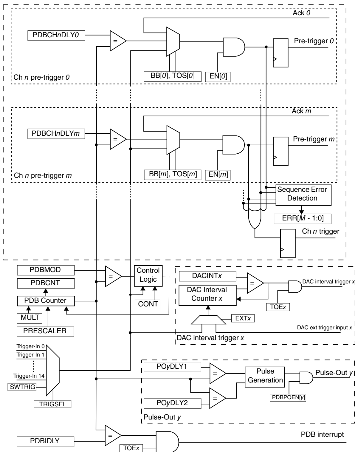
Figure 42-1. PDB Block Diagram
