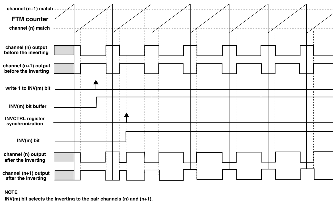
Figure 43-267. Channels (n) and (n+1) Outputs After the Inverting in Low-True (ELSnB:ELSnA = X:1) Combine Mode
