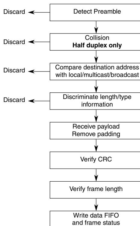
Figure 48-55. MAC Receive Flow
