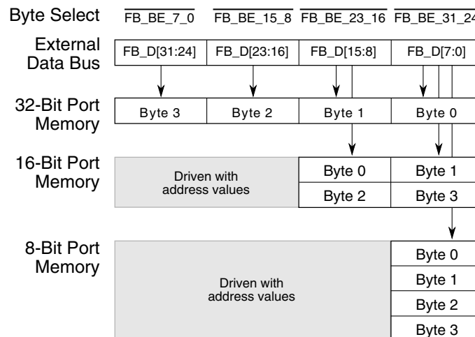
Figure 33-24. Connections for External Memory Port Sizes (CSCRn[BLS] = 1)
