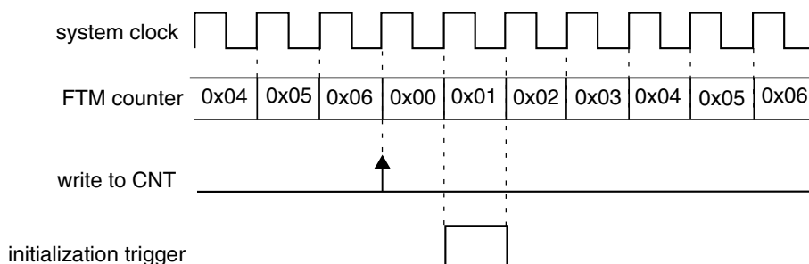
Figure 43-281. Initialization Trigger Is Generated When There Is a Write to CNT Register
