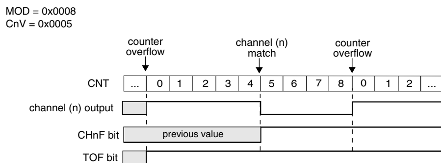
Figure 43-223. EPWM Signal with ELSnB:ELSnA = 1:0
