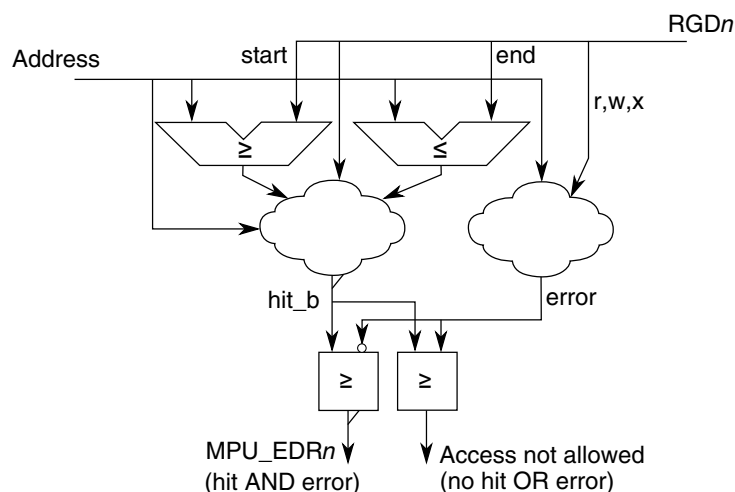
Figure 19-100. MPU Access Evaluation Macro
