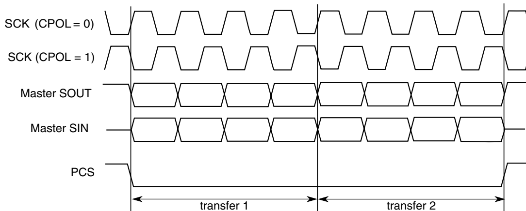
Figure 54-99. Continuous SCK Timing Diagram (CONT=1)
