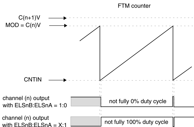
Figure 43-243. Channel (n) Output If (C(n+1)V > MOD) and (CNTIN < C(n)V = MOD)
