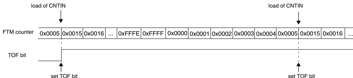
Figure 43-211. Example of Up Counting When the Value of CNTIN Is Greater Than the Value of MOD
