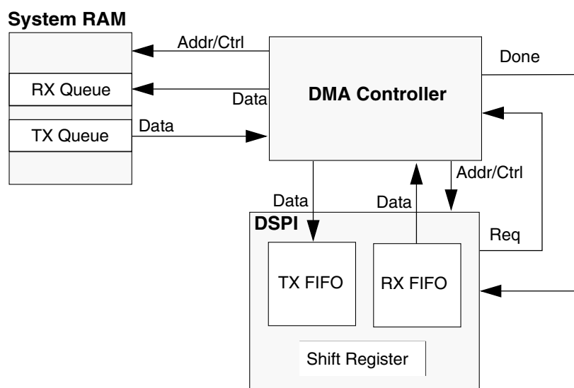
Figure 54-2. DSPI with Queues and DMA
