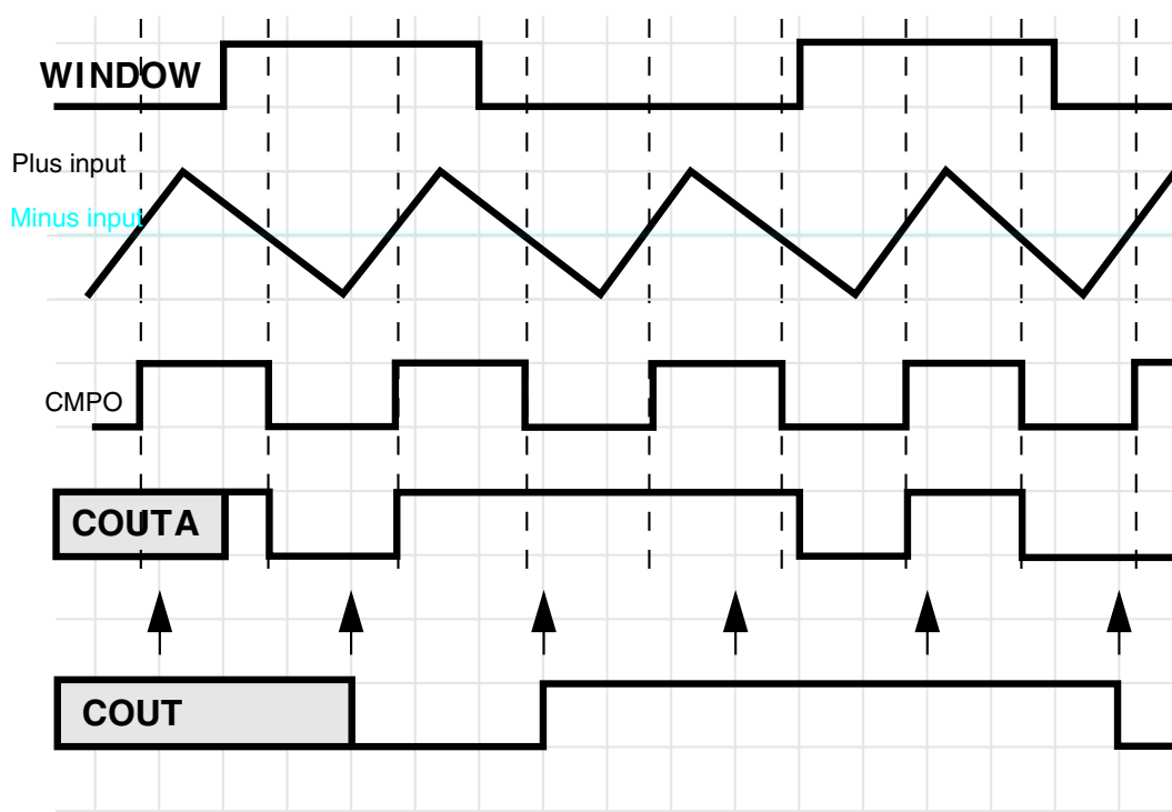
Figure 39-40. Windowed / Resampled Mode Operation
