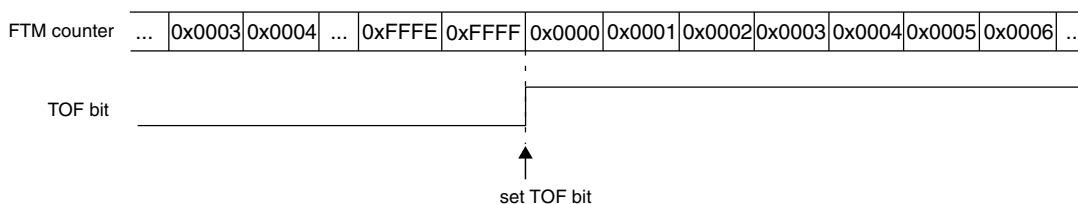
Figure 43-213. Example When the FTM Counter Is a Free Running
