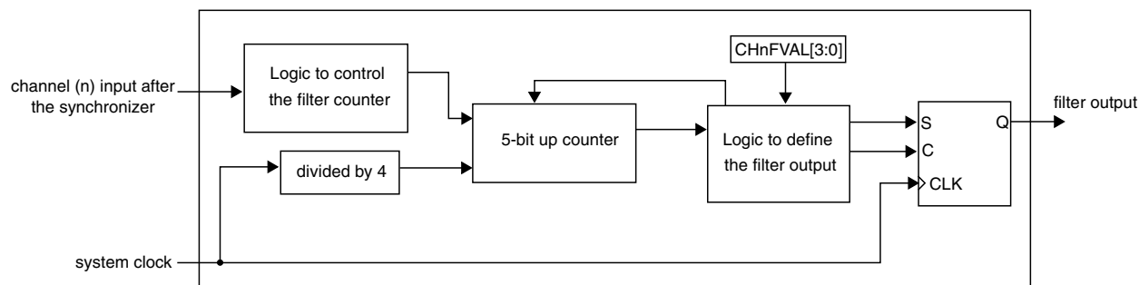
Figure 43-217. Channel Input Filter
