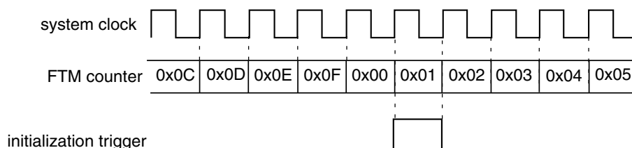
Figure 43-280. Initialization Trigger Is Generated When the FTM Counting Achieves the CNTIN Register Value
