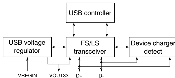
Figure 3-58. USB Subsystem Overview
