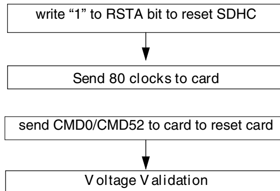
Figure 57-40. Flow chart for reset of the SDHC and SD I/O card
