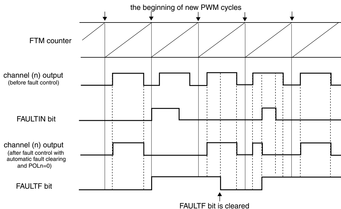
Figure 43-276. Fault Control with Automatic Fault Clearing
