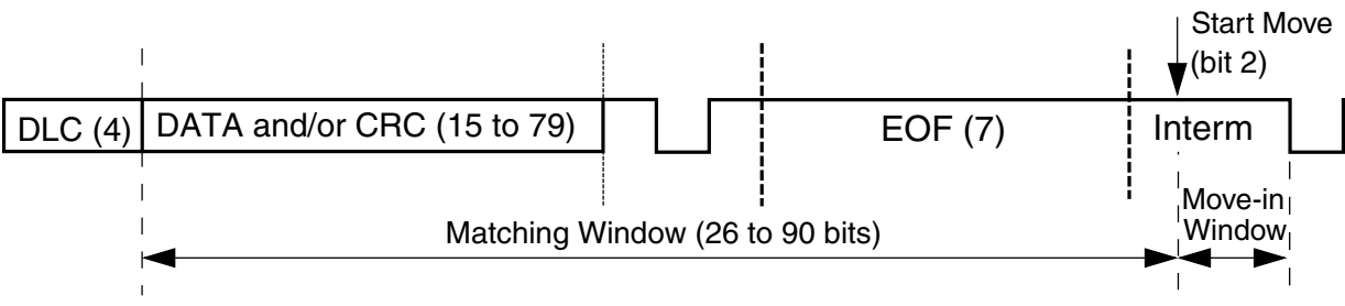
Figure 53-106. Matching and Move-In Time Windows
