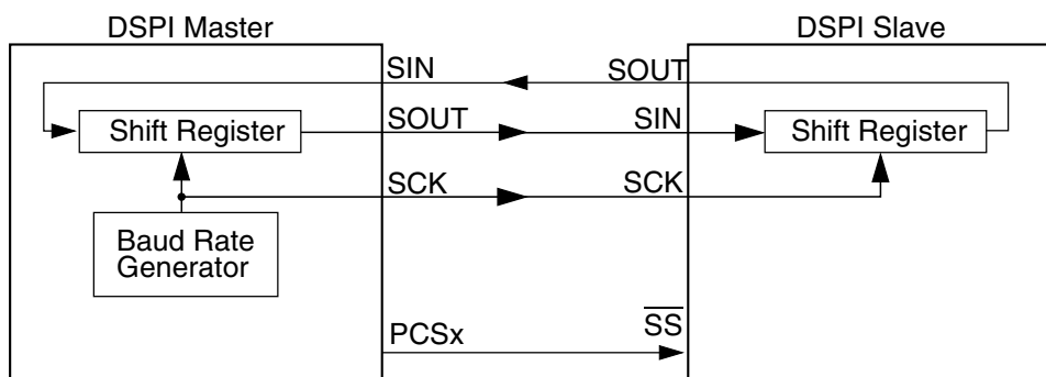
Figure 54-91. SPI Serial Protocol Overview
