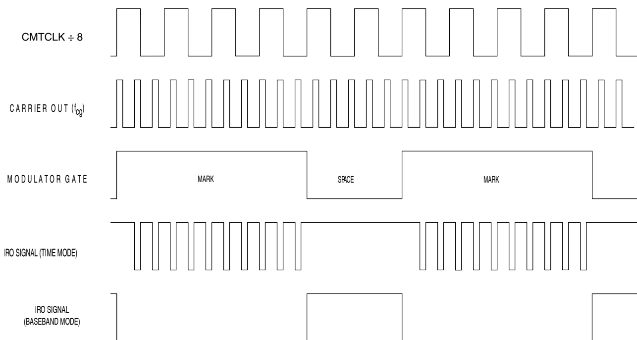
Figure 46-17. Example: CMT Output in Time and Baseband Modes with OC[CMTPOL]=0
