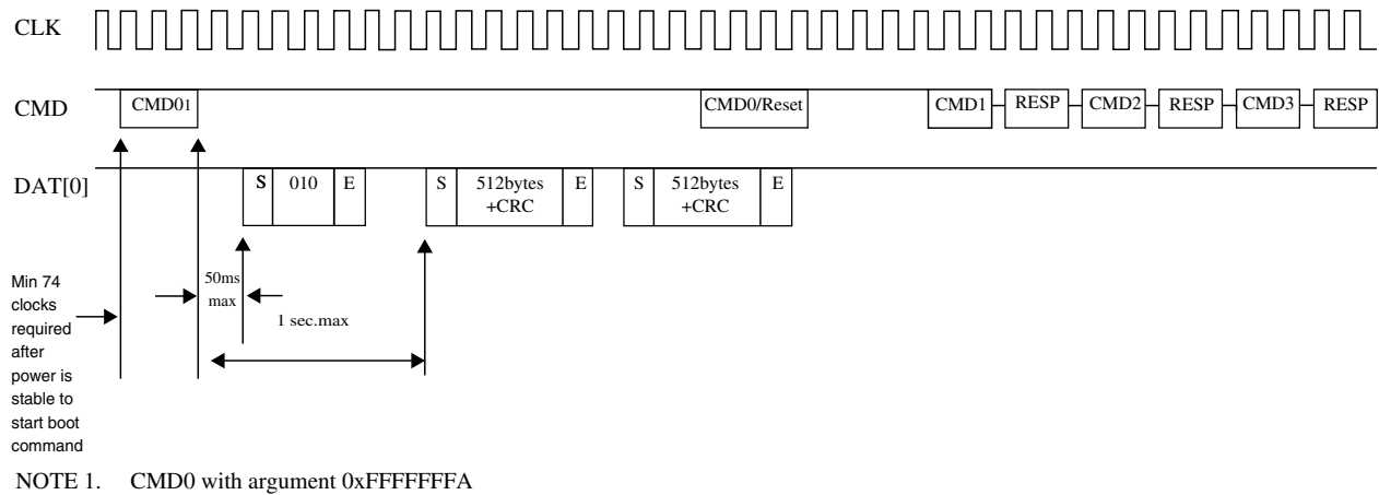
Figure 57-38. MultiMediaCard state diagram (alternative boot mode)
