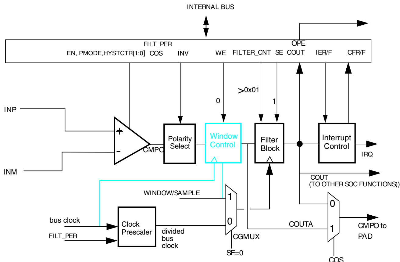
Figure 39-37. Sampled, Filtered (# 4B): Sampling point internally derived
