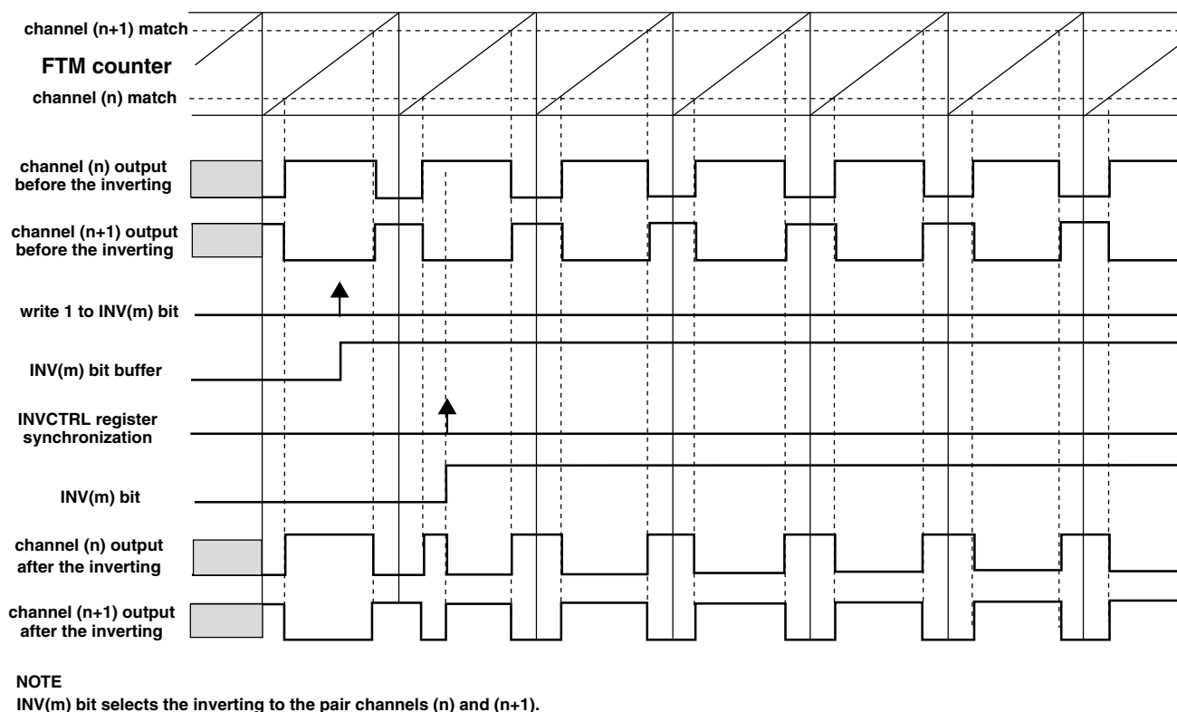
Figure 43-266. Channels (n) and (n+1) Outputs After the Inverting in High-True (ELSnB:ELSnA = 1:0) Combine Mode
