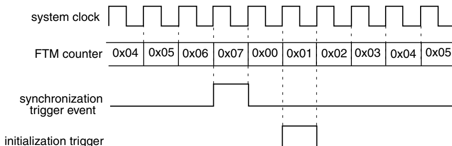
Figure 43-282. Initialization Trigger Is Generated When There Is the FTM Counter Synchronization
