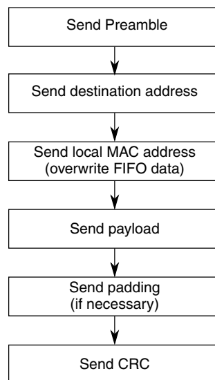
Figure 48-56. Frame Transmit Overview
