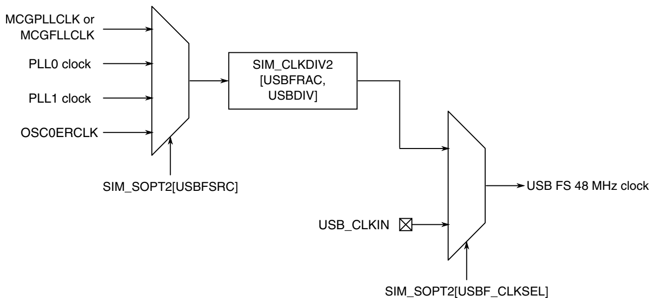
Figure 5-8. USB FS clock generation
