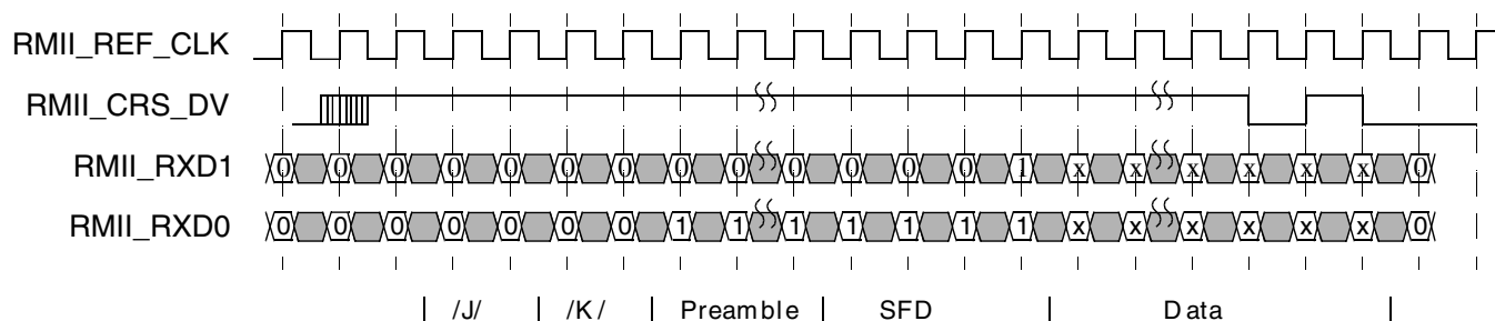
Figure 48-69. RMII receive operation
