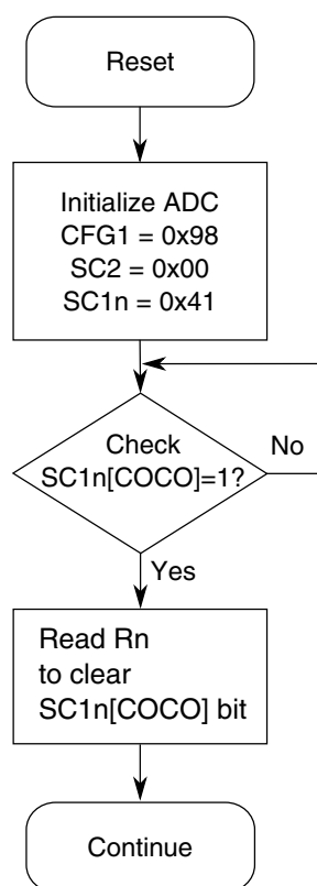
Figure 38-159. Initialization Flowchart for Example
