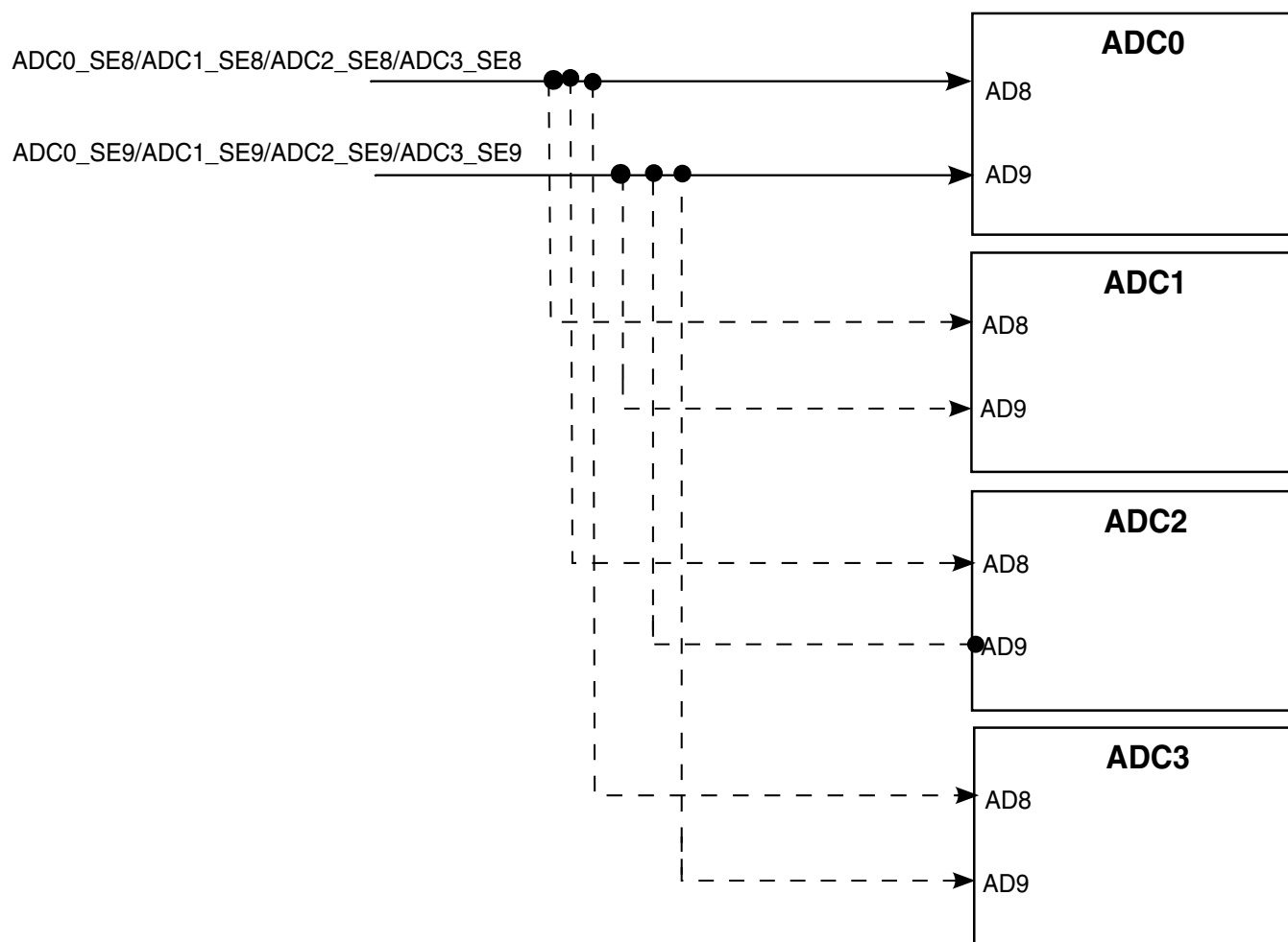
Figure 3-41. ADC hardware interleaved channels integration
