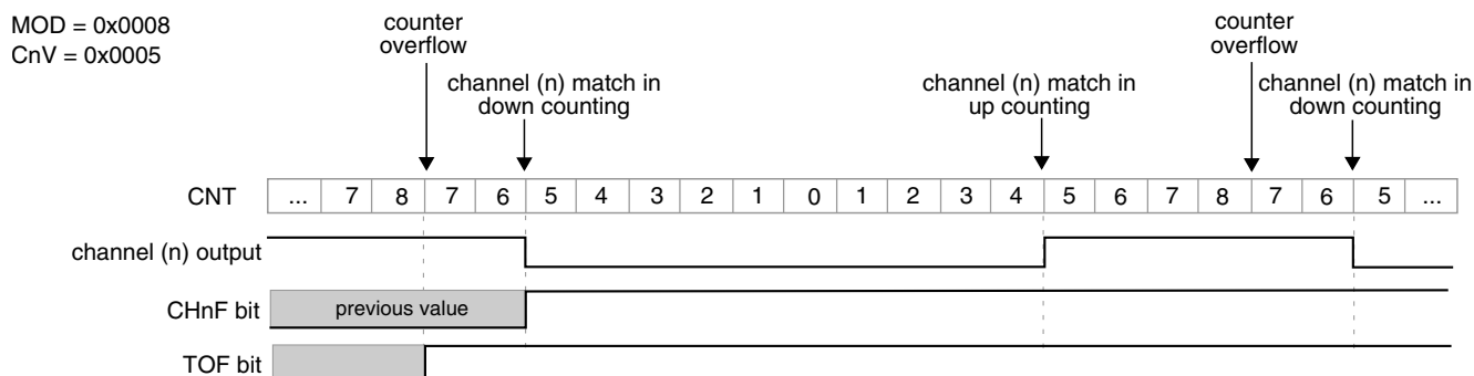
Figure 43-227. CPWM Signal with ELSnB:ELSnA = X:1
