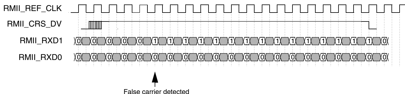
Figure 48-70. RMII receive operation with false carrier
