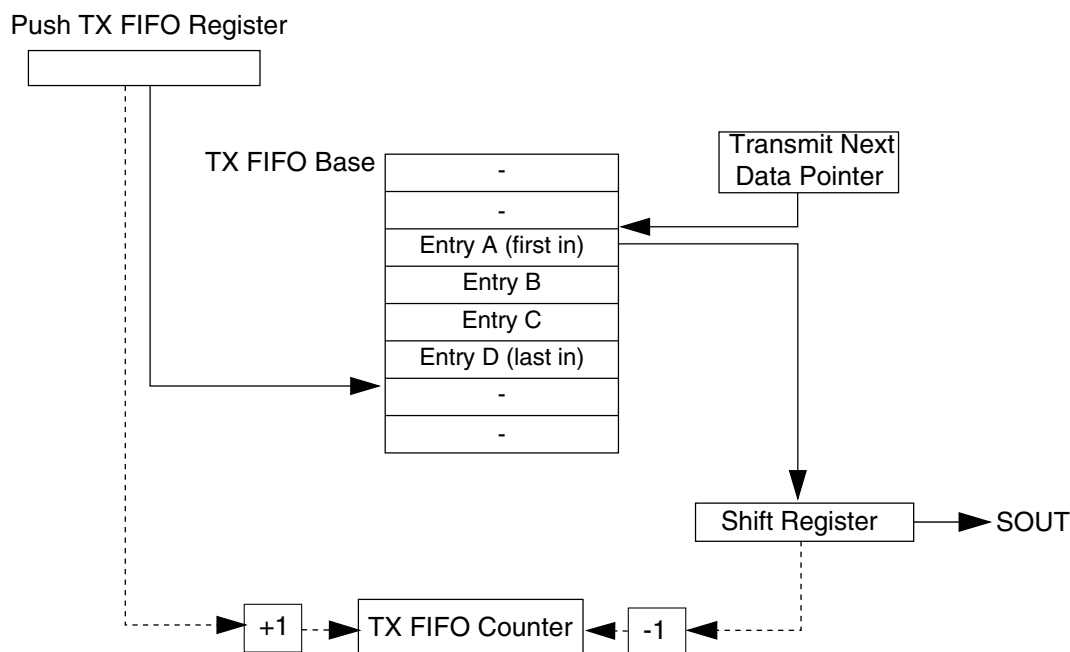
Figure 54-100. TX FIFO Pointers and Counter
