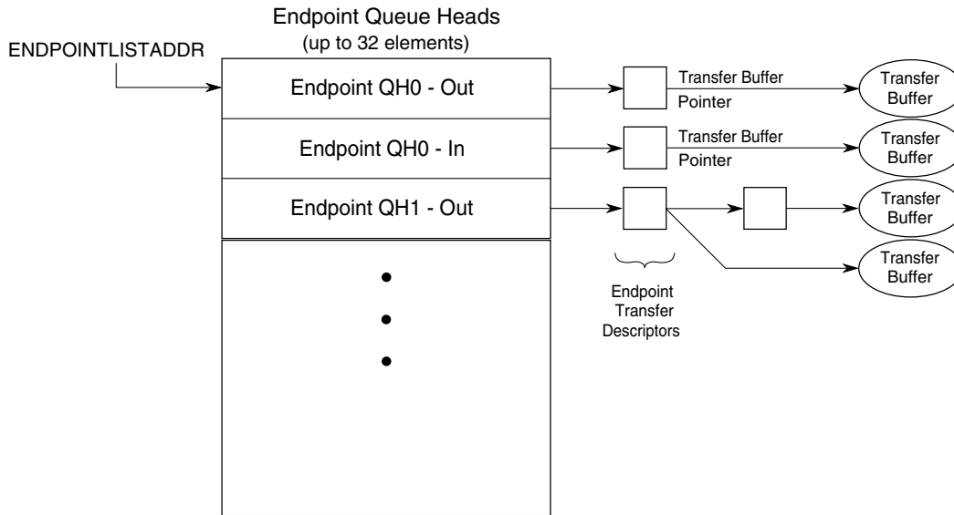
Figure 52-50. Endpoint Queue Head Diagram
