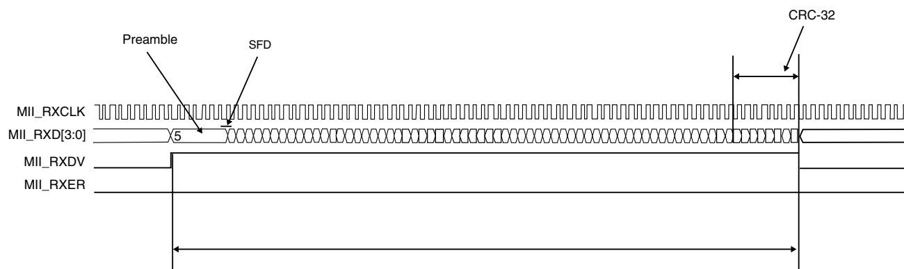
Figure 48-75. MII Receive Operation
