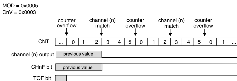
Figure 43-220. Example of the Output Compare Mode when the Match Clears the Channel Output
