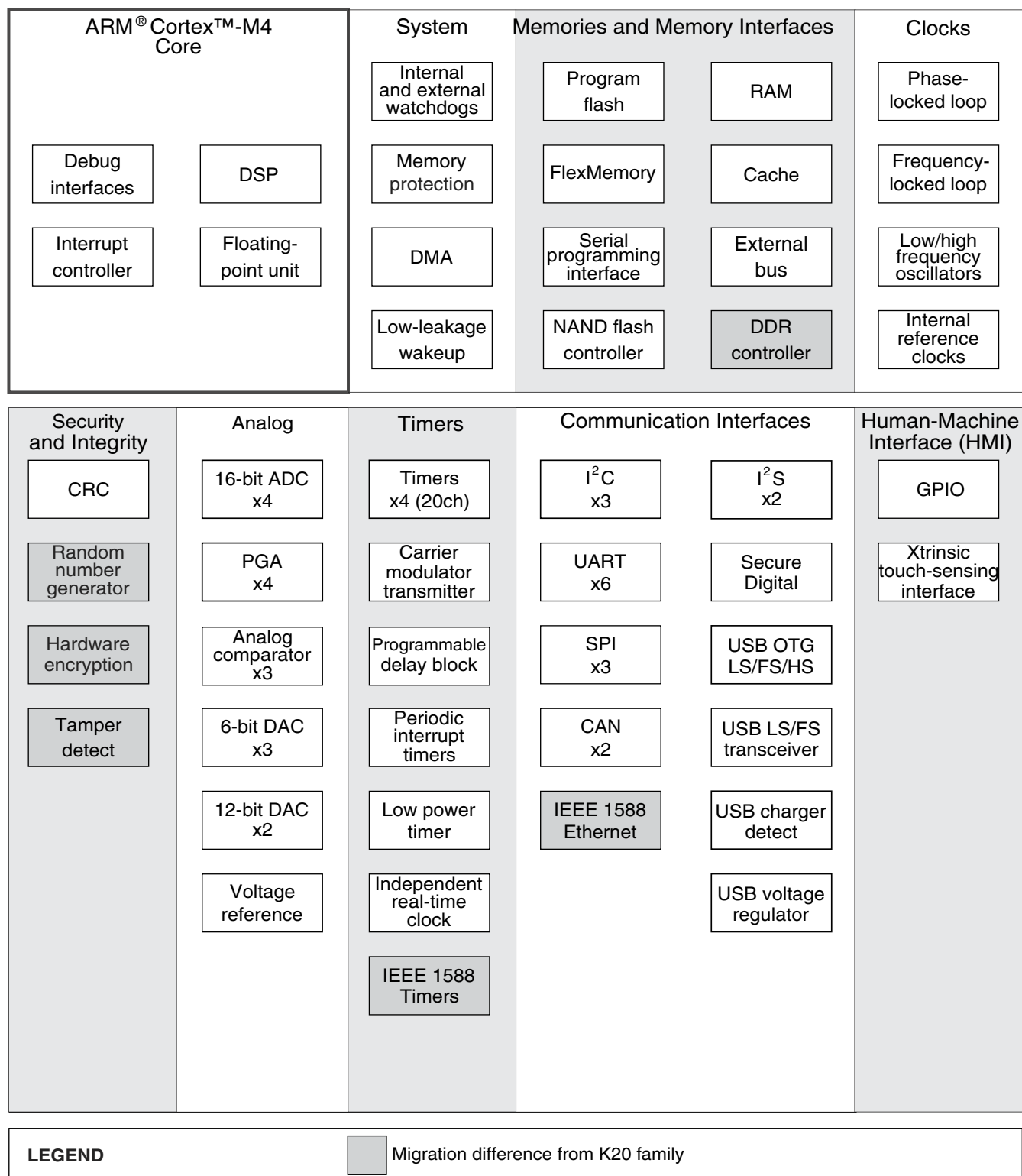
Figure 2. K61 Block Diagram
