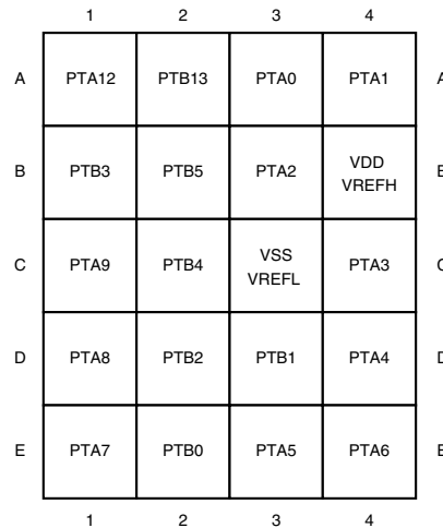
Figure 10-2. KL02 20-pin WLCSP pinout diagram
