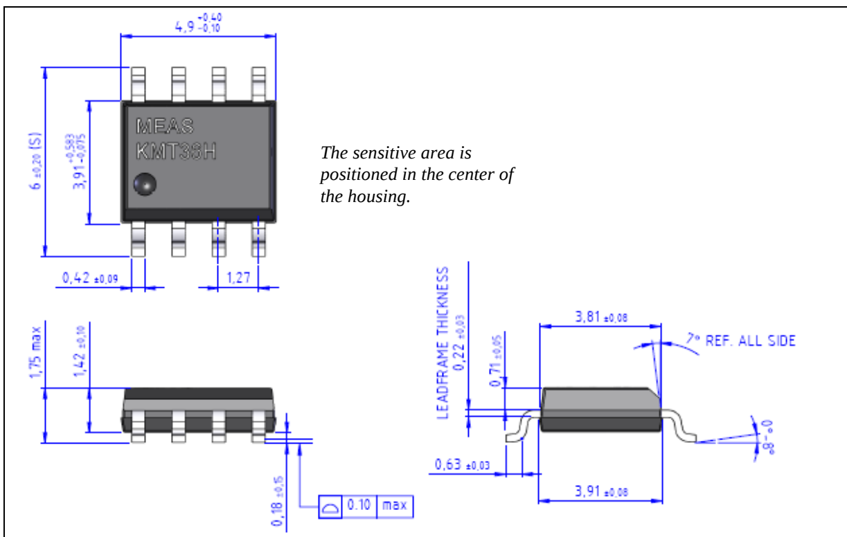
Figure 2: SO8 outline
