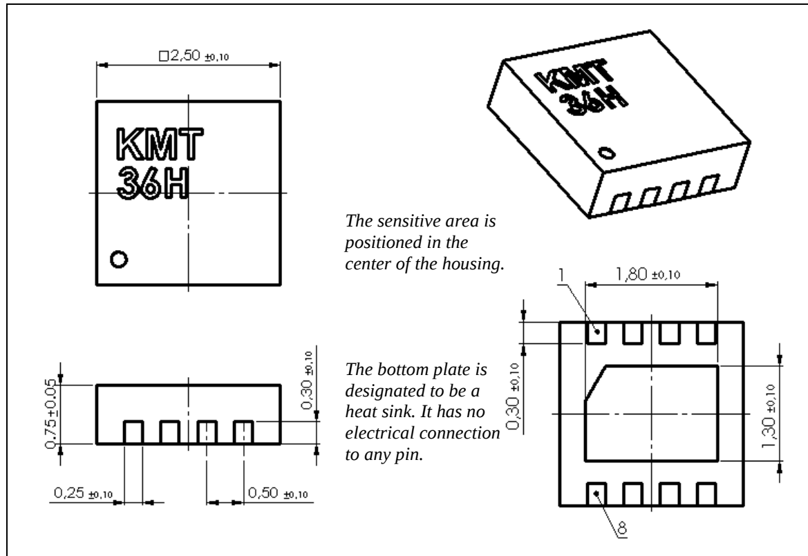
Figure 3: TDFN outline
