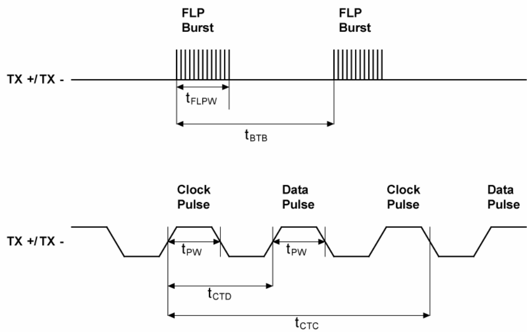
Figure 30. Auto-Negotiation Timing
