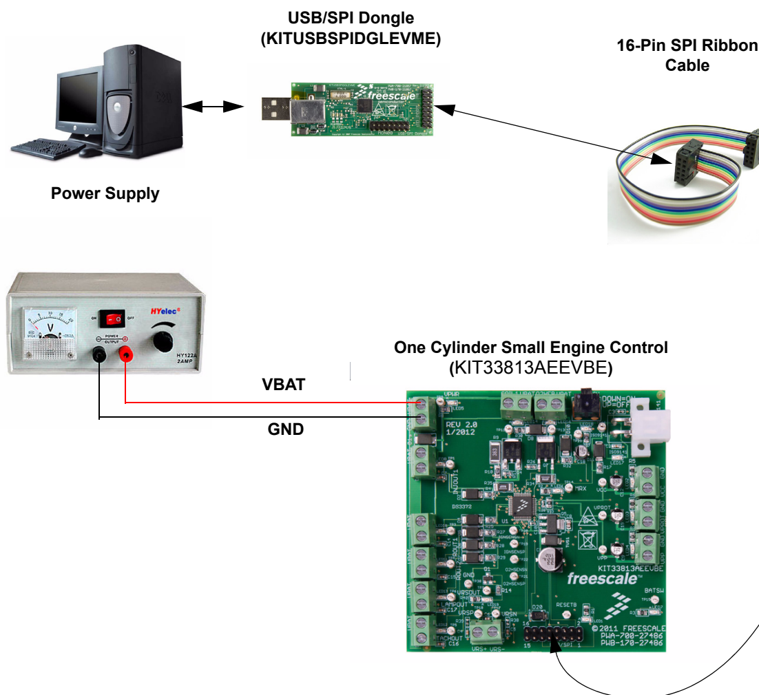
Figure 2. KIT33813AEEVBE plus KITUSBSPIDGLEVME Board Setup
