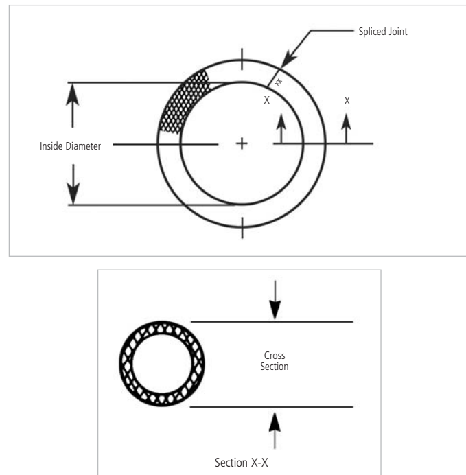
FIGURE 1. O-RING CONSTRUCTION
