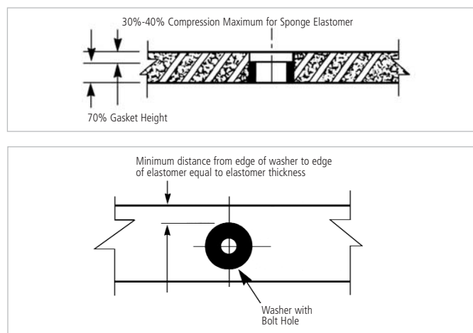
FIGURE 3B. WASHER TYPE COMPRESSION STOP
