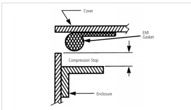
FIGURE 5B. COMPRESSION STOP BUILT INTO ENCLOSURE
