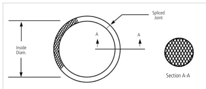
FIGURE 2. O-RING CONSTRUCTION
