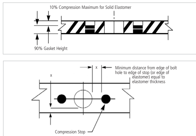
FIGURE 3A. DISC TYPE COMPRESSION STOP
