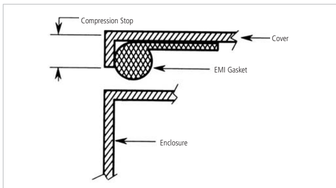
FIGURE 5A. COVER WITH COMPRESSION STOP
