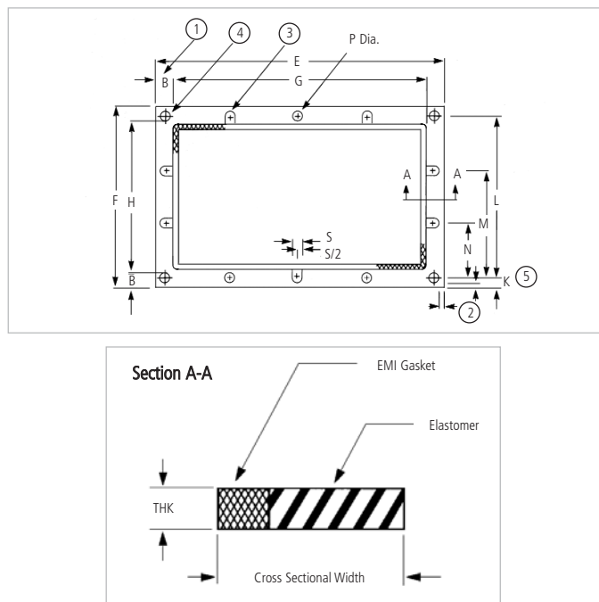
FIGURE 2. ENVIRO-SEAL GASKET
