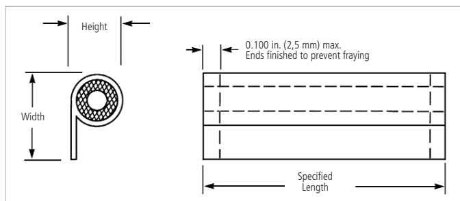
FIGURE 2. CUT-TO-LENGTH
