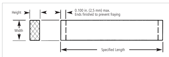
FIGURE 3. CUT-TO-LENGTH RECTANGULAR
