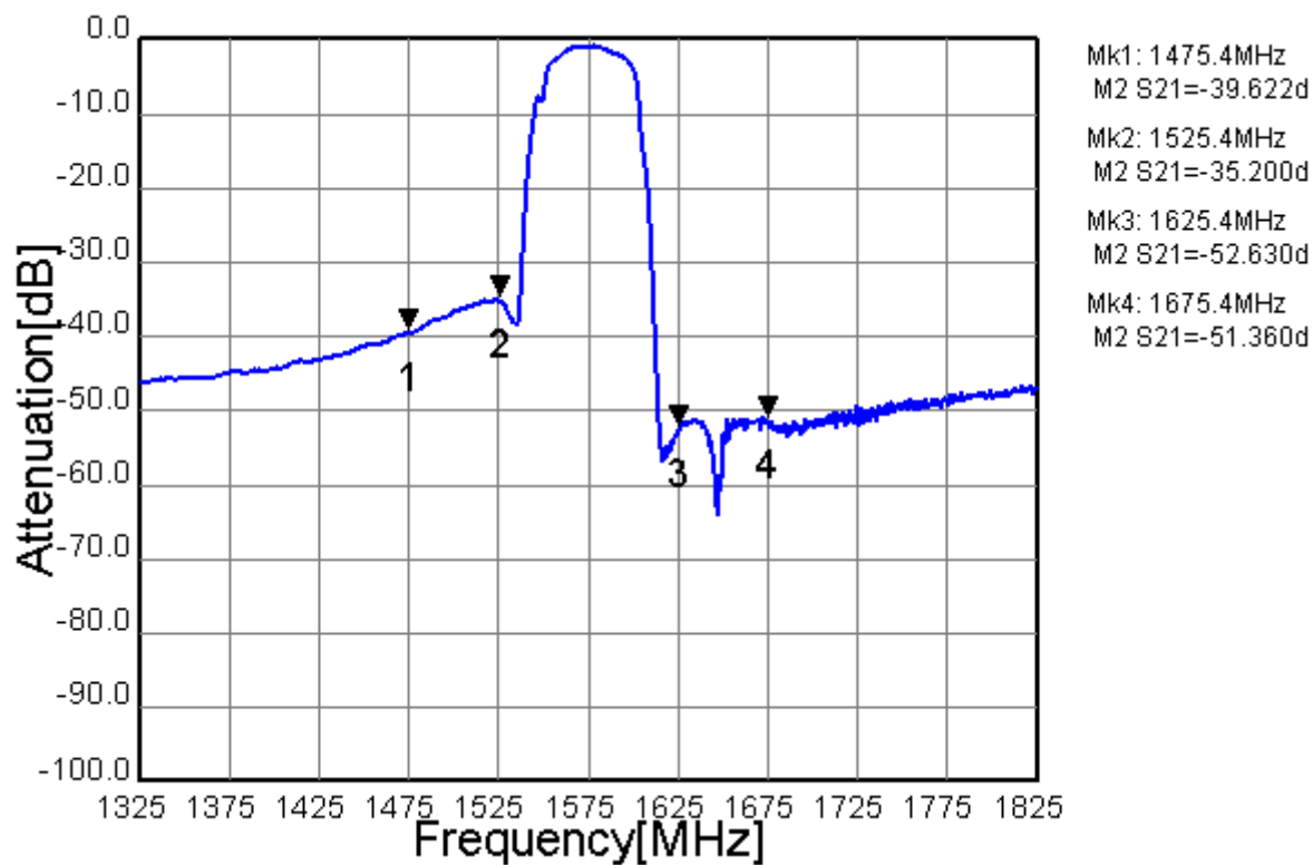
Fig.1 Pass-band Characteristics
